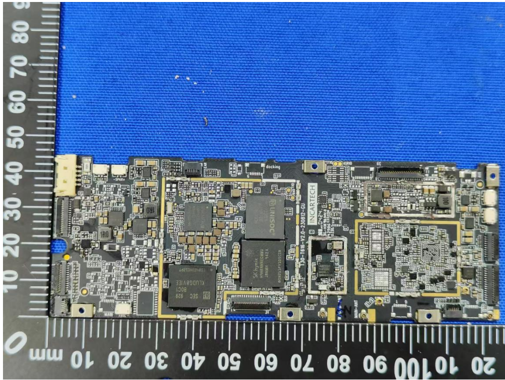
Figure 9. PCB Motherboard view of unit
