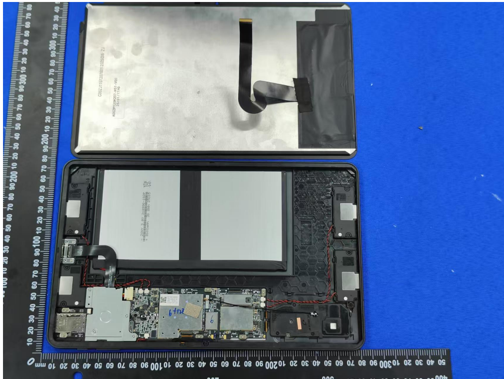
Figure 1. Internal view of unit
