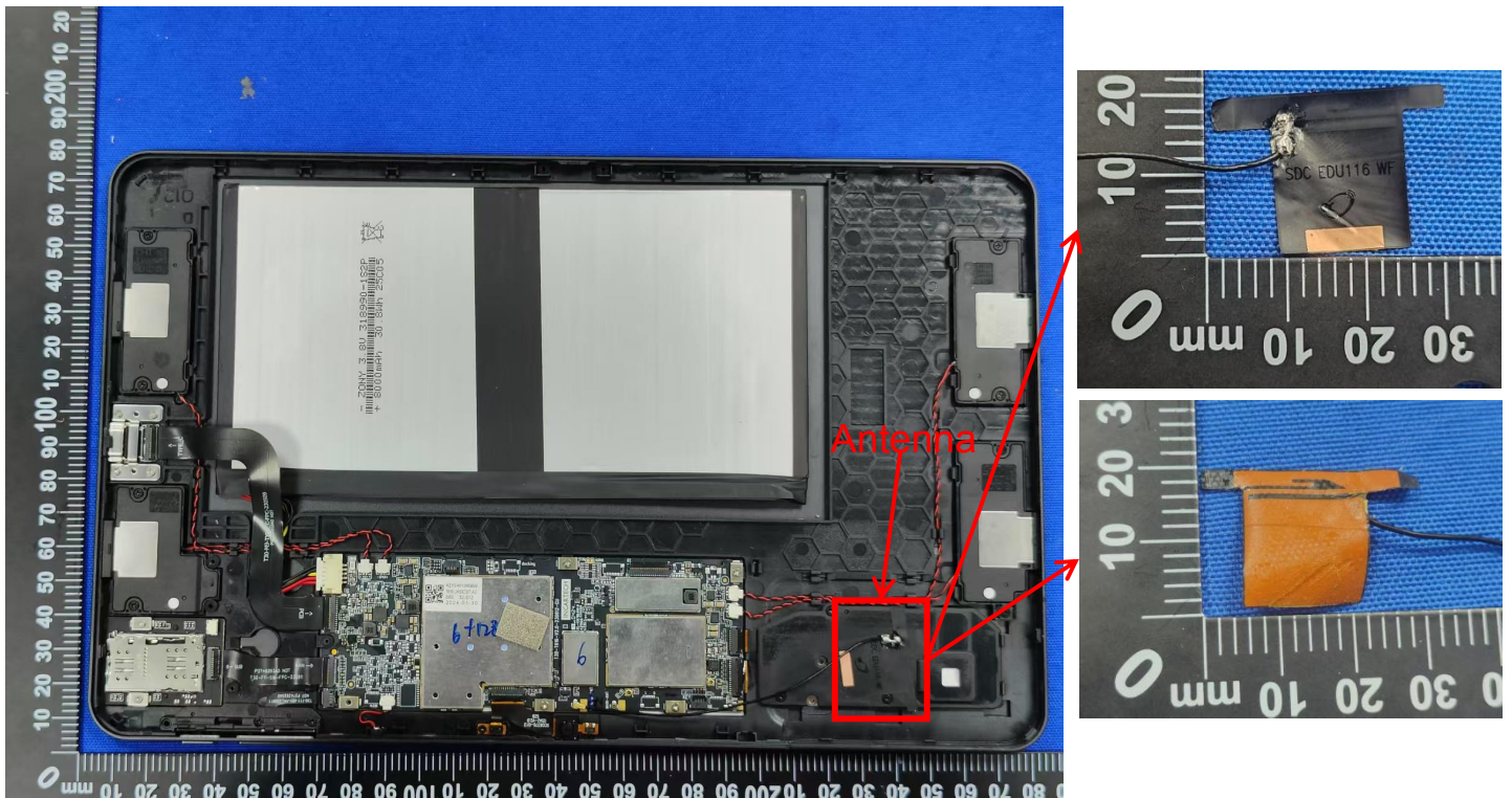
Figure 3. Internal view of unit
