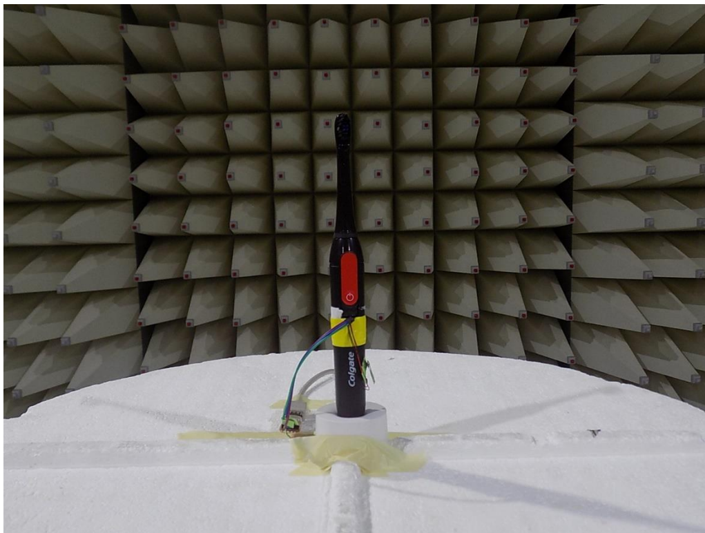
Figure 8: EUT (Z-Axis)
