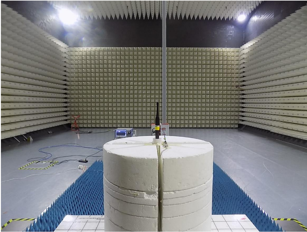
Figure 5: Test Setup for Radiated Emissions 1GHz to 18GHz
