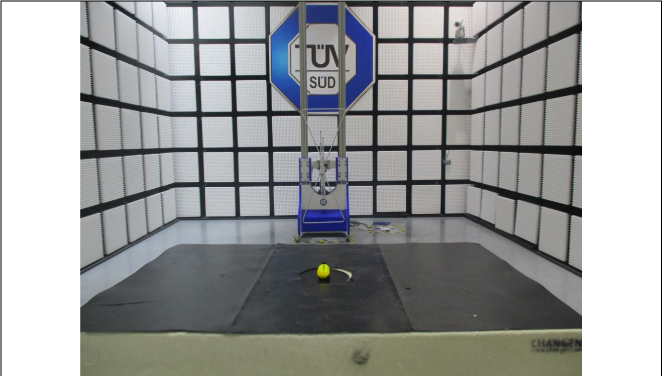
Radiated Emission test below 1GHz
