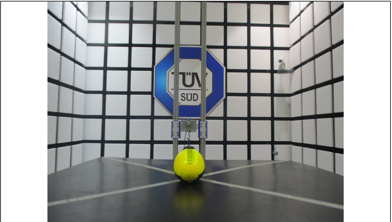
Radiated Emission test above 1GHz
