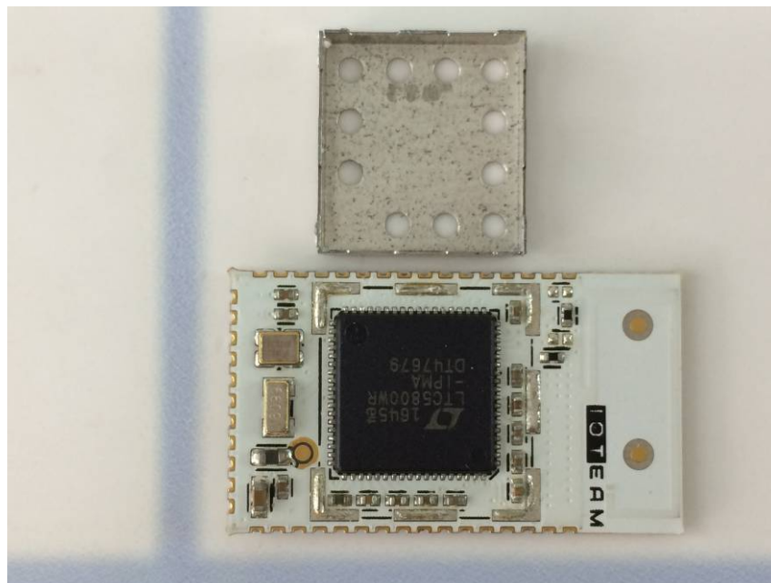
PCB Antenna Type Internal view
