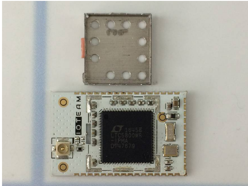
External Antenna Type Internal view
