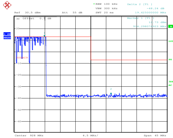
Figure 8.4-1: Conducted spurious emissions
