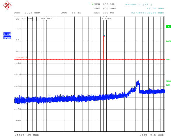
Figure 8.7-1: Conducted spurious emissions, low channel
