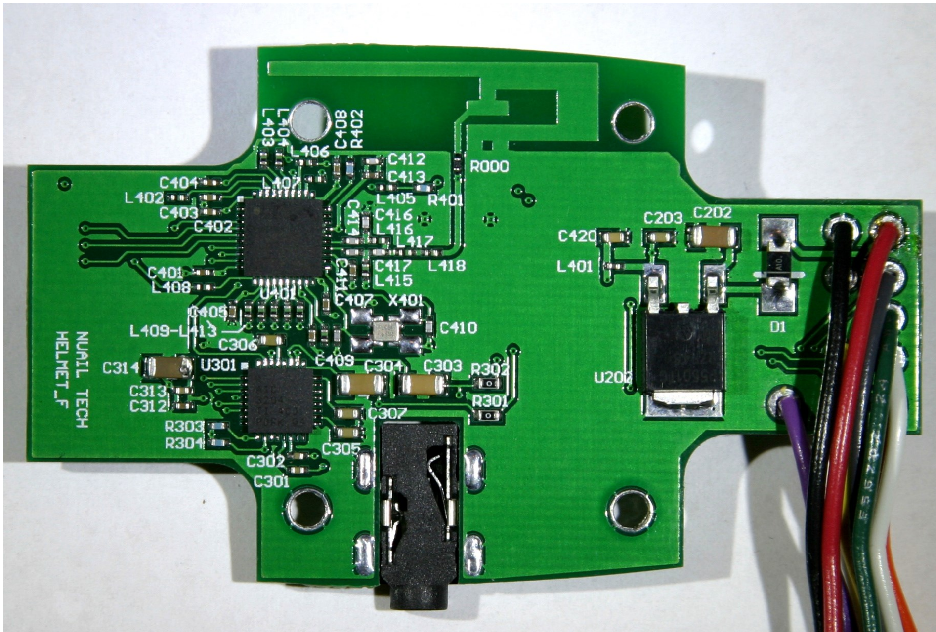
Helmet Headset - Bottom
