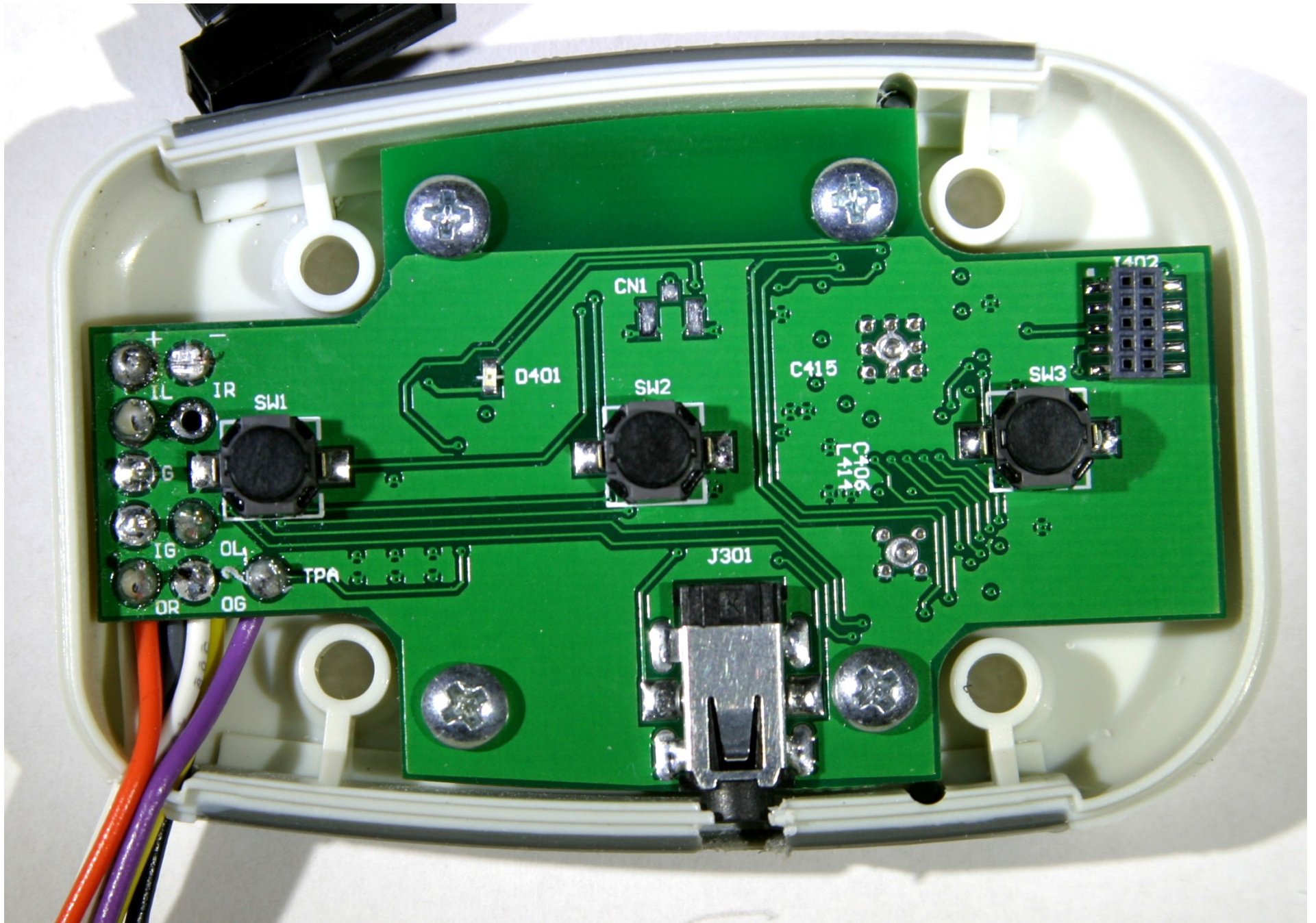
Helmet Headset - Full assembly installed in case
