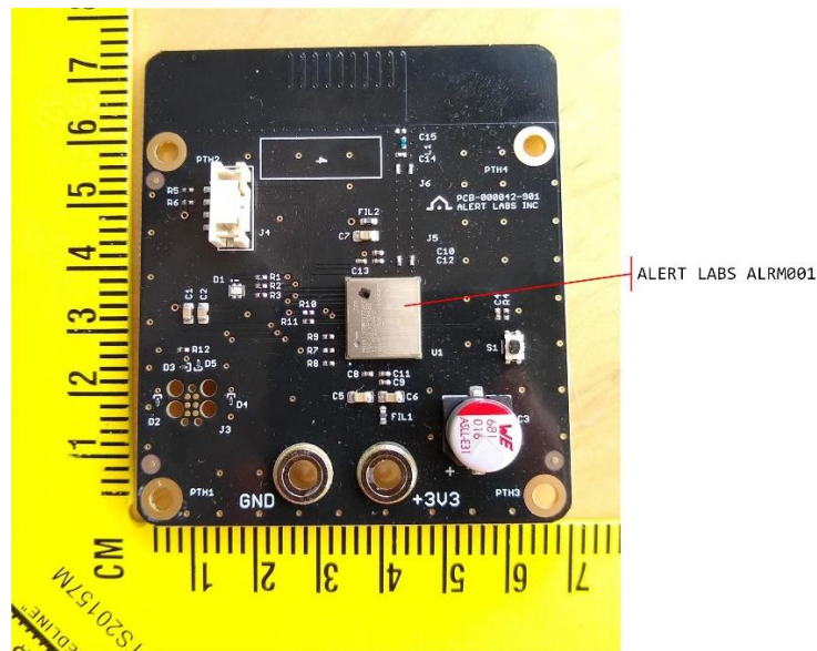
Figure 1: ALRM001 embedded on test PCB
