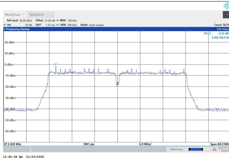
11N40SISO_Ant1_2422_30~1000
