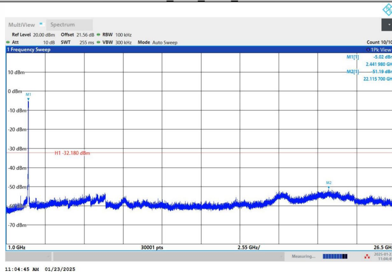
11AX40SISO_Ant1_2452_0~Reference
