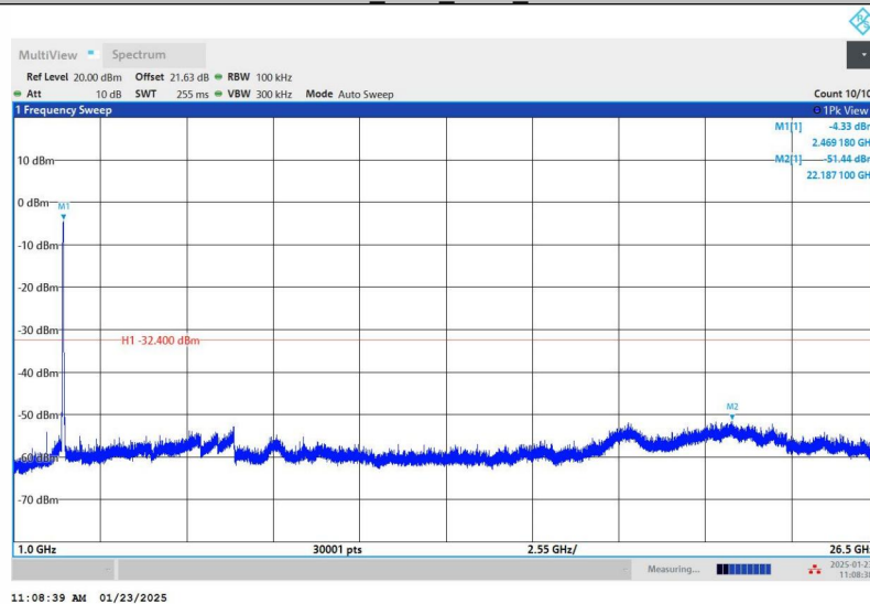
11AX40SISO_Ant1_2452_1000~26500
