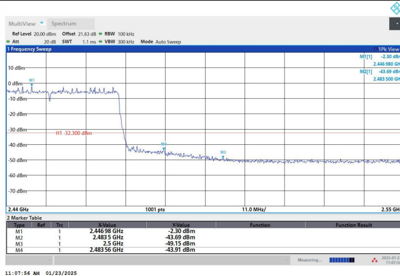
11AX40SISO_Ant1_High_2452
