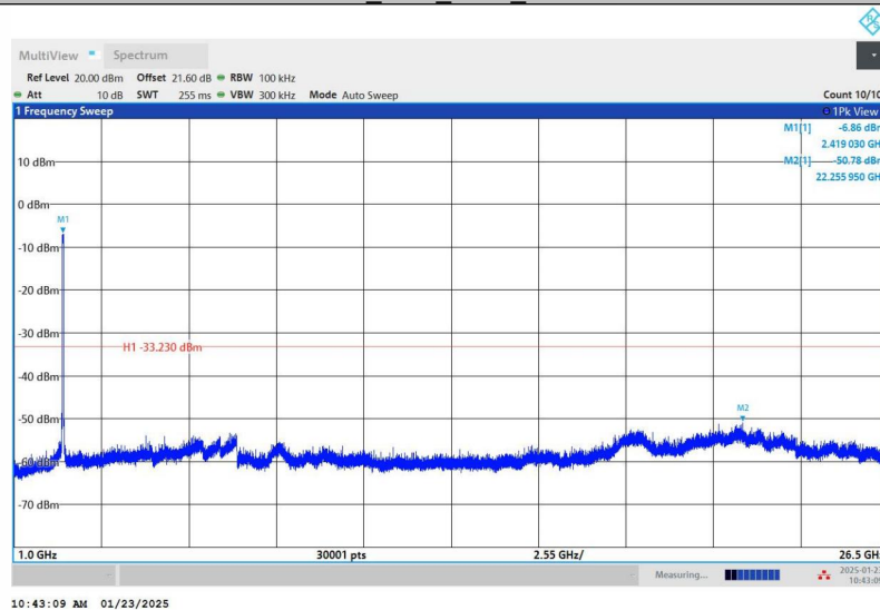
11N40SISO_Ant1_2437_0~Reference
