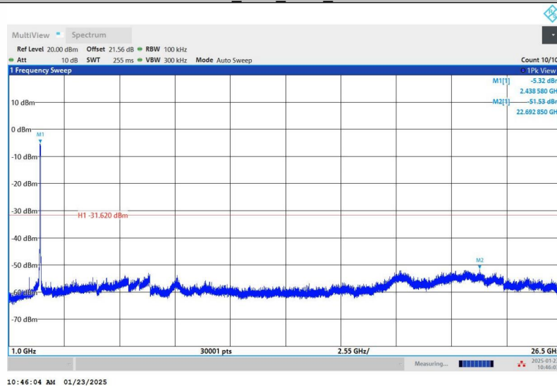
11N40SISO_Ant1_2452_0~Reference
