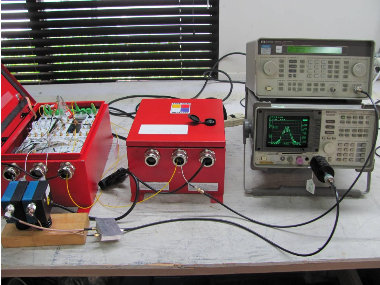
Figure 7. Conducted RF Emissions
