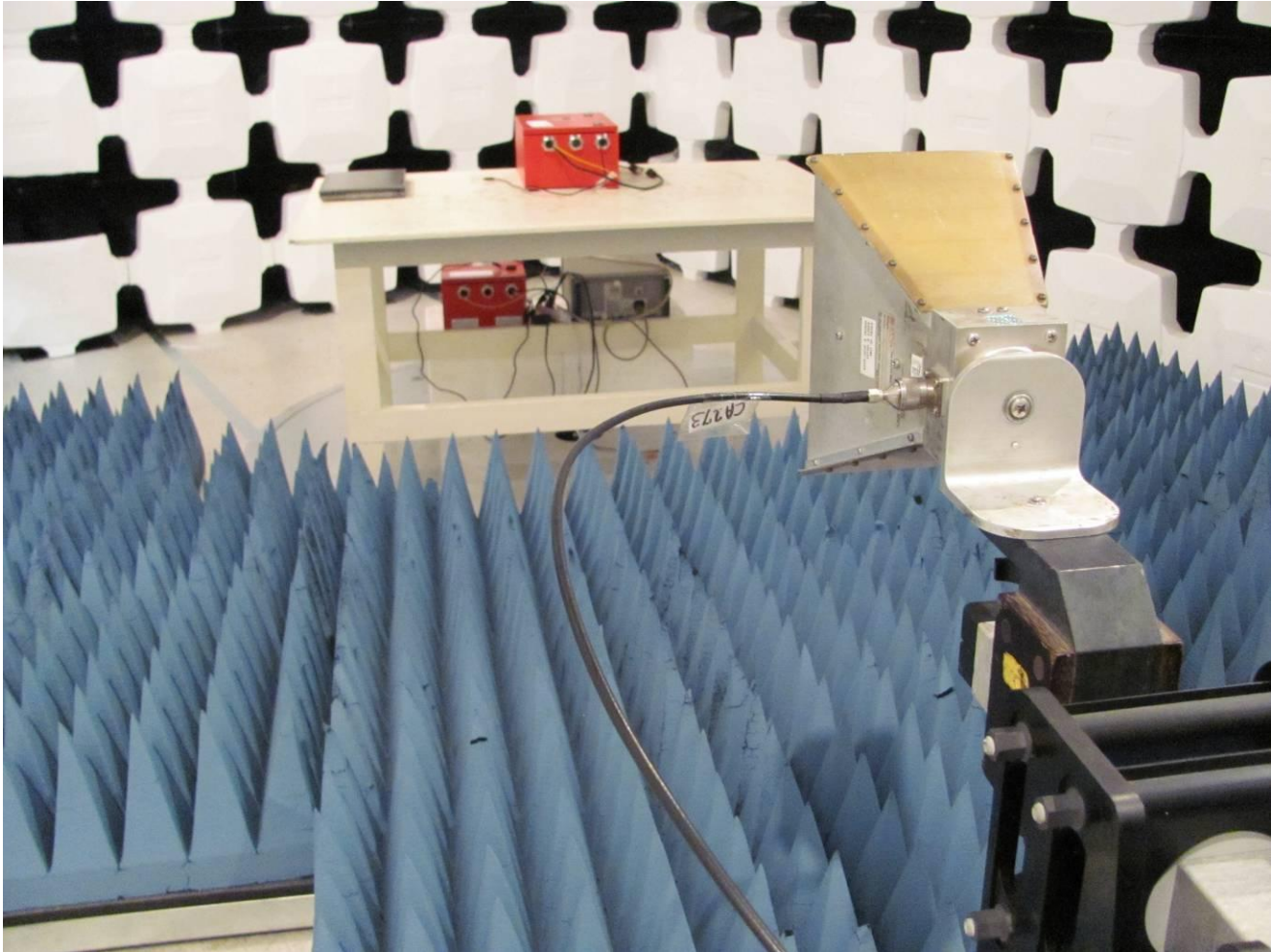
Figure 5. Radiated Emissions, 1 – 6 GHz
