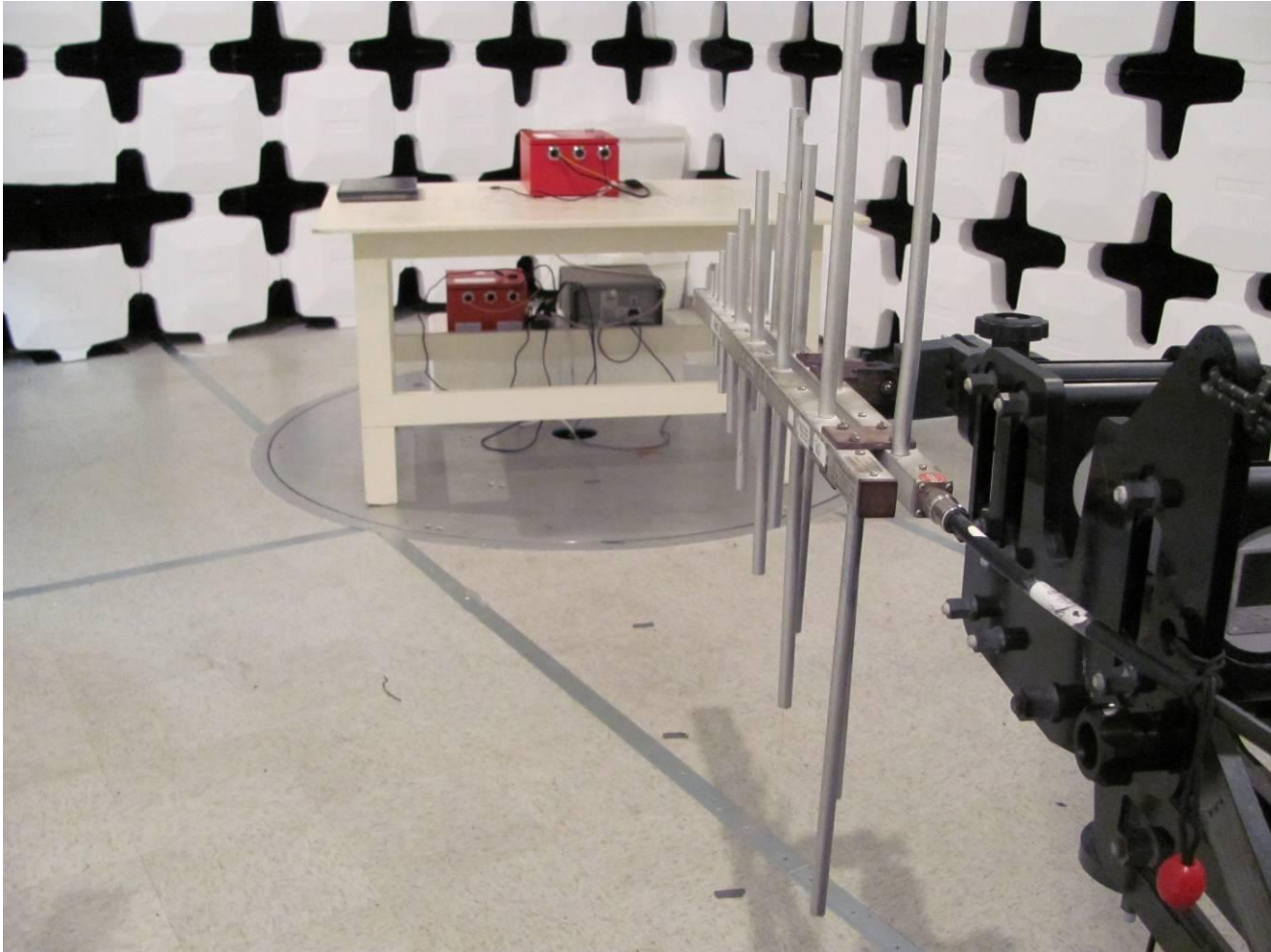
Figure 4. Radiated Emissions, 200 MHz – 1 GHz
