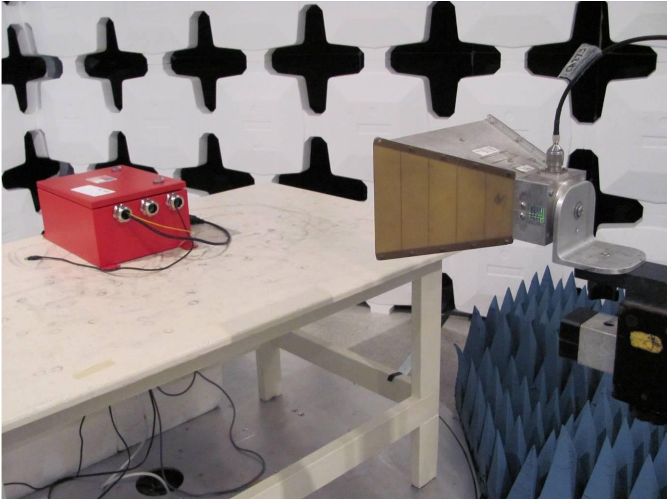
Figure 6. Radiated Emissions, Above 6 GHz
