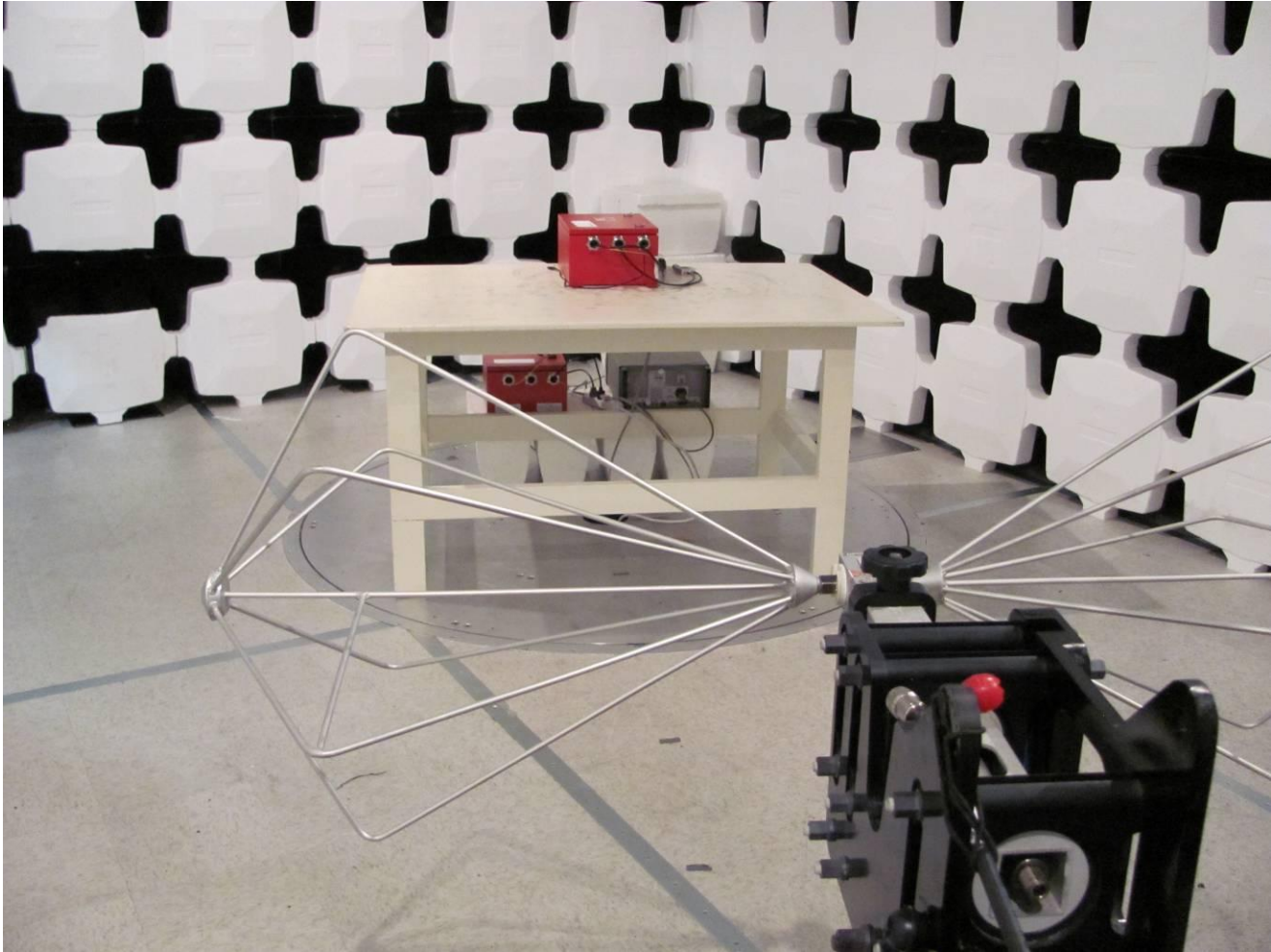
Figure 3. Radiated Emissions, 30 – 200 MHz
