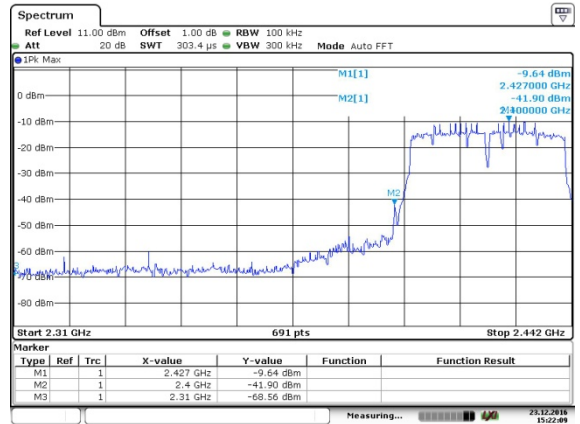
CH03-Bandedge
