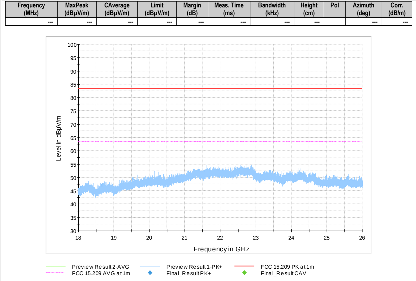
Plot # 8 Radiated Emission 18GHz – 26GHz Mid Ch
