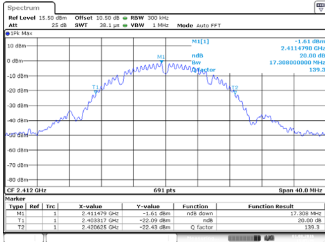
ANT 1(802.11b)
