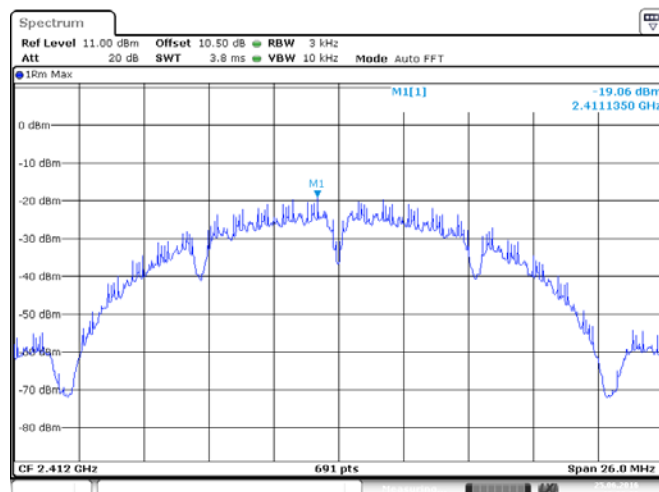
ANT 2(802.11b)
