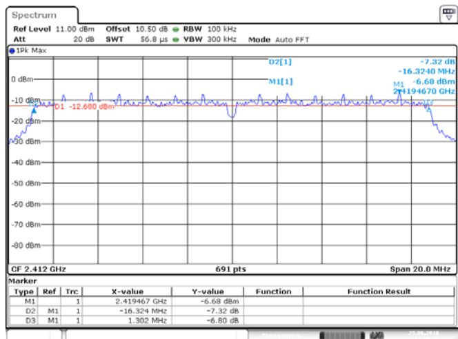
ANT 1(802.11n20)
