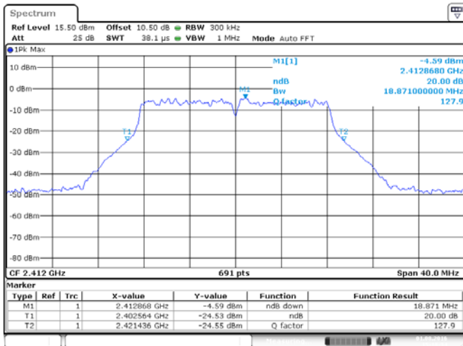
ANT 1(802.11g)
