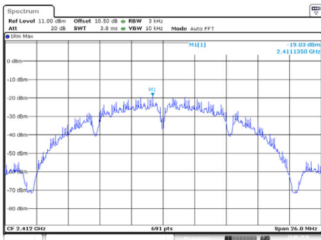
ANT 1(802.11b)
