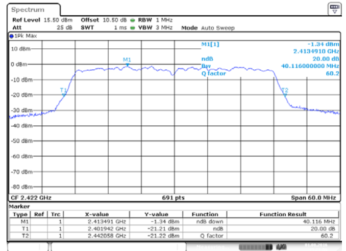
ANT 2(802.11n40)
