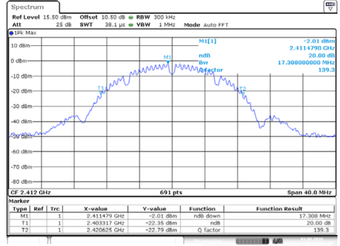
ANT 2(802.11b)
