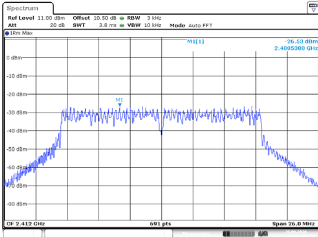
ANT 1(802.11g)
