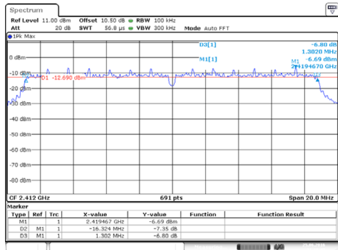
ANT 2(802.11 n20)
