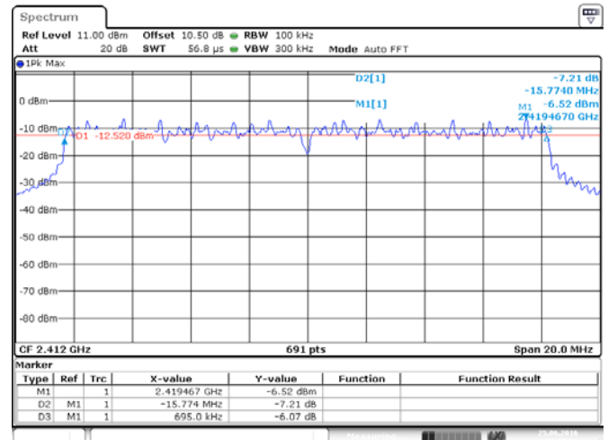
ANT 2(802.11g)
