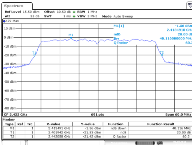
ANT 1(802.11n40)
