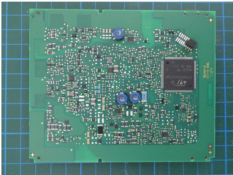
Board 1 – bottom view
