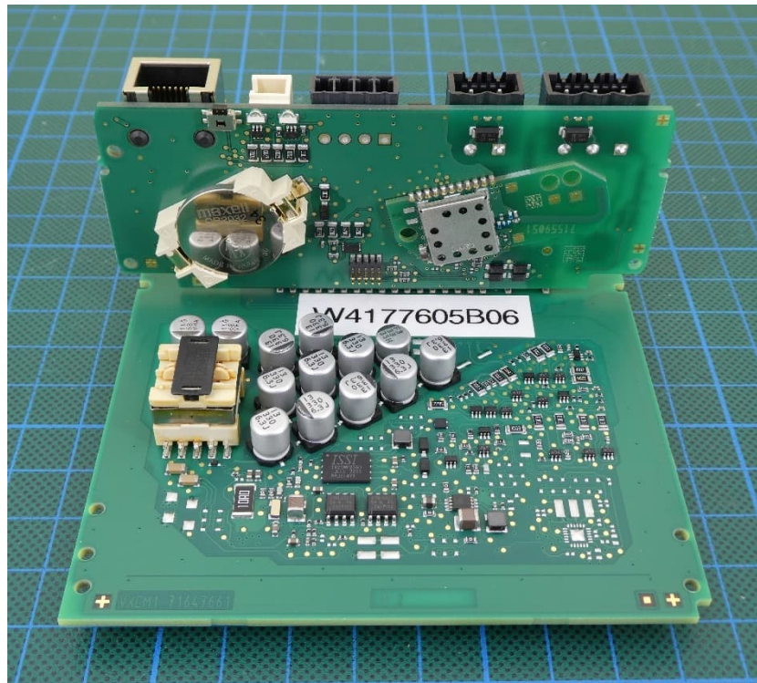
PCBs – front view
