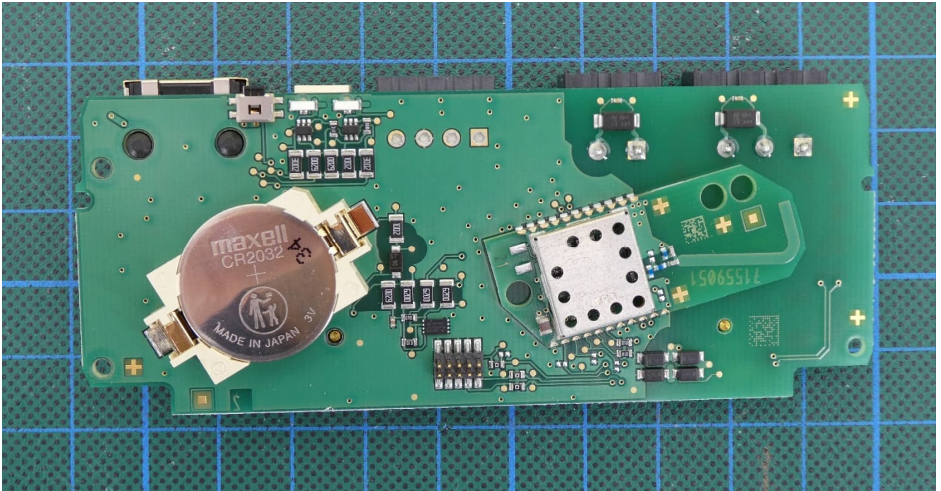
Board 2 – front view
