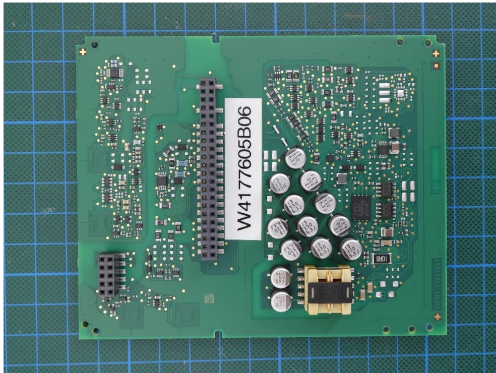
Board 1 – top view
