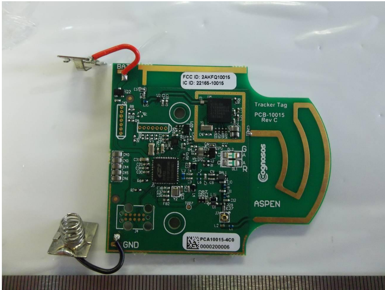
Figure 1. EUT (Cognosos Module) Top View
