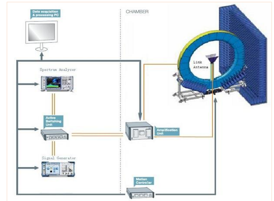
Testing Diagram of SATIMO (暗房测试示意图)
