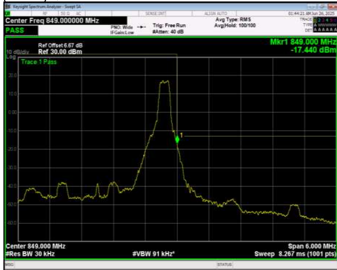
Band26(824-849) QPSK BW=3MHz Channel=27025 RB Size=15 Position=#0 Normal
