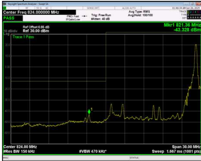
Band26(824-849) 16QAM BW=15MHz Channel=26865 RB Size=75 Position=#0 Normal
