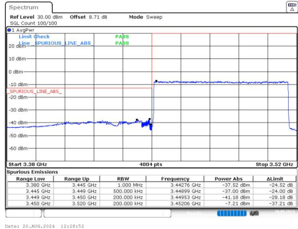
n77(3450-3550) SCS=30kHz DFT_BPSK BW=70MHz LowChannel=632334 RB=180@0 NVNT
