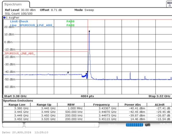
n77(3450-3550) SCS=30kHz DFT_BPSK BW=70MHz LowChannel=632334 RB=1@0 NVNT
