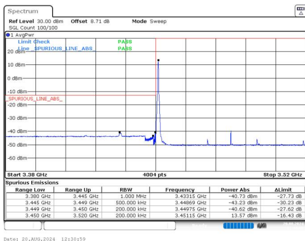
n77(3450-3550) SCS=30kHz DFT_16QAM BW=70MHz LowChannel=632334 RB=1@0 NVNT
