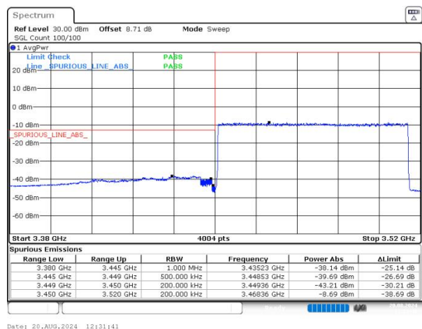
n77(3450-3550) SCS=30kHz DFT_16QAM BW=70MHz LowChannel=632334 RB=180@0 NVNT
