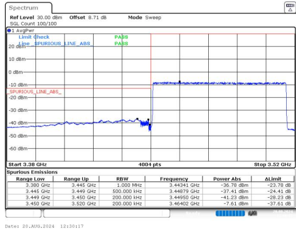
n77(3450-3550) SCS=30kHz DFT_QPSK BW=70MHz LowChannel=632334 RB=180@0 NVNT
