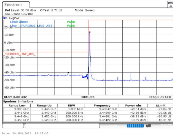
n77(3450-3550) SCS=30kHz DFT_QPSK BW=70MHz LowChannel=632334 RB=1@0 NVNT
