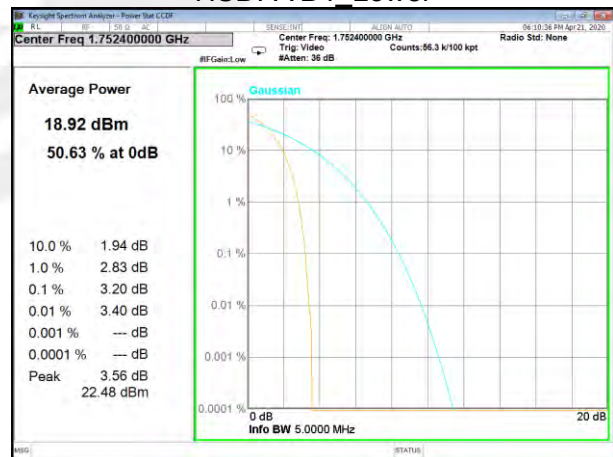
HSDPA B4_Higher
