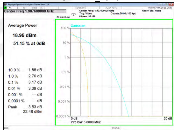
HSDPA B2_Higher
