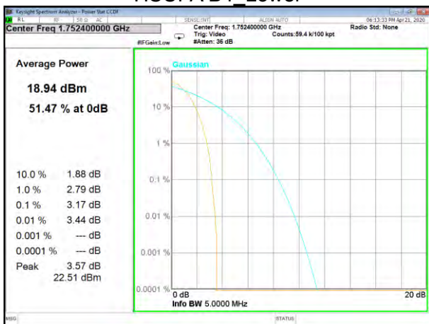
HSUPA B4_Higher
