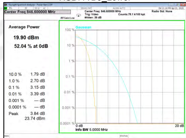
HSDPA B5_Higher
