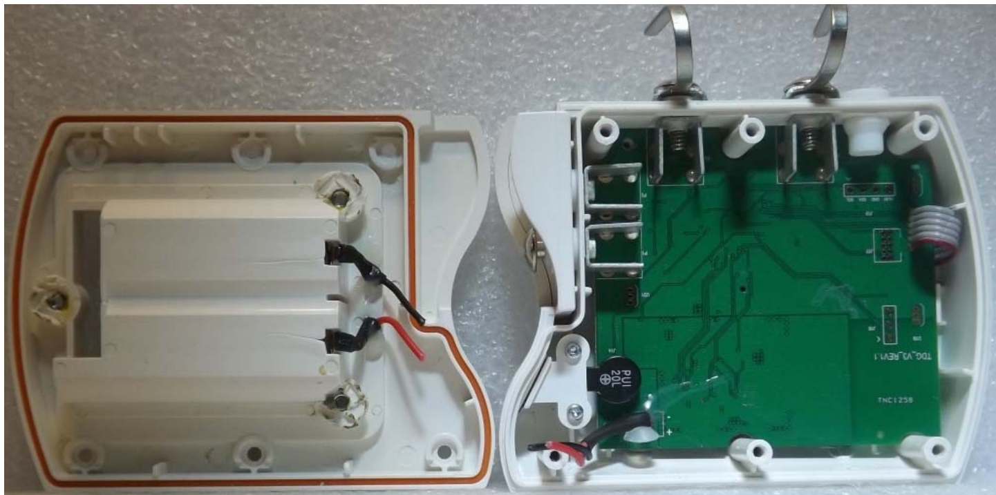
Figure E22.3 – Back Cover Removed
