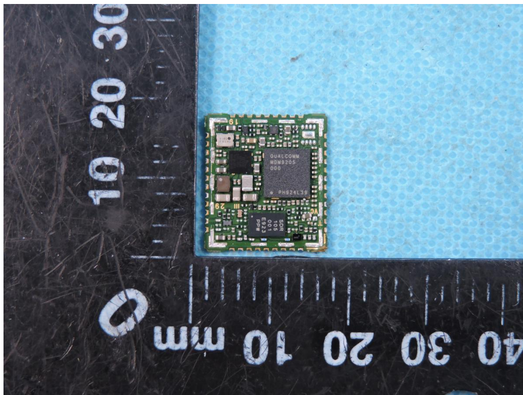
Photo 1(SIM7080G module)
