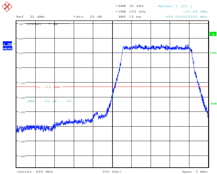
LTE Band12, 1.4MHz bandwidth, QPSK,(1,0) Mode , Below 698MHz
