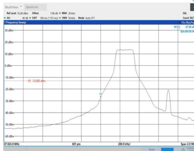
Band26-1.4MHz-16QAM-26797-1RB#5
