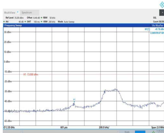
Band40-5MHz-QPSK-39175-25RB#0
