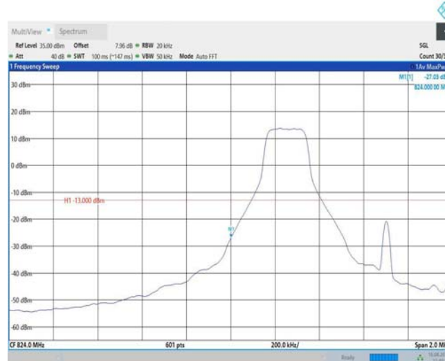
Band26-1.4MHz-QPSK-26797-1RB#5
