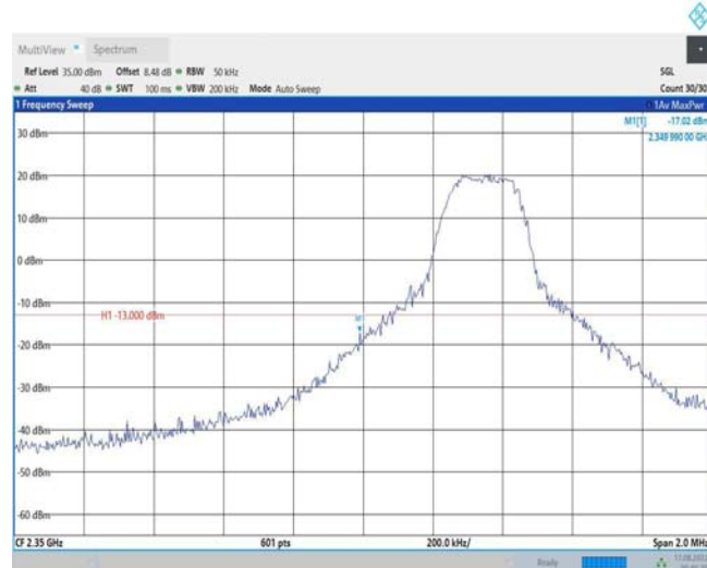
Band40-5MHz-QPSK-39175-1RB#24
