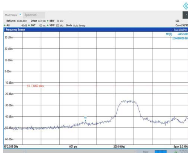
Band40-5MHz-16QAM-38725-25RB#0
