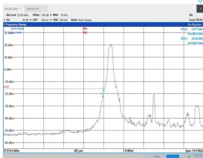
Band26-5MHz-16QAM-26715-1RB#24
