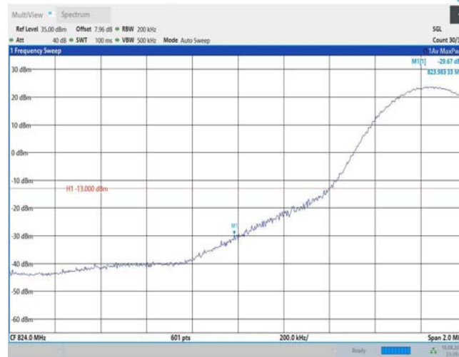
Band26-15MHz-16QAM-26865-1RB#74
