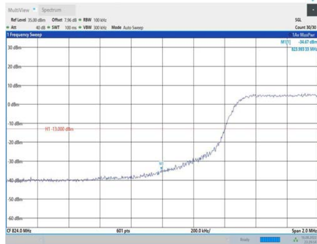
Band26-10MHz-QPSK-26990-1RB#0
