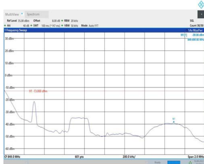
Band26-1.4MHz-16QAM-27033-1RB#5
