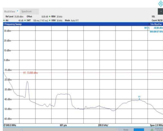
Band26-1.4MHz-QPSK-27033-1RB#5
