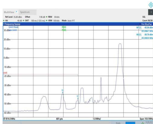
Band26-3MHz-QPSK-26705-15RB#0
