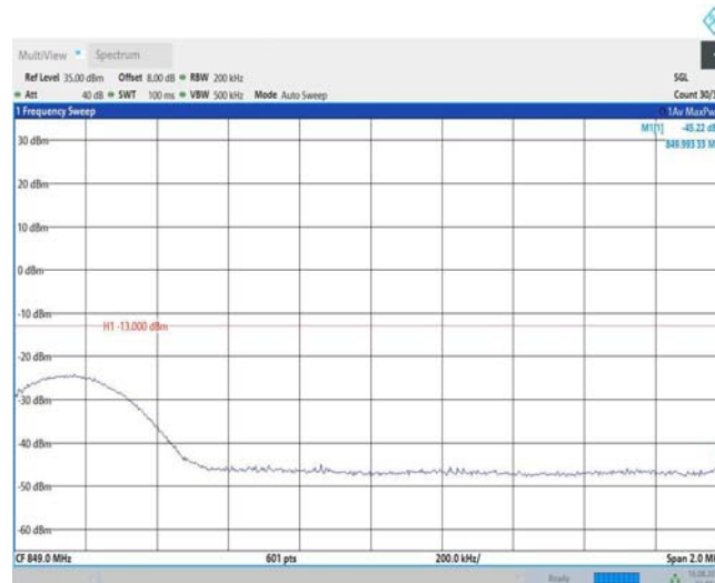
Band26-15MHz-16QAM-26965-1RB#74
