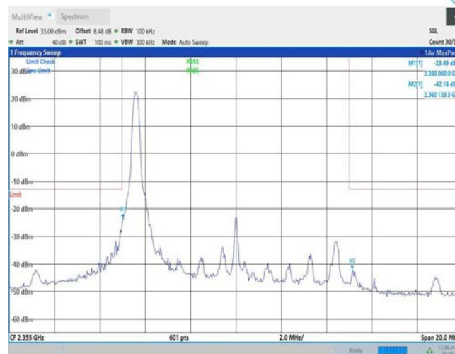
Band40-10MHz-QPSK-39200-1RB#49
