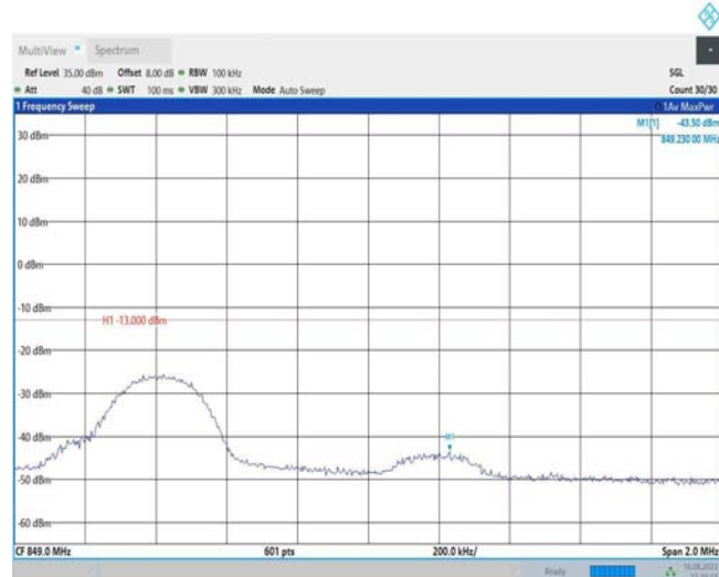
Band26-10MHz-QPSK-26990-1RB#49
