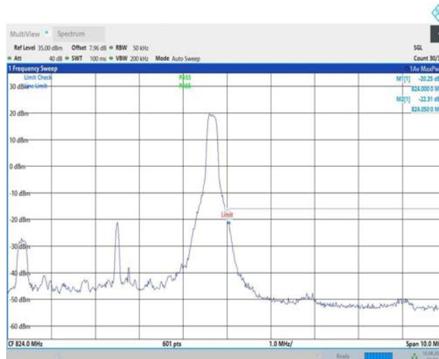
Band26-5MHz-QPSK-26765-25RB#0
