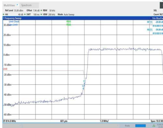
Band26-5MHz-QPSK-26765-1RB#0
