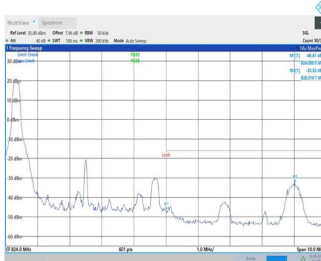
Band26-5MHz-QPSK-26765-1RB#24
