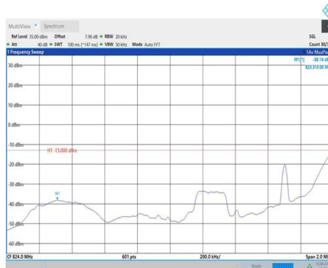
Band26-1.4MHz-16QAM-26797-6RB#0
