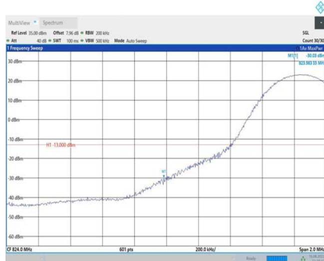
Band26-15MHz-QPSK-26865-1RB#74
