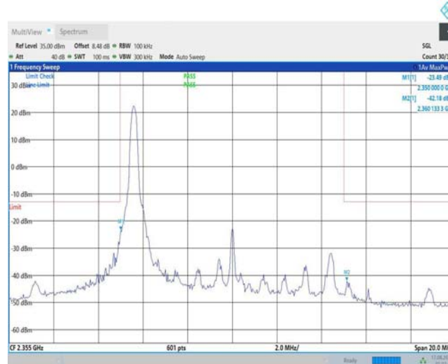
Band40-10MHz-QPSK-39200-1RB#49
