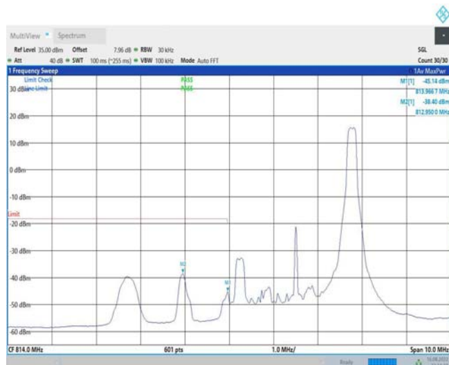
Band26-3MHz-16QAM-26705-15RB#0
