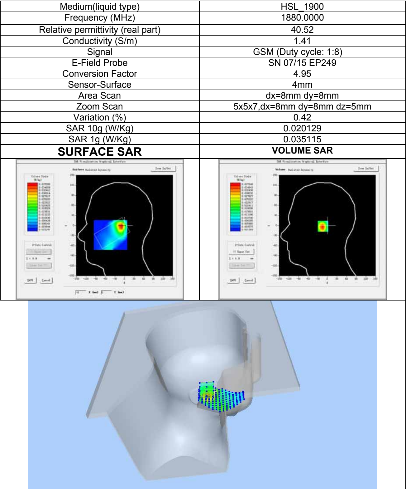
Plot 10: GSM1900, Middle channel (Left Head Tilt) Product Description: Mobile Phone Model: RD70 Test Date: Oct 09,2016
