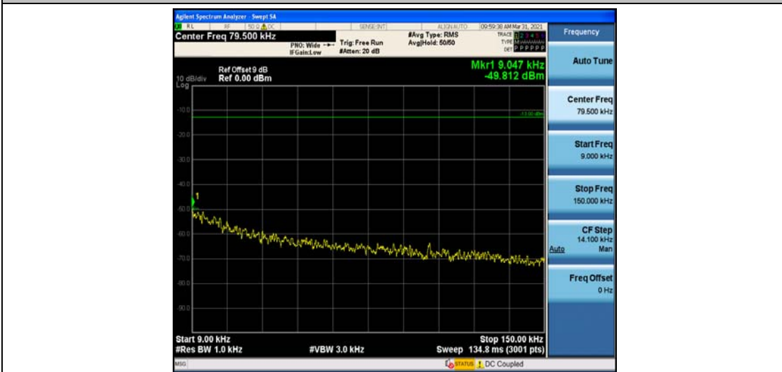
Band25_1.4MHz_16QAM_26047_1RB#0
