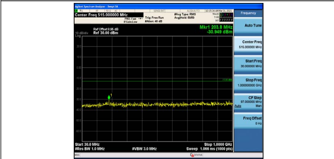
Band25_3MHz_QPSK_26675_1RB#0
