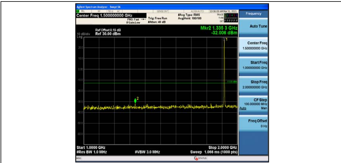
Band25_1.4MHz_QPSK_26683_1RB#0
