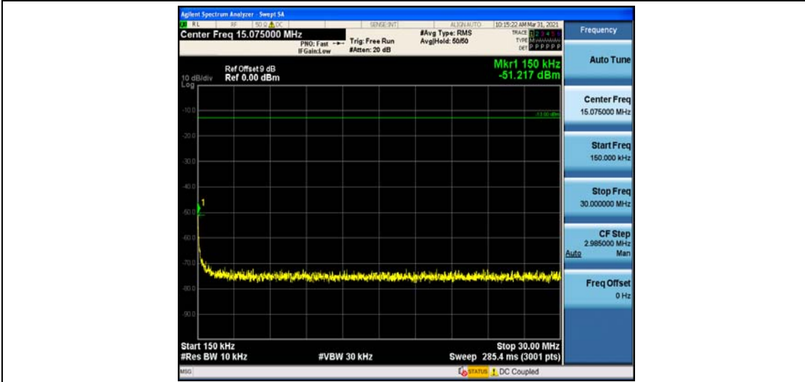
Band25_3MHz_QPSK_26675_1RB#0
