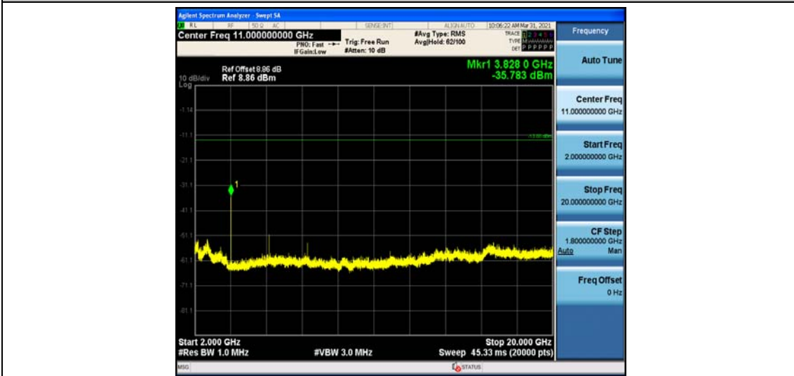
Band25_1.4MHz_16QAM_26047_1RB#0
