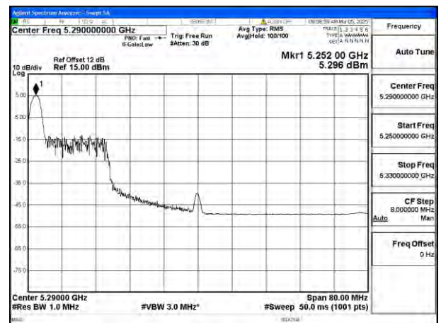
Mode:802.11ax HE80 Tone:26T Frequency:5290MHz Ant:Chain1
