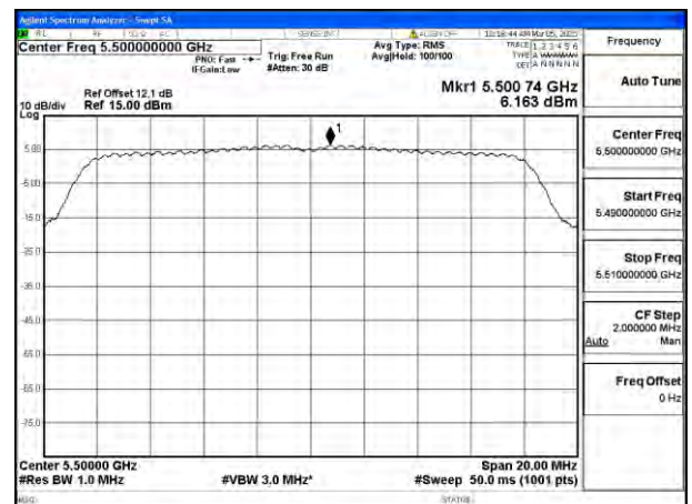
Mode:802.11a Frequency:5500MHz Ant:Chain1
