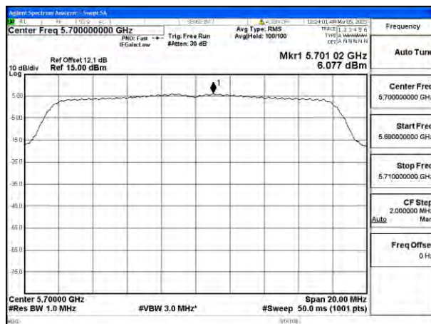
Mode:802.11a Frequency:5700MHz Ant:Chain0
