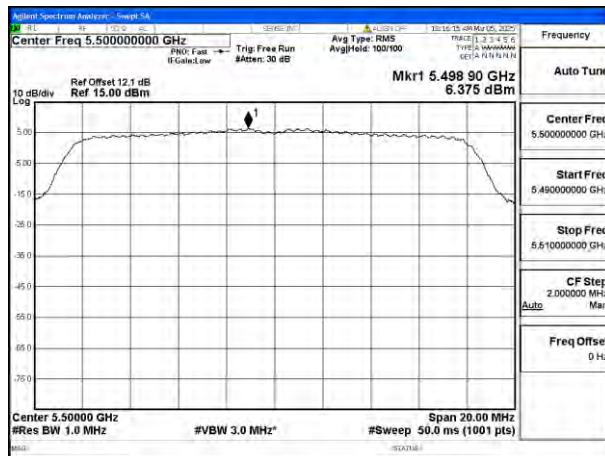
Mode:802.11a Frequency:5500MHz Ant:Chain0
