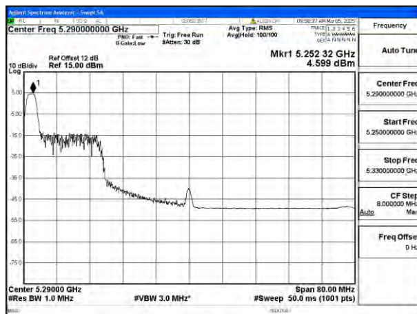
Mode:802.11ax HE80 Tone:26T Frequency:5290MHz Ant:Chain0
