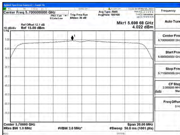
Mode:802.11n HT20 Frequency:5700MHz Ant:Chain0
