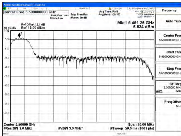
Mode:802.11ax HE20 Tone:26T Frequency:5500MHz Ant:Chain0
