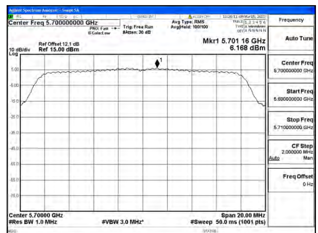
Mode:802.11a Frequency:5700MHz Ant:Chain1
