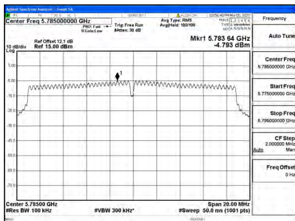
Mode:802.11n HT20 Frequency:5785MHz Ant:Chain1
