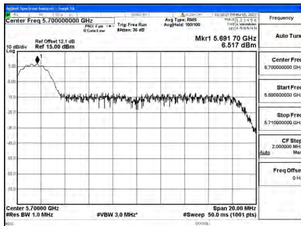
Mode:802.11ax HE20 Tone:26T Frequency:5700MHz Ant:Chain0
