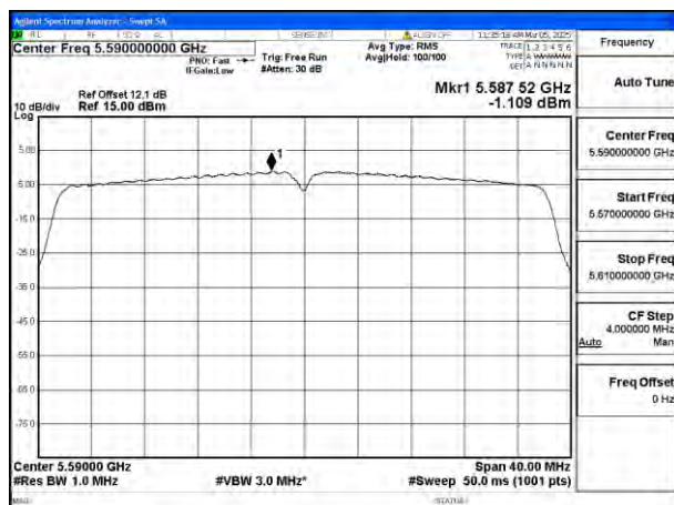
Mode:802.11n HT40 Frequency:5590MHz Ant:Chain1
