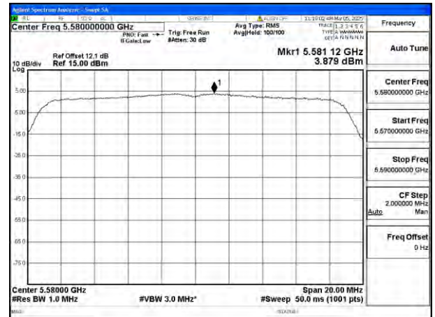
Mode:802.11n HT20 Frequency:5580MHz Ant:Chain0
