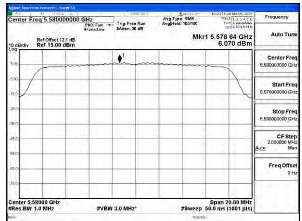
Mode:802.11a Frequency:5580MHz Ant:Chain0
