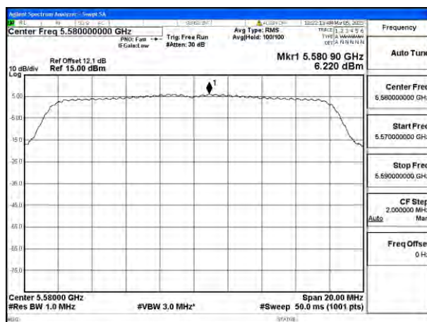
Mode:802.11a Frequency:5580MHz Ant:Chain1
