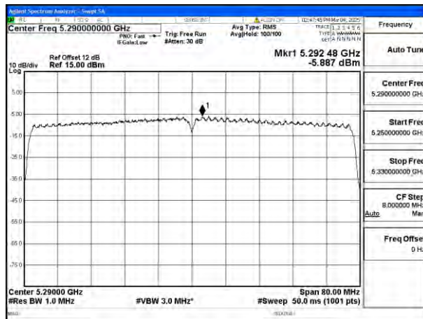
Mode:802.11ac VHT80 Frequency:5290MHz Ant:Chain0
