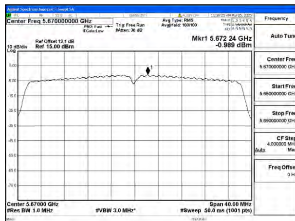
Mode:802.11n HT40 Frequency:5670MHz Ant:Chain1
