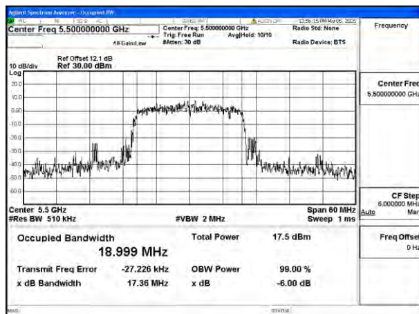
Mode:802.11ax HE20 Frequency:5500MHz Ant:Chain0
