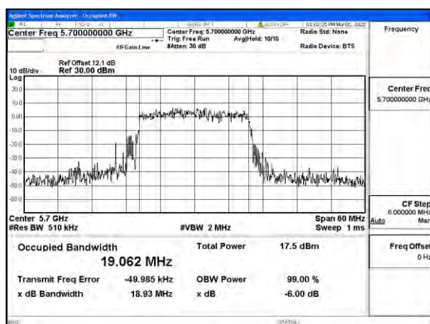
Mode:802.11ax HE20 Frequency:5700MHz Ant:Chain0
