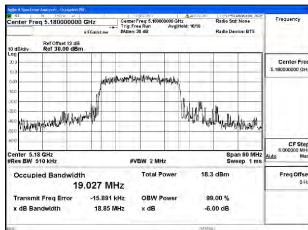
Mode:802.11ax HE20 Frequency:5180MHz Ant:Chain1
