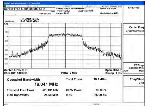
Mode:802.11n HT20 Frequency:5785MHz Ant:Chain0
