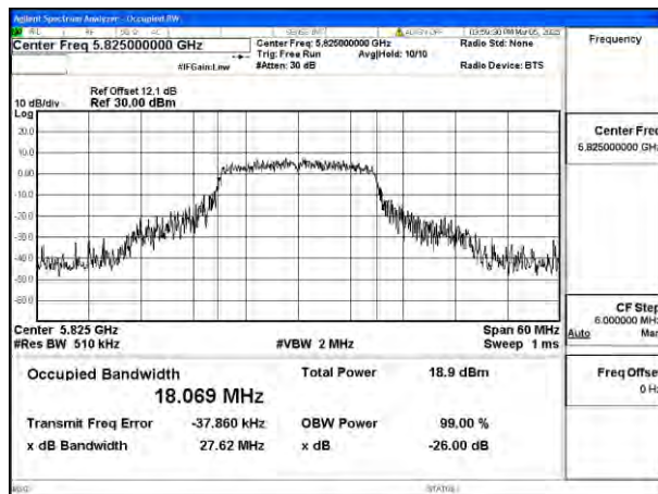
Mode:802.11n HT20 Frequency:5825MHz Ant:Chain0
