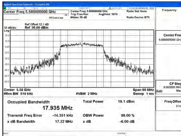
Mode:802.11n HT20 Frequency:5580MHz Ant:Chain1
