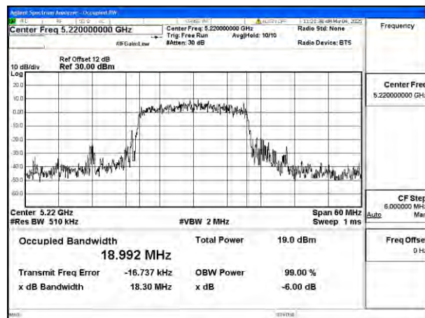
Mode:802.11ax HE20 Frequency:5220MHz Ant:Chain0
