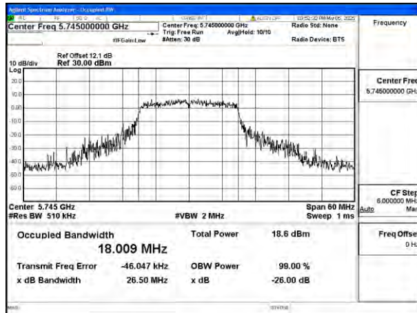
Mode:802.11n HT20 Frequency:5745MHz Ant:Chain0
