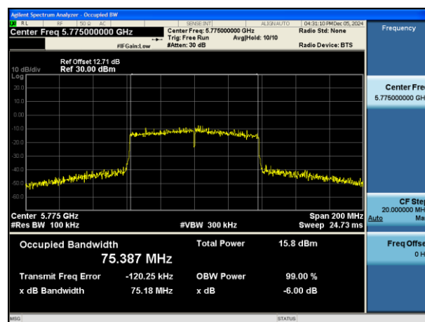
Mode:802.11ac VHT80 Frequency:5775MHz Ant:Chain1
