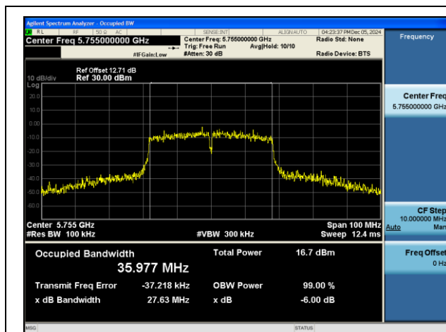
Mode:802.11ac VHT40 Frequency:5755MHz Ant:Chain1
