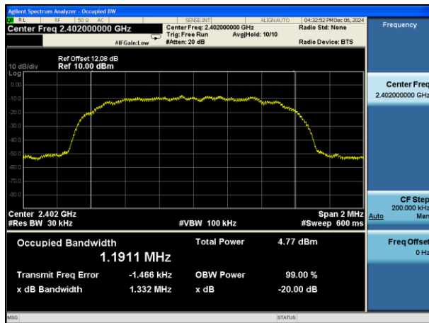
Test Mode:8DPSK(3DH5) 2402MHz
