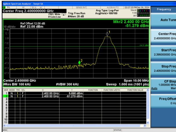
CH0(Hopping off)
