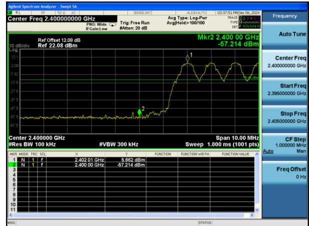
CH0(Hopping on)
