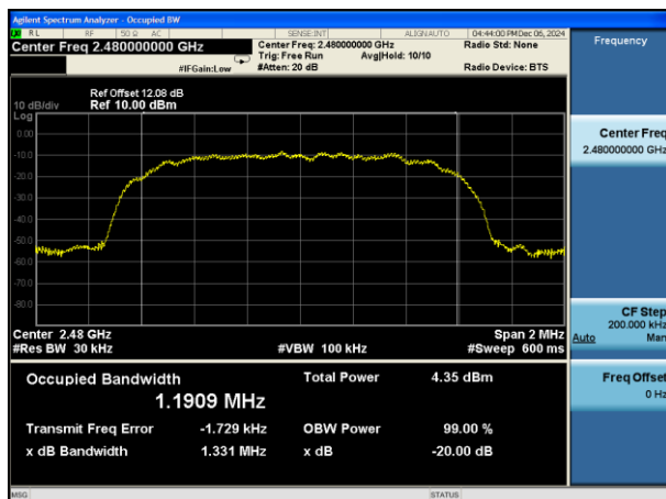
Test Mode:8DPSK(3DH5) 2480MHz
