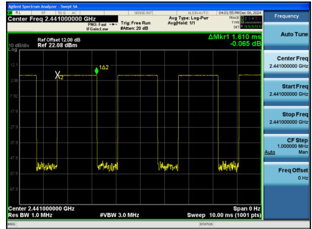
Test Mode:GFSK(DH3) 2441MHz
