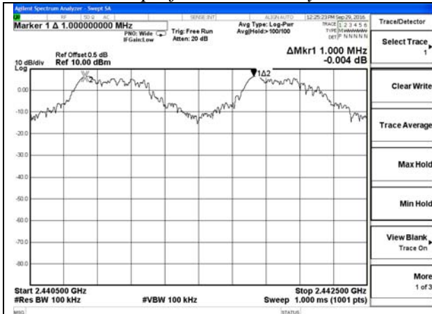
Test Plot Of Frequency Separation (1Mbps)
