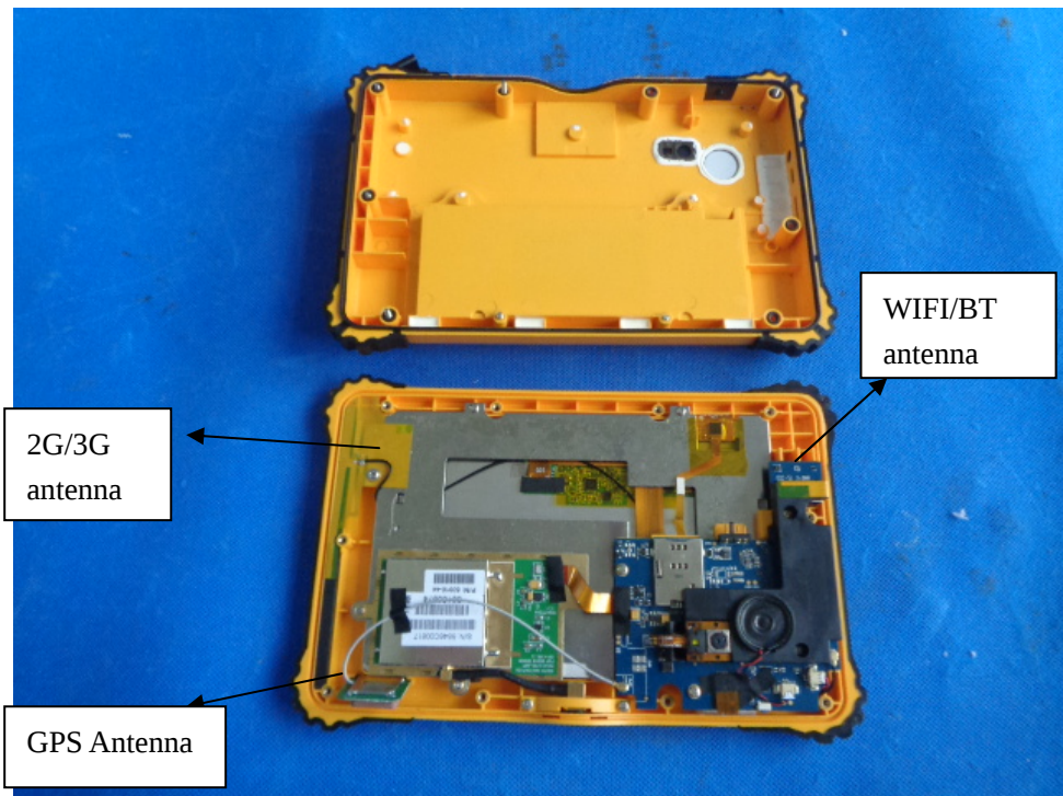
Photo 14 2G/3G antenna
