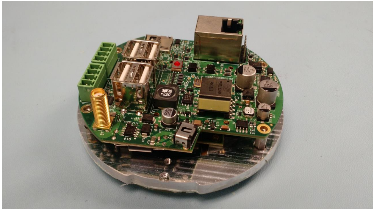
Main PCBA + Heat Spreader + Daughter PCBA
