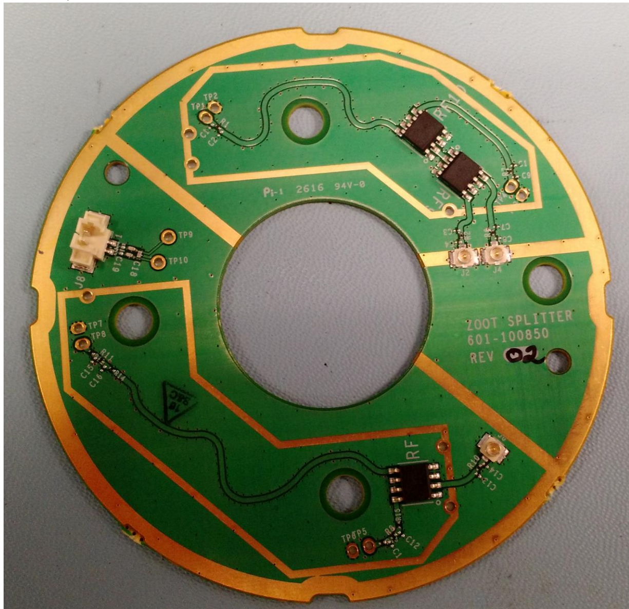
Antenna Splitter PCBA
