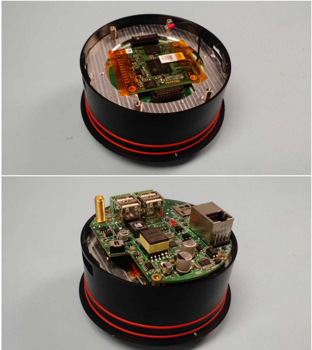
Electronics installed in Trim Ring with Antenna PCBA
