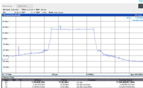
Band66-20MHz-16QAM-132322-100RB#0
