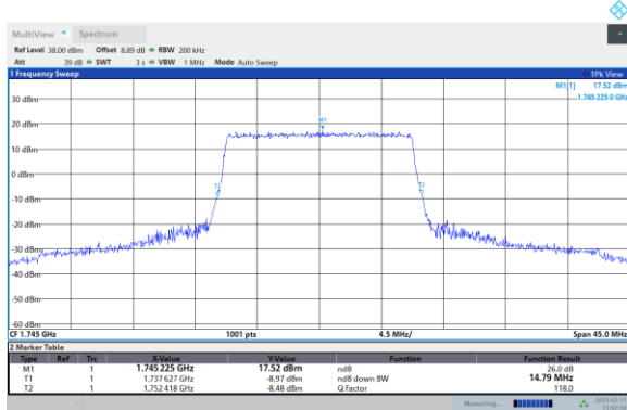
Band66-15MHz-64QAM-132047-75RB#0
