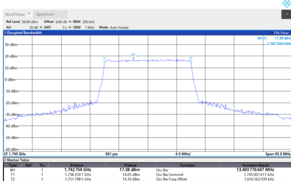
Band66-15MHz-64QAM-132047-75RB#0
