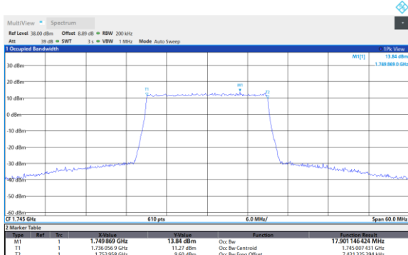
Band66-20MHz-256QAM-132322-100RB#0
