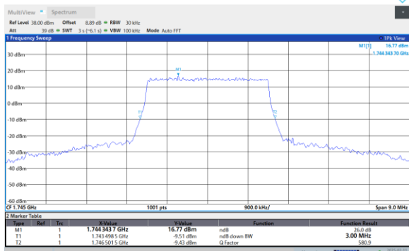
Band66-3MHz-64QAM-131987-15RB#0
