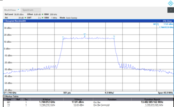
Band66-15MHz-256QAM-132047-75RB#0
