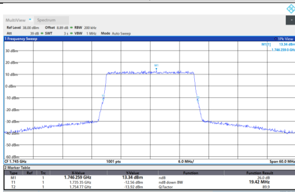
Band66-20MHz-256QAM-132322-100RB#0
