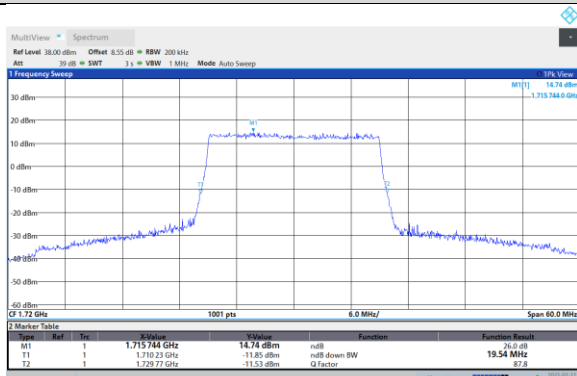
Band66-20MHz-64QAM-132572-100RB#0
