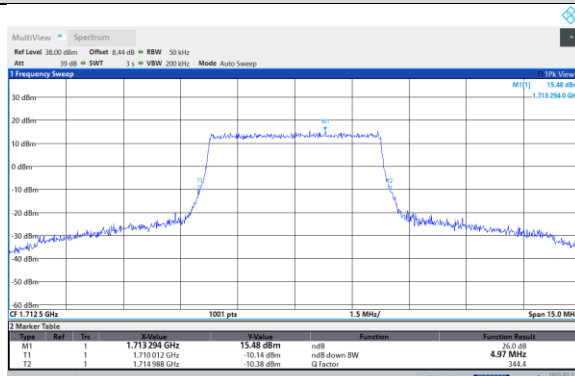
Band66-5MHz-16QAM-132647-25RB#0
