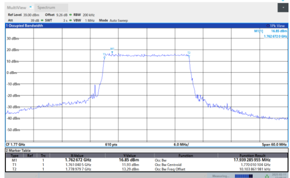
Band66-20MHz-64QAM-132322-100RB#0
