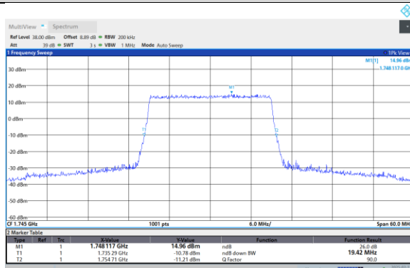
Band66-20MHz-256QAM-132072-100RB#0
