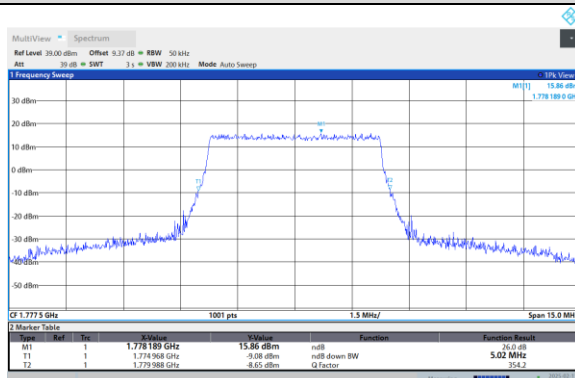
Band66-5MHz-64QAM-132322-25RB#0
