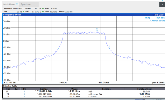
Band66-1.4MHz-256QAM-132665-6RB#0
