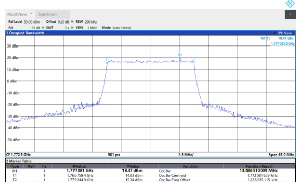
Band66-15MHz-64QAM-132322-75RB#0
