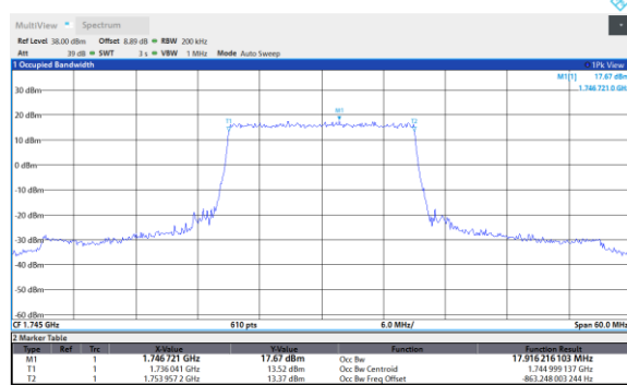
Band66-20MHz-16QAM-132072-100RB#0
