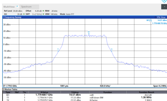
Band66-3MHz-QPSK-132322-15RB#0
