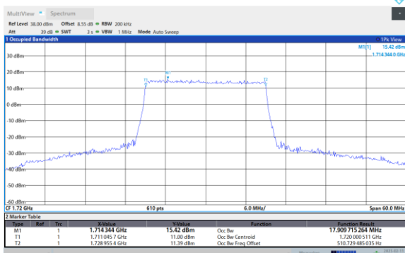
Band66-20MHz-64QAM-132572-100RB#0
