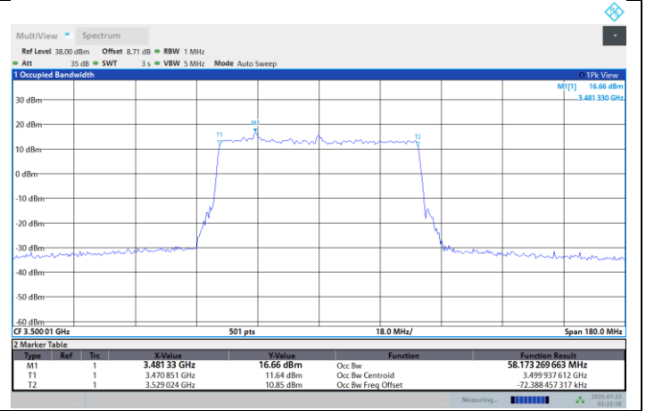
N77-3450-3550-PC2-30-60-M-DFT-256QAM-Outer_Full
