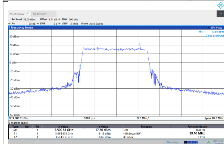
N77-3450-3550-PC2-30-30-M-DFT-64QAM-Outer_Full
