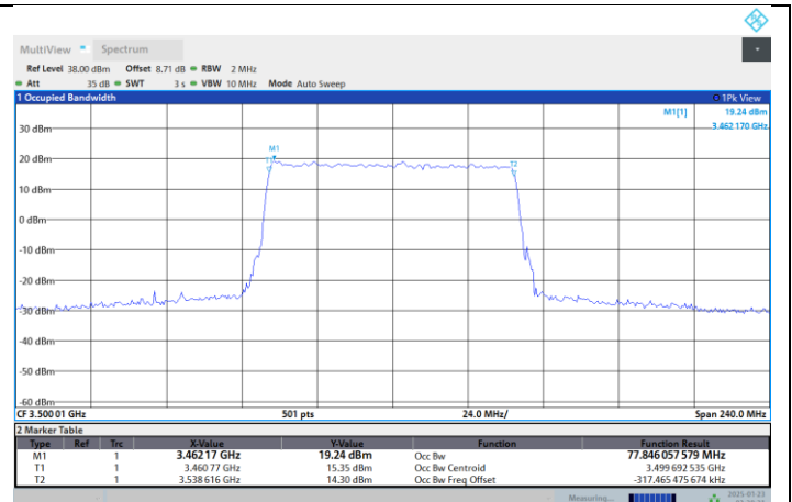
N77-3450-3550-PC2-30-80-M-DFT-16QAM-Outer_Full
