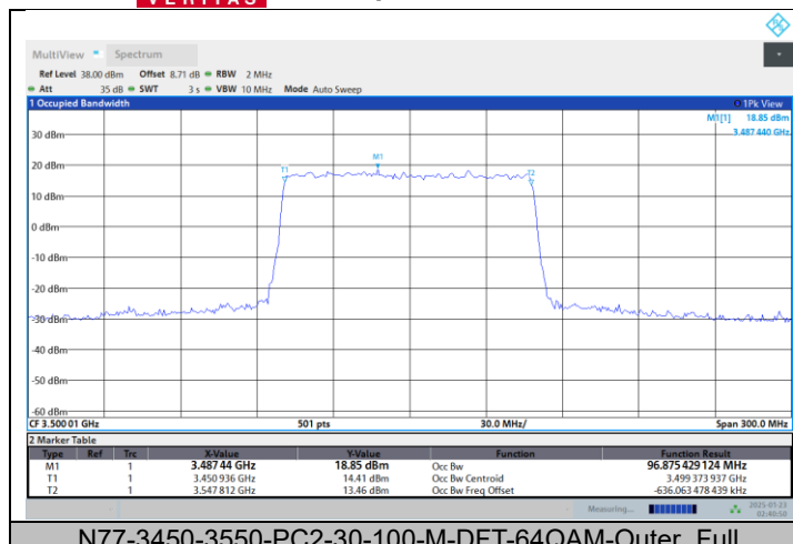
N77-3450-3550-PC2-30-100-M-DFT-64QAM-Outer_Full
