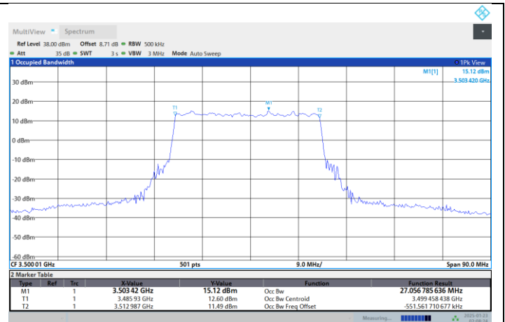
N77-3450-3550-PC2-30-30-M-DFT-256QAM-Outer Full
