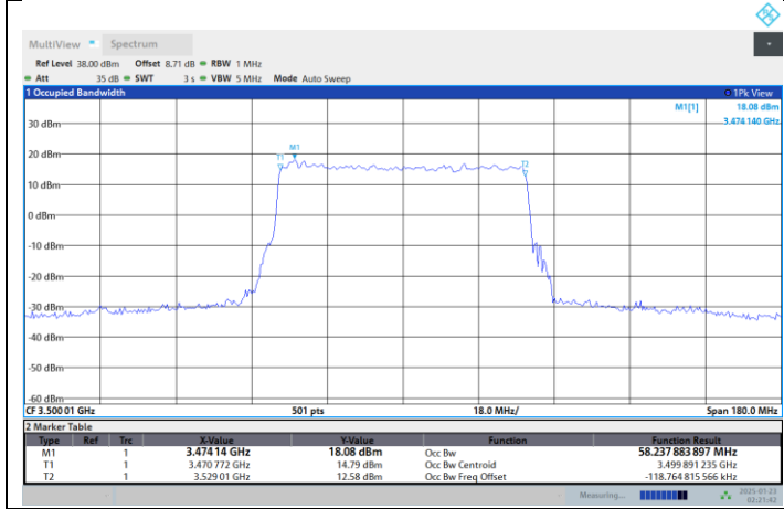
N77-3450-3550-PC2-30-60-M-DFT-64QAM-Outer_Full
