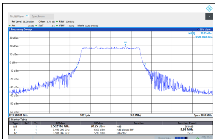
N77-3450-3550-PC2-30-10-M-DFT-PI2BPSK-Outer_Full
