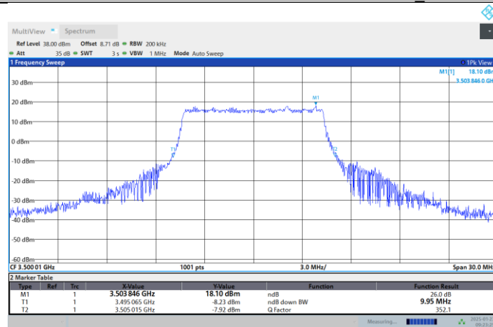
N77-3450-3550-PC2-30-10-M-DFT-64QAM-Outer_Full
