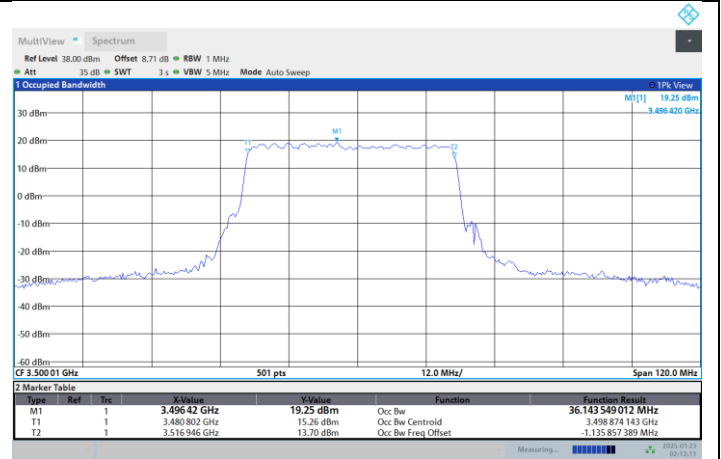
N77-3450-3550-PC2-30-40-M-DFT-64QAM-Outer Full
