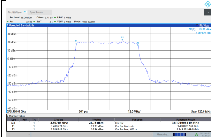
N77-3450-3550-PC2-30-40-M-DFT-PI2BPSK-Outer Full
