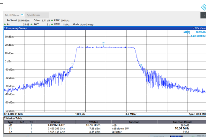
N77-3450-3550-PC2-30-10-M-DFT-QPSK-Outer_Full
