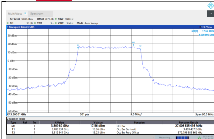
N77-3450-3550-PC2-30-30-M-DFT-64QAM-Outer Full
