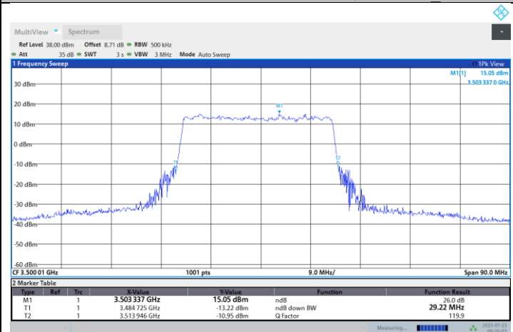
N77-3450-3550-PC2-30-30-M-DFT-256QAM-Outer_Full
