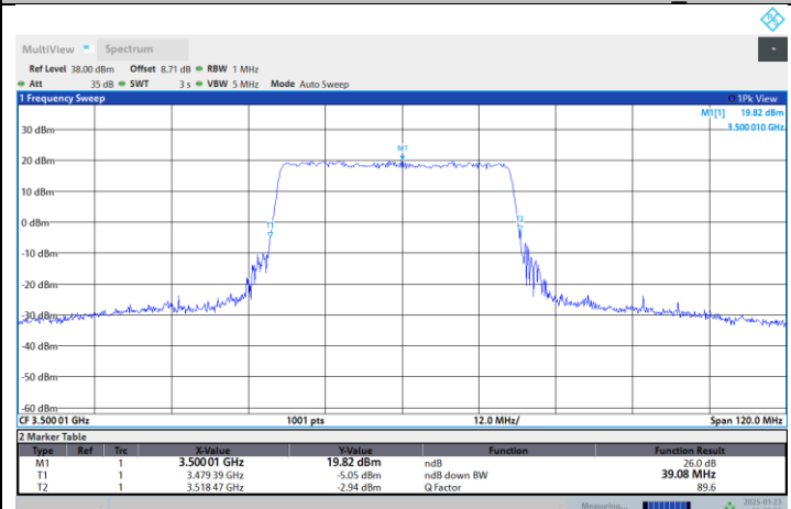
N77-3450-3550-PC2-30-40-M-DFT-QPSK-Outer_Full
