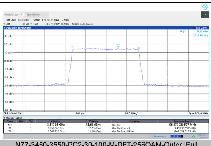
N77-3450-3550-PC2-30-100-M-DFT-256QAM-Outer_Full
