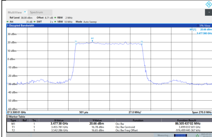
N77-3450-3550-PC2-30-90-M-DFT-PI2BPSK-Outer_Full
