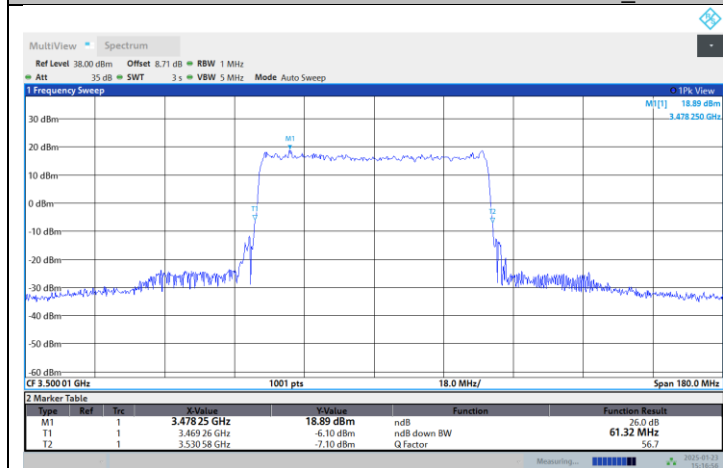
N77-3450-3550-PC2-30-60-M-DFT-QPSK-Outer_Full
