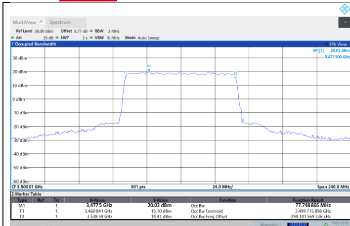
N77-3450-3550-PC2-30-80-M-DFT-QPSK-Outer_Full
