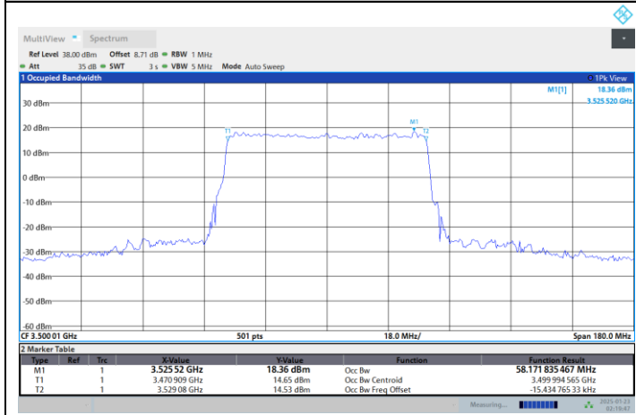
N77-3450-3550-PC2-30-60-M-DFT-QPSK-Outer_Full
