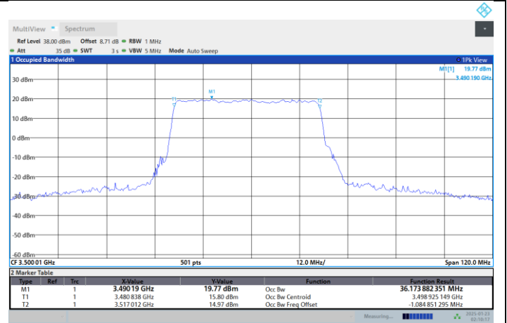
N77-3450-3550-PC2-30-40-M-DFT-QPSK-Outer Full
