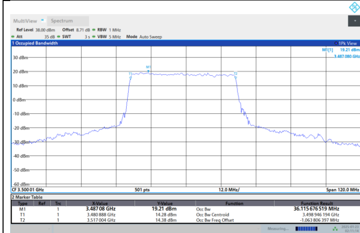
N77-3450-3550-PC2-30-40-M-DFT-16QAM-Outer Full
