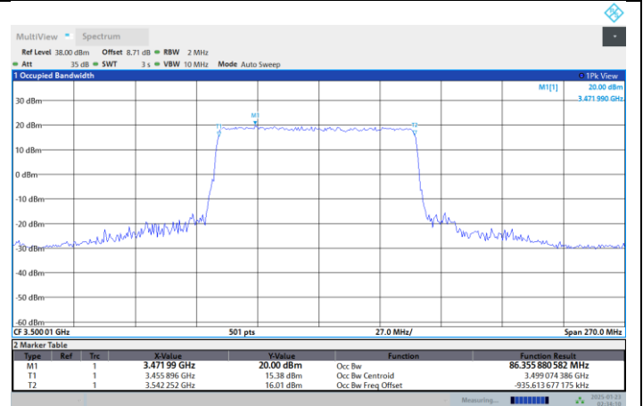
N77-3450-3550-PC2-30-90-M-DFT-QPSK-Outer_Full
