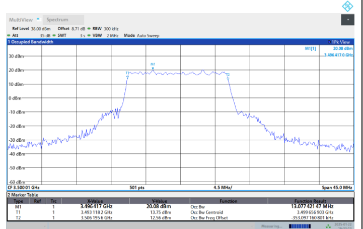
N77-3450-3550-PC2-30-15-M-DFT-PI2BPSK-Outer_Full
