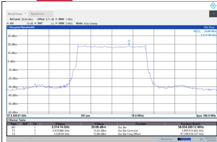
N77-3450-3550-PC2-30-60-M-DFT-PI2BPSK-Outer_Full
