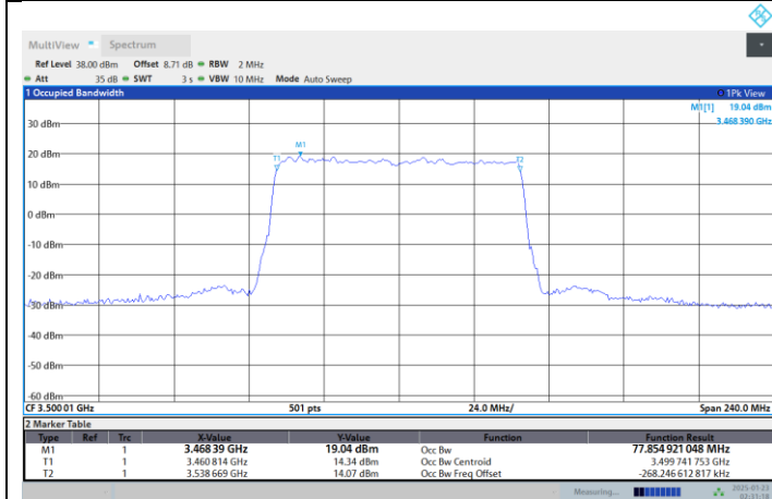
N77-3450-3550-PC2-30-80-M-DFT-64QAM-Outer_Full
