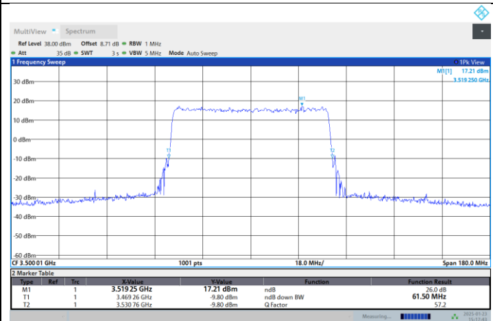
N77-3450-3550-PC2-30-60-M-DFT-16QAM-Outer_Full
