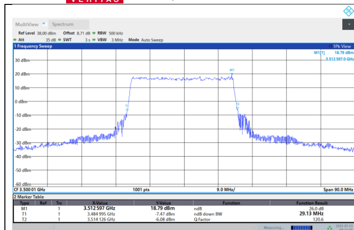
N77-3450-3550-PC2-30-30-M-DFT-QPSK-Outer_Full
