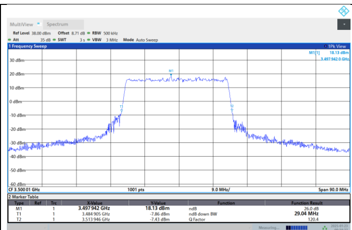
N77-3450-3550-PC2-30-30-M-DFT-16QAM-Outer_Full
