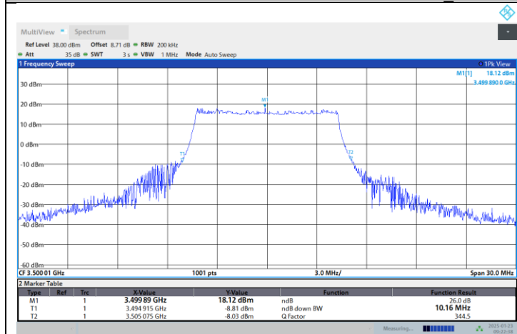
N77-3450-3550-PC2-30-10-M-DFT-16QAM-Outer_Full
