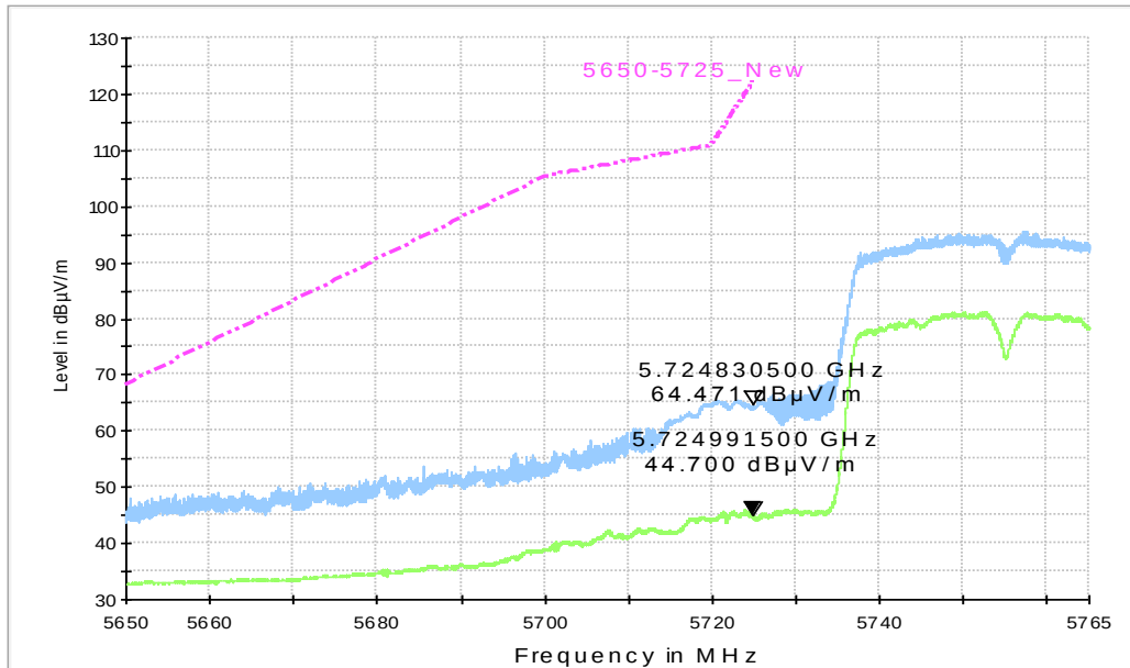
Fig. 51 Band Edges (802.11n-HT40, 5755MHz)
