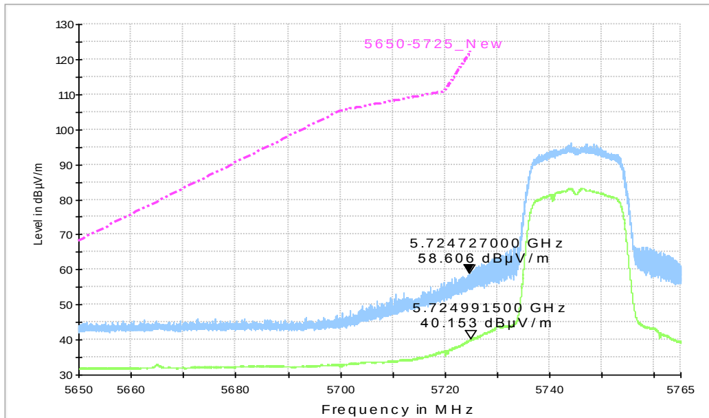
Fig. 49 Band Edges (802.11n-HT20, 5745MHz)
