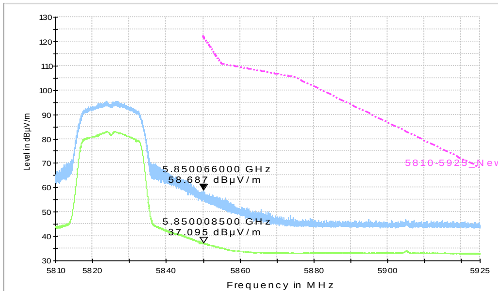
RE - Power-5.810GHz-5.925GHz
