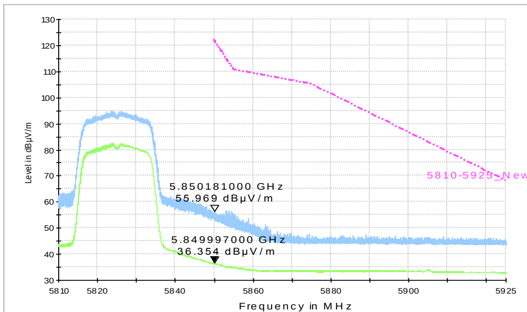
Fig. 50 Band Edges (802.11n-HT20, 5825MHz)
