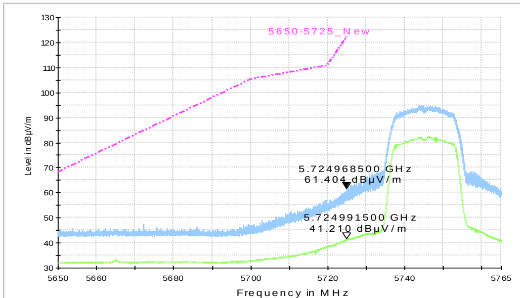
RE - Power-5.650GHz-5.765GHz
