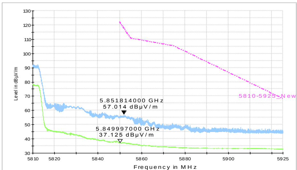
Fig. 52 Band Edges (802.11n-HT40, 5795MHz)
