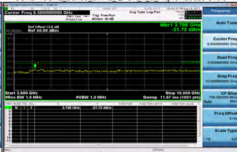
3GHz~10GHz_Band5_5MHz_QPSK_1_0_HighCH20625-846.5
