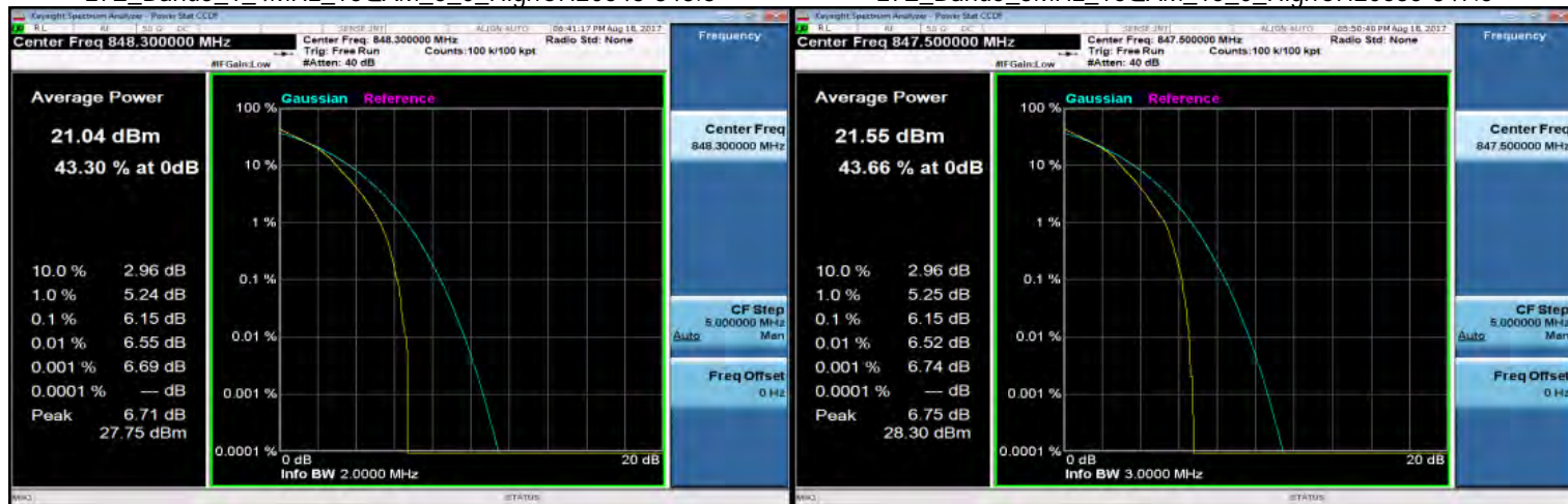
LTE_Band5_1_4MHz_16QAM_6_0_HighCH20643-848.3
