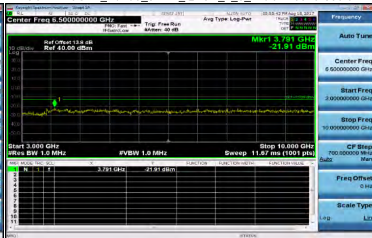
3GHz~10GHz_Band5_3MHz_QPSK_1_0_MidCH20525-836.5
