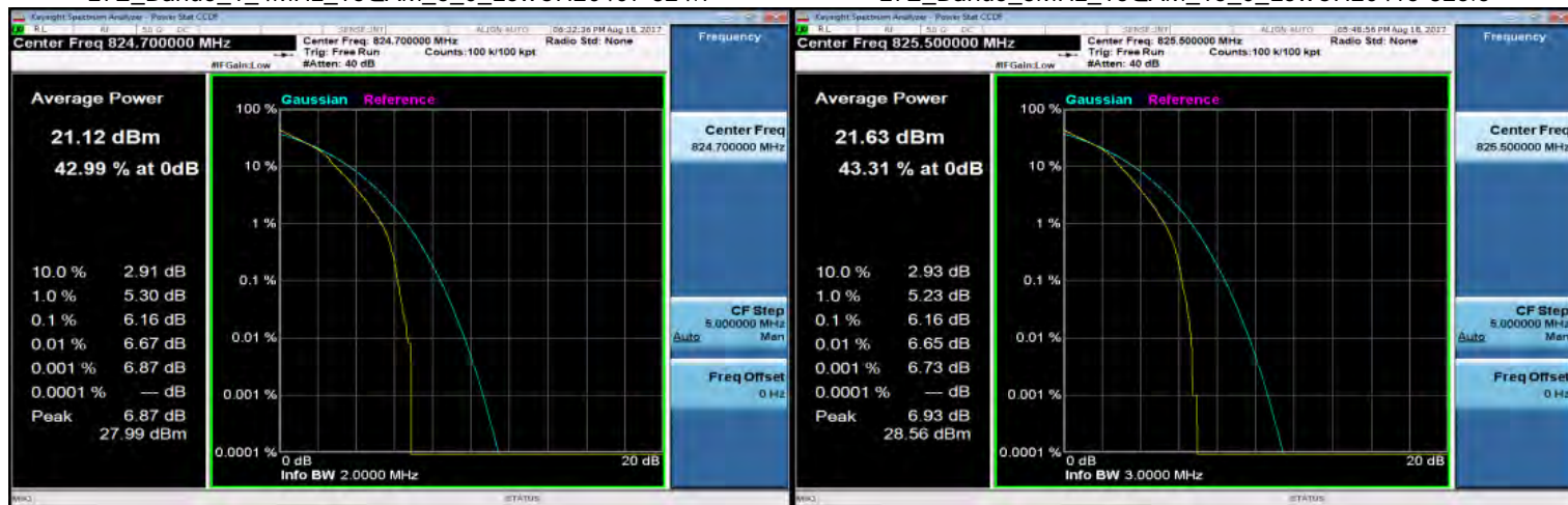
LTE_Band5_1_4MHz_16QAM_6_0_LowCH20407-824.7
