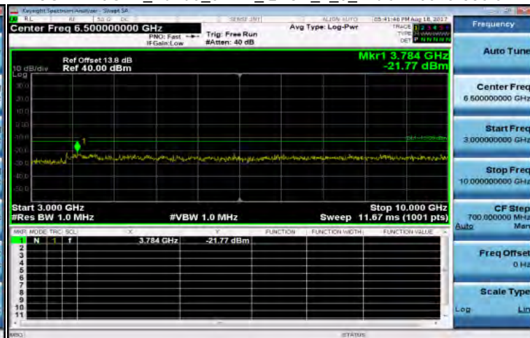
3GHz~10GHz_Band5_5MHz_QPSK_1_0_MidCH20525-836.5
