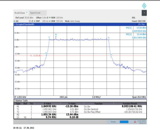
1-N2--15-10-L-1-DFT-QPSK-Outer_Full-50@0-Ant0-8.953-9.740-≤10-PASS
