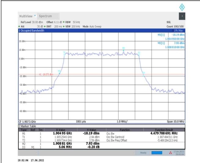
1-N2--15-5-H-5-DFT-256QAM-Outer_Full-25@0-Ant0-4.48-5.060-≤5-PASS
