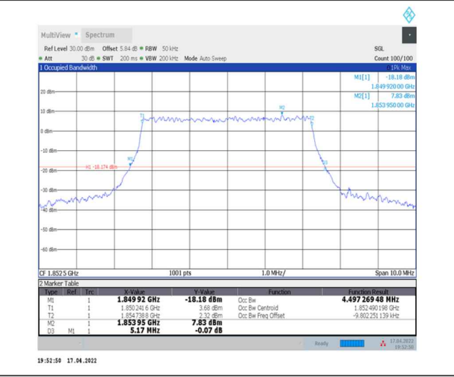
1-N2--15-5-L-8-CP-64QAM-Outer_Full-25@0-Ant0-4.497-5.170-≤5-PASS
