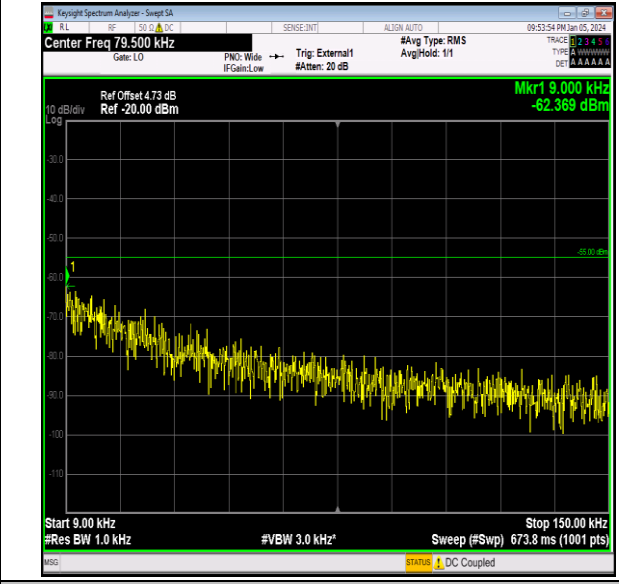
Band41_10MHz_64QAM_40640_1RB#0_0.009~0.15_0.009~0.15
