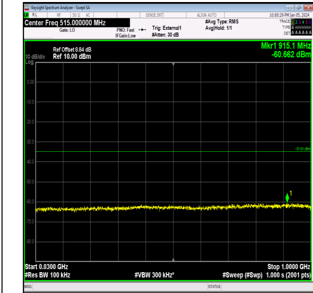
Band41_10MHz_64QAM_41190_1RB#0_30~1000_30~10 00
