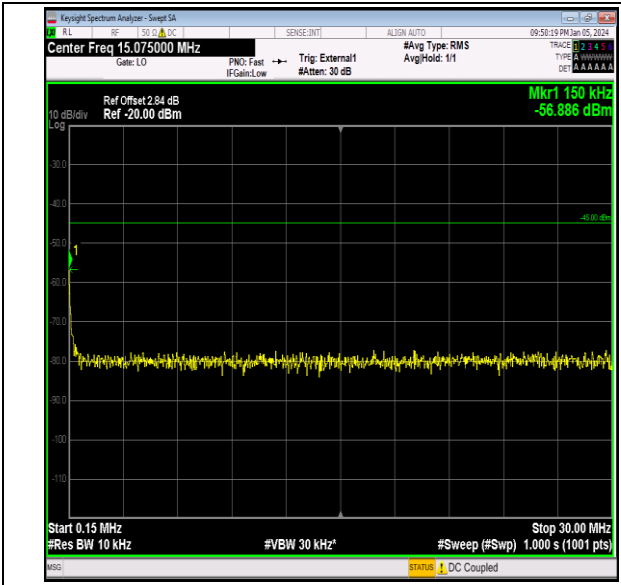
Band41_10MHz_QPSK_40640_1RB#0_0.15~30_0.15~30
