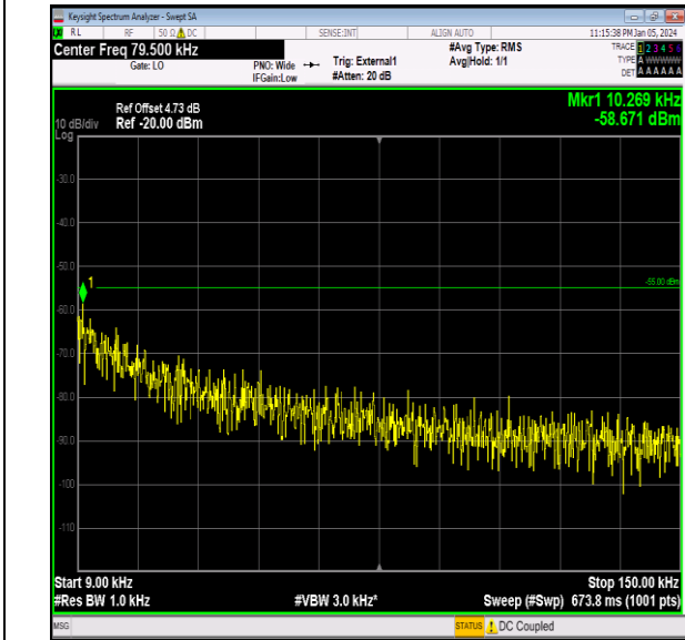
Band41_15MHz_16QAM_41165_1RB#0_0.009~0.15_0.00 9~0.15
