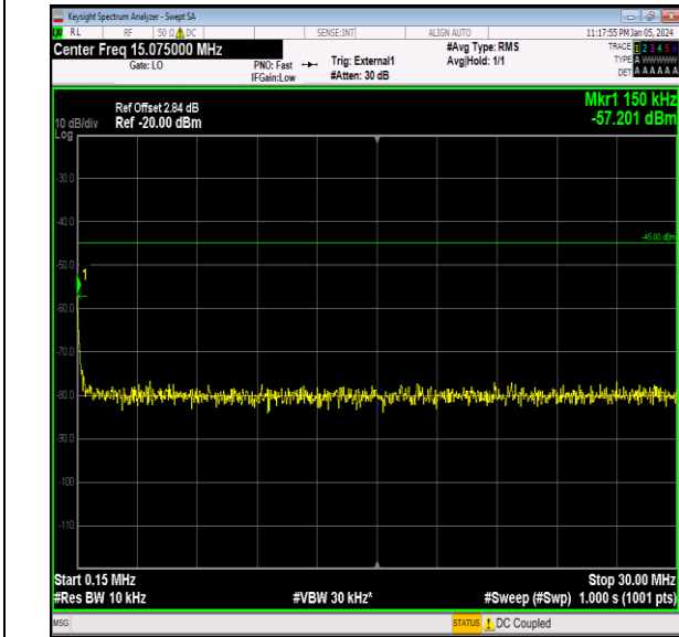
Band41_15MHz_64QAM_41165_1RB#0_0.15~30_0.15~3 0
