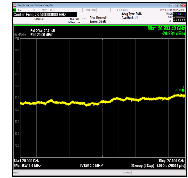
Band41_10MHz_64QAM_40090_1RB#0_20000~27000_20000~27000
