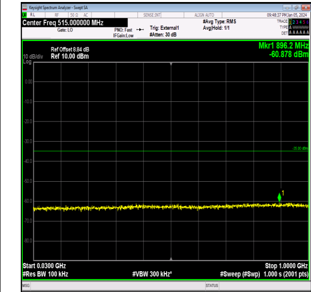
Band41_10MHz_64QAM_40090_1RB#0_30~1000_30~10 00
