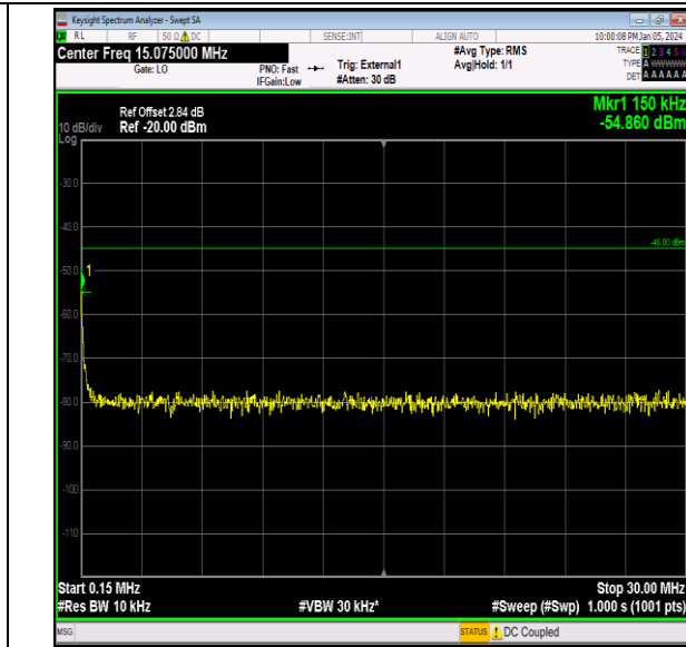
Band41_10MHz_64QAM_41190_1RB#0_0.15~30_0.15~3 0
