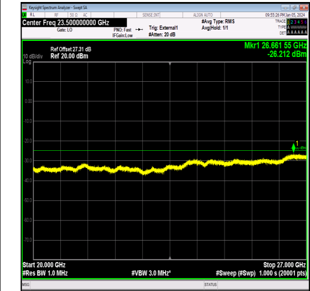
Band41_10MHz_64QAM_40640_1RB#0_20000~27000_2 0000~27000
