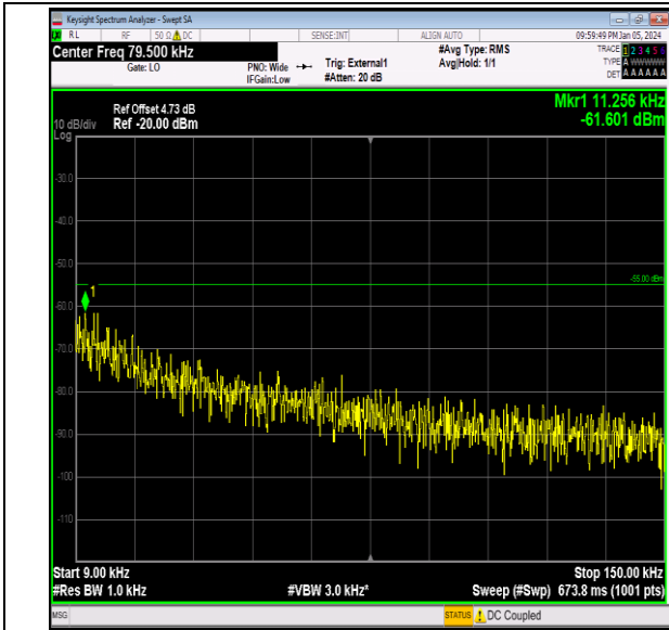
Band41_10MHz_64QAM_41190_1RB#0_0.009~0.15_0.00 9~0.15
