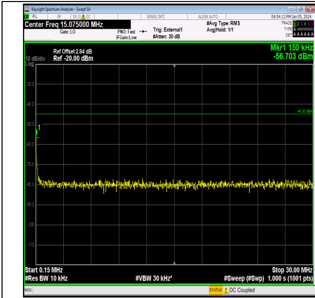
Band41_10MHz_64QAM_40640_1RB#0_0.15~30_0.15~3 0
