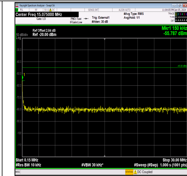
Band41_15MHz_16QAM_40115_1RB#0_0.15~30_0.15~3 0
