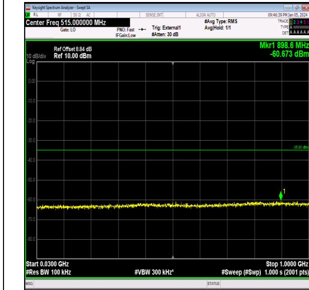
Band41_10MHz_16QAM_40090_1RB#0_30~1000_30~1000
