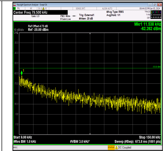
Band41_10MHz_QPSK_40090_1RB#0_0.009~0.15_0.009~0.15
