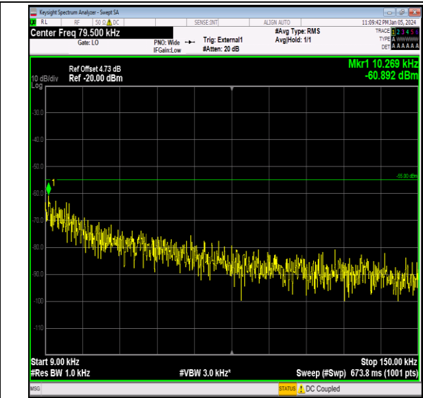
Band41_15MHz_16QAM_40640_1RB#0_0.009~0.15_0.00 9~0.15
