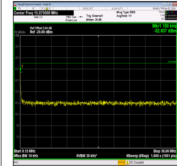
Band41_10MHz_64QAM_40090_1RB#0_0.15~30_0.15~3 0
