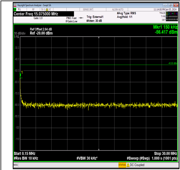
Band41_15MHz_QPSK_41165_1RB#0_0.15~30_0.15~30
