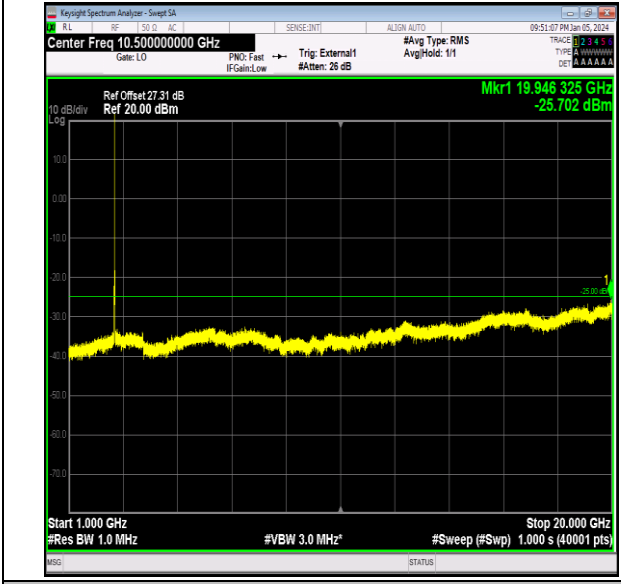
Band41_10MHz_QPSK_40640_1RB#0_1000~20000_100 0~20000
