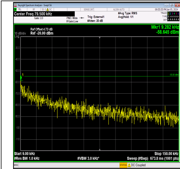
Band41_10MHz_QPSK_41190_1RB#0_0.009~0.15_0.009 ~0.15
