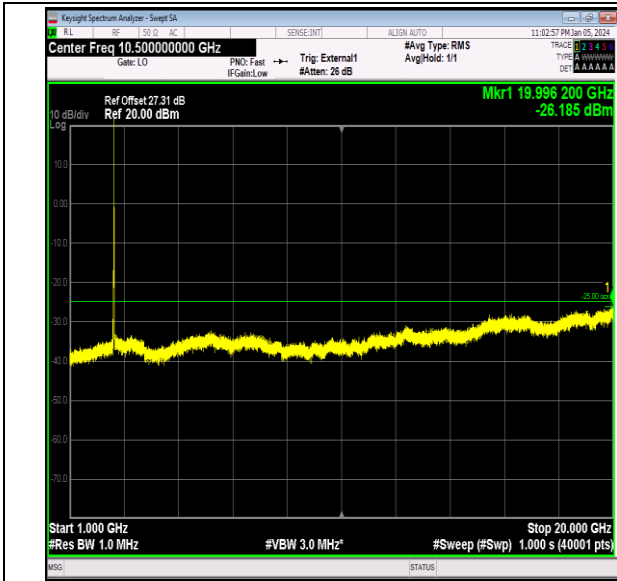
Band41_15MHz_QPSK_40115_1RB#0_1000~20000_100 0~20000
