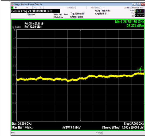
Band41_15MHz_16QAM_40115_1RB#0_20000~27000_2 0000~27000
