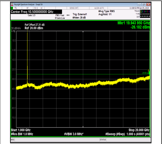
Band41_15MHz_QPSK_40640_1RB#0_1000~20000_100 0~20000
