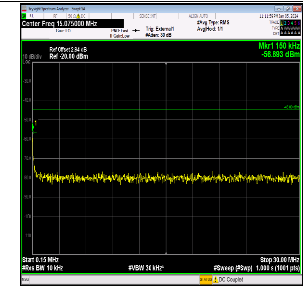
Band41_15MHz_64QAM_40640_1RB#0_0.15~30_0.15~3 0
