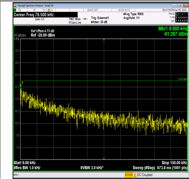
Band41_10MHz_64QAM_40090_1RB#0_0.009~0.15_0.00 9~0.15
