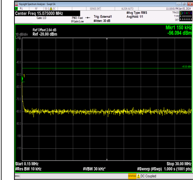
Band41_15MHz_16QAM_40640_1RB#0_0.15~30_0.15~3 0
