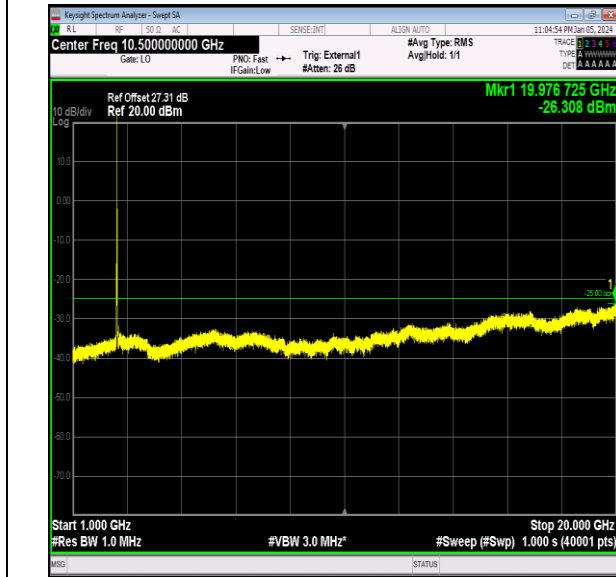
Band41_15MHz_16QAM_40115_1RB#0_1000~20000_10 00~20000
