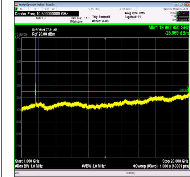
Band41_10MHz_64QAM_40640_1RB#0_1000~20000_10 00~20000
