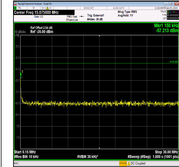
Band41_15MHz_QPSK_40115_1RB#0_0.15~30_0.15~30
