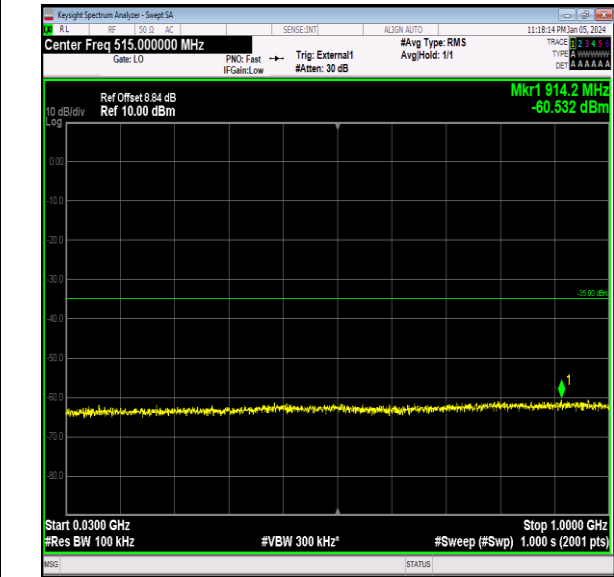
Band41_15MHz_64QAM_41165_1RB#0_30~1000_30~10 00
