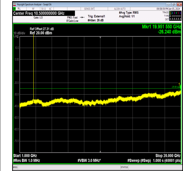
Band41_10MHz_16QAM_41190_1RB#0_1000~20000_10 00~20000
