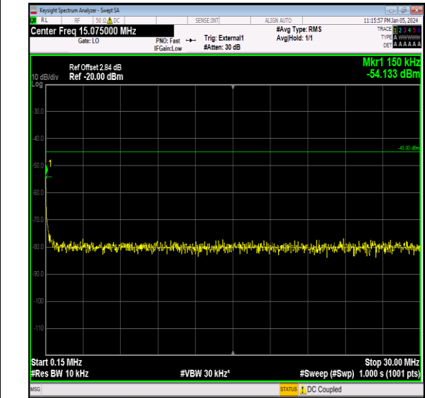
Band41_15MHz_16QAM_41165_1RB#0_0.15~30_0.15~3 0
