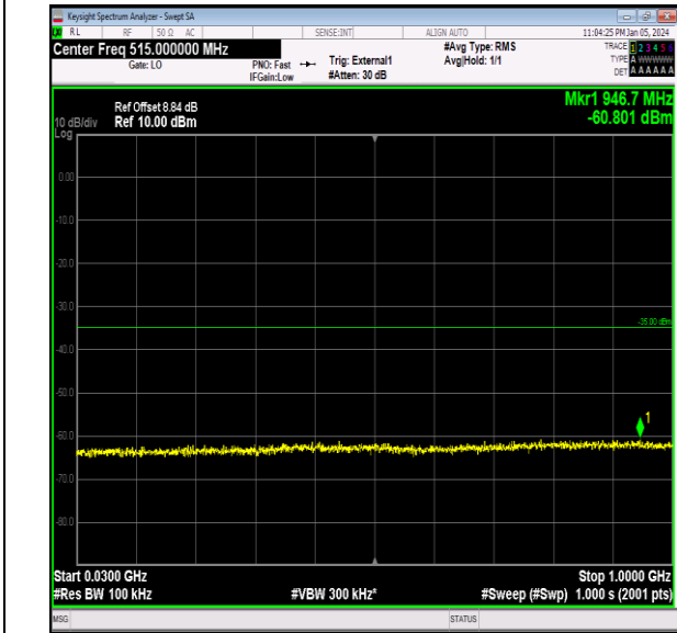
Band41_15MHz_16QAM_40115_1RB#0_30~1000_30~10 00
