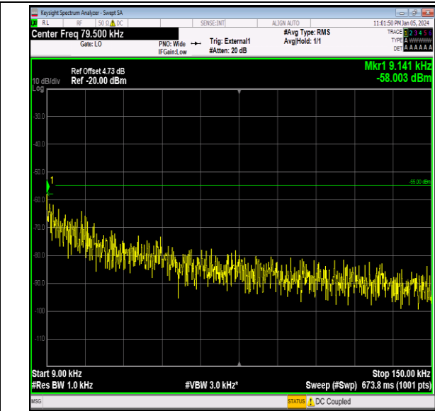
Band41_15MHz_QPSK_40115_1RB#0_0.009~0.15_0.009 ~0.15
