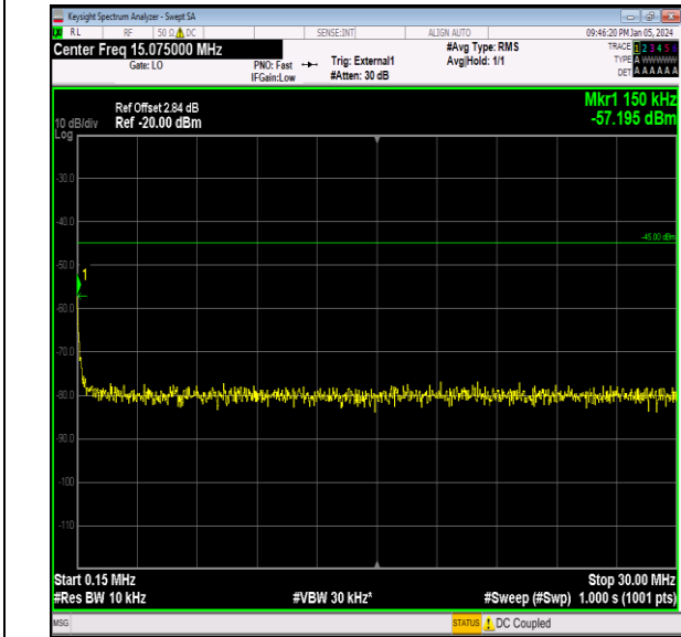
Band41_10MHz_16QAM_40090_1RB#0_0.15~30_0.15~30
