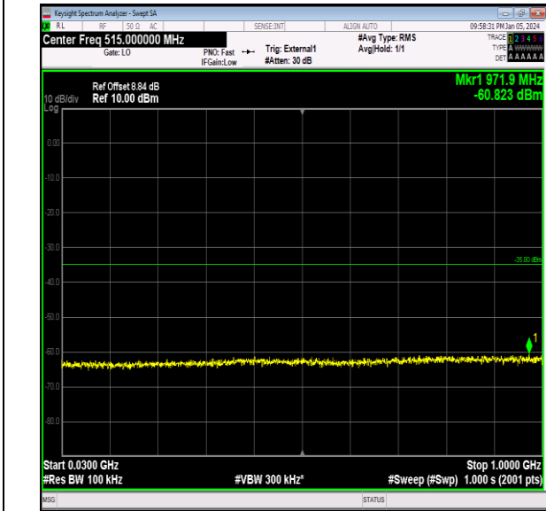
Band41_10MHz_16QAM_41190_1RB#0_30~1000_30~10 00
