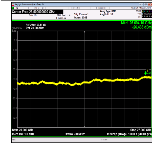
Band41_10MHz_64QAM_41190_1RB#0_20000~27000_2 0000~27000
