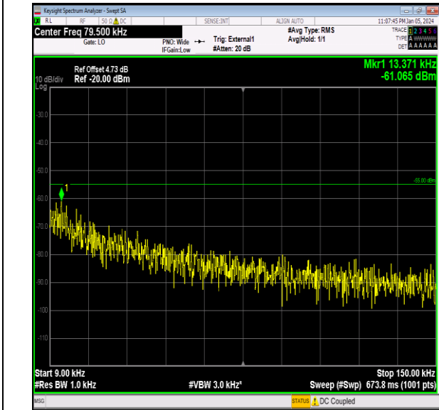
Band41_15MHz_QPSK_40640_1RB#0_0.009~0.15_0.009 ~0.15
