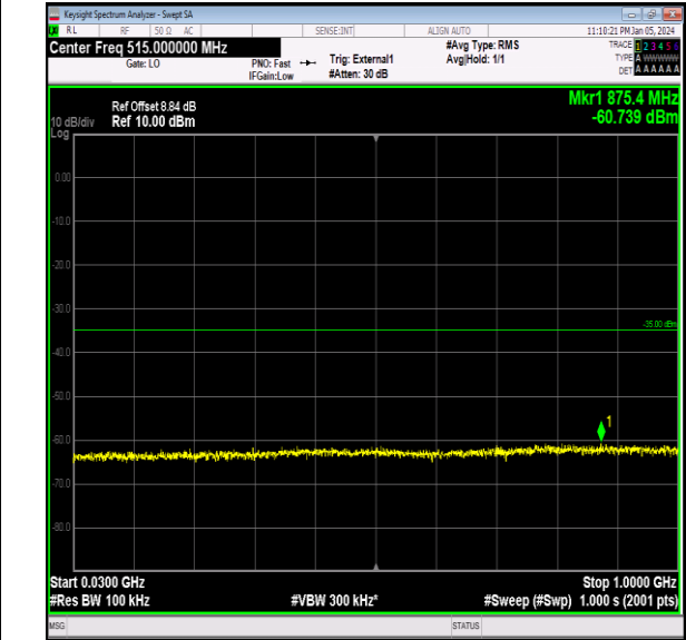
Band41_15MHz_16QAM_40640_1RB#0_30~1000_30~10 00
