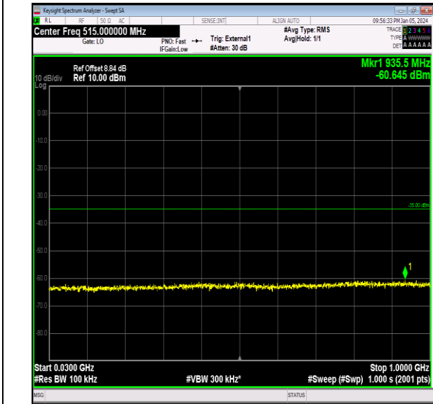
Band41_10MHz_QPSK_41190_1RB#0_30~1000_30~100 0
