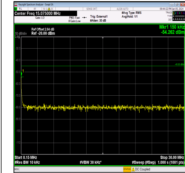
Band41_10MHz_QPSK_40090_1RB#0_0.15~30_0.15~30
