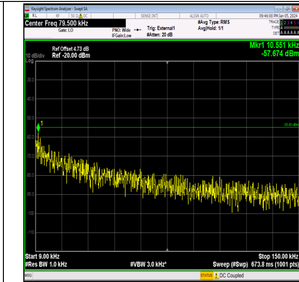
Band41_10MHz_16QAM_40090_1RB#0_0.009~0.15_0.009~0.15
