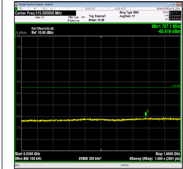
Band41_10MHz_QPSK_40090_1RB#0_30~1000_30~1000
