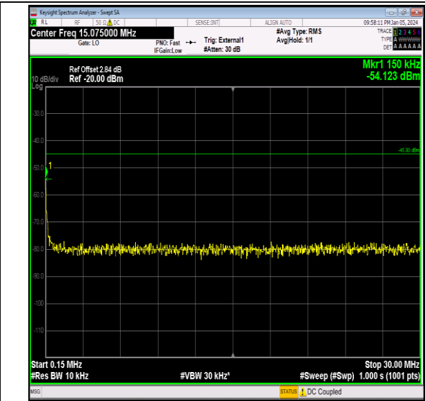
Band41_10MHz_16QAM_41190_1RB#0_0.15~30_0.15~3 0
