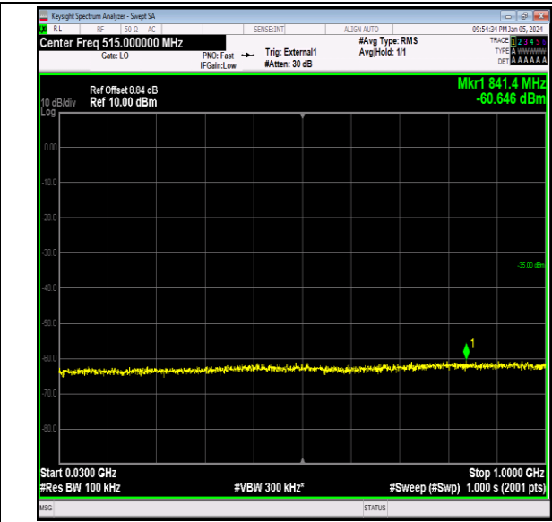
Band41_10MHz_64QAM_40640_1RB#0_30~1000_30~10 00
