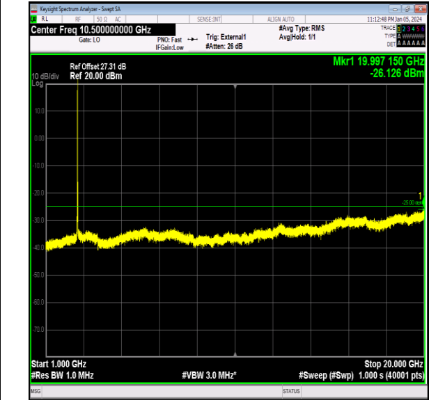
Band41_15MHz_64QAM_40640_1RB#0_1000~20000_10 00~20000
