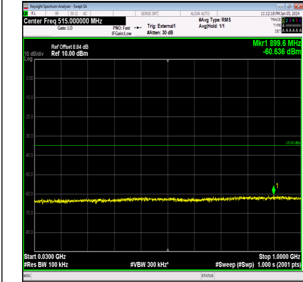
Band41_15MHz_64QAM_40640_1RB#0_30~1000_30~10 00
