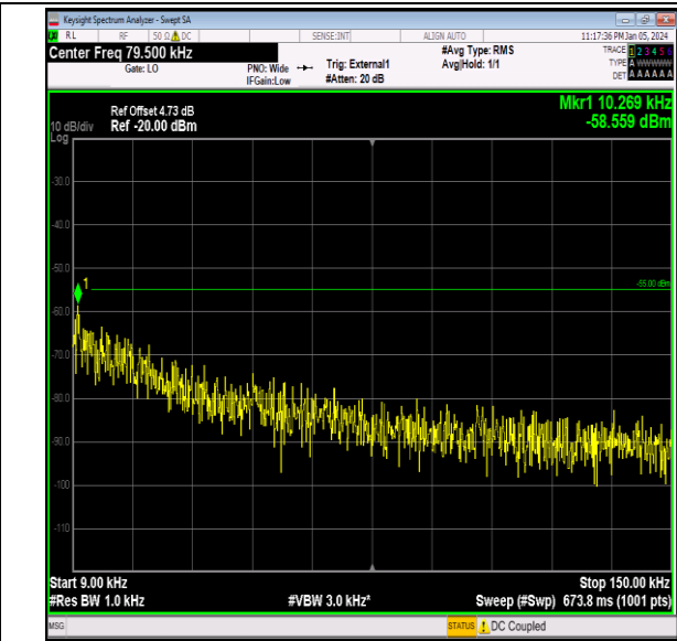
Band41_15MHz_64QAM_41165_1RB#0_0.009~0.15_0.00 9~0.15
