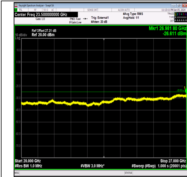
Band41_15MHz_64QAM_40640_1RB#0_20000~27000_2 0000~27000
