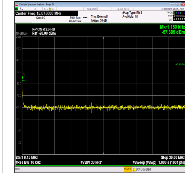
Band41_15MHz_QPSK_40640_1RB#0_0.15~30_0.15~30
