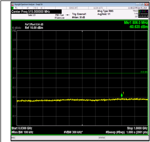
Band41_15MHz_QPSK_40640_1RB#0_30~1000_30~100 0
