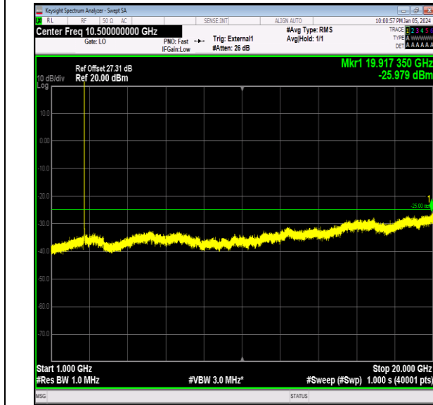
Band41_10MHz_64QAM_41190_1RB#0_1000~20000_10 00~20000
