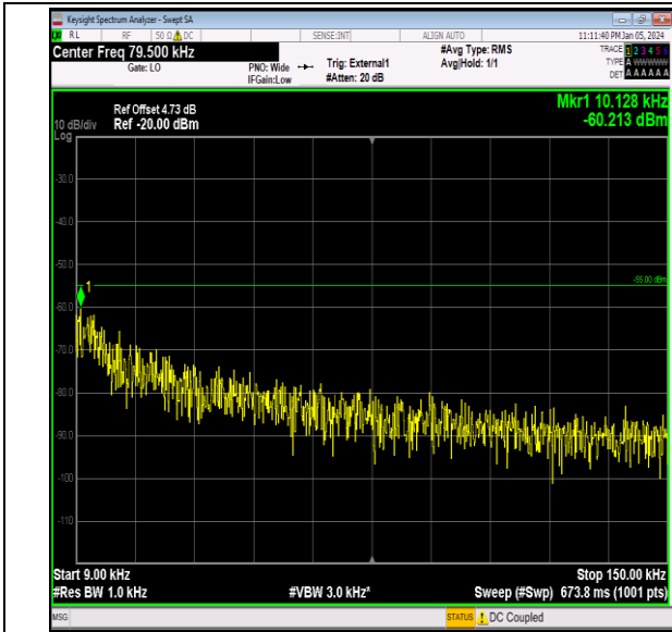
Band41_15MHz_64QAM_40640_1RB#0_0.009~0.15_0.00 9~0.15
