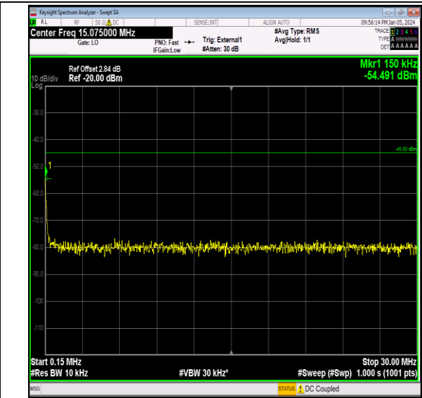
Band41_10MHz_QPSK_41190_1RB#0_0.15~30_0.15~30
