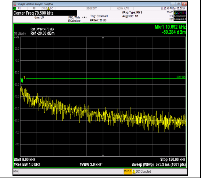
Band41_15MHz_QPSK_41165_1RB#0_0.009~0.15_0.009 ~0.15
