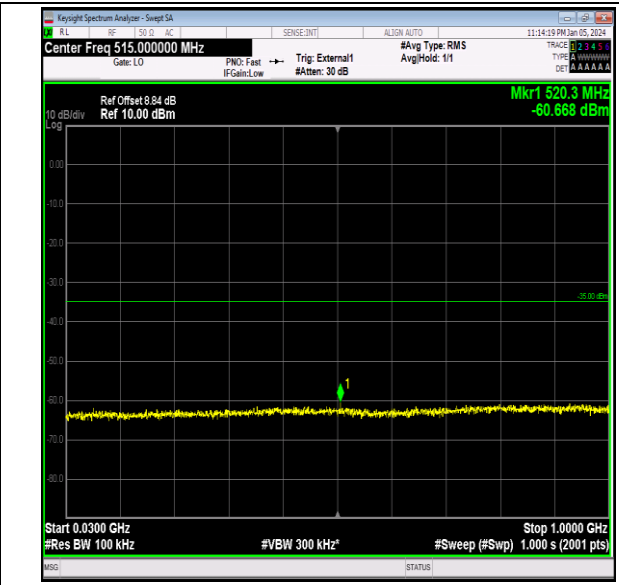
Band41_15MHz_QPSK_41165_1RB#0_30~1000_30~100 0
