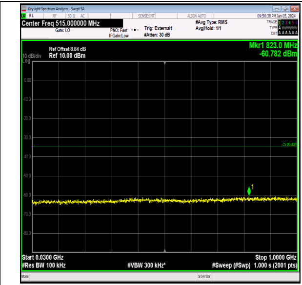
Band41_10MHz_QPSK_40640_1RB#0_30~1000_30~100 0
