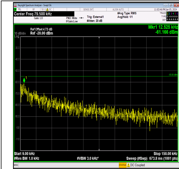
Band41_15MHz_16QAM_40115_1RB#0_0.009~0.15_0.00 9~0.15
