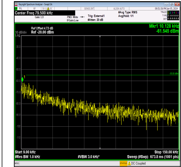
Band41_10MHz_16QAM_40640_1RB#0_0.009~0.15_0.00 9~0.15
