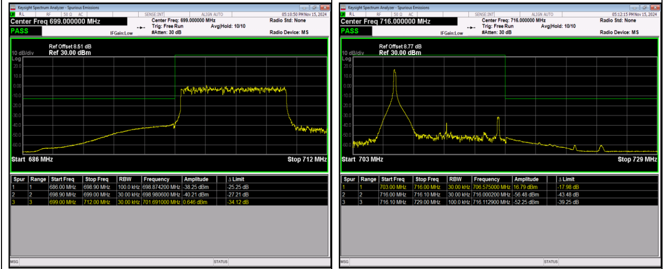
Band12-10MHz-64QAM-23130-1RB#49
