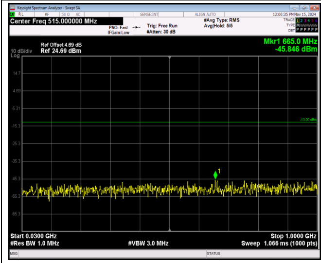
Band4-1.4MHz-QPSK-19957-1RB#0-Range1:30~100 OMHz
