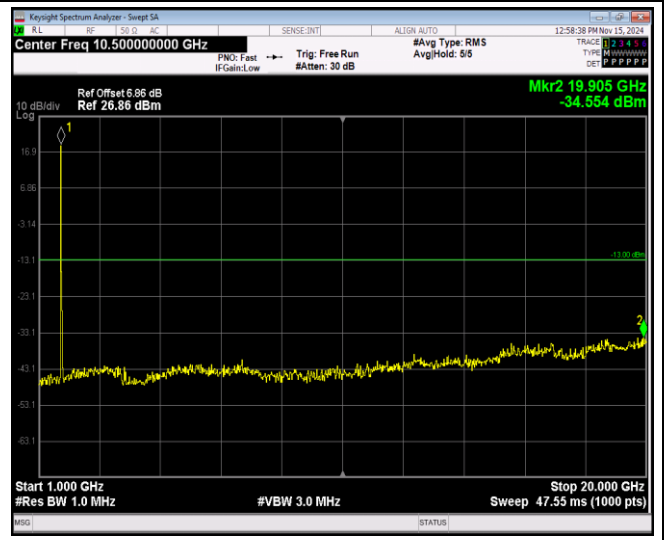
Band4-20MHz-64QAM-20175-1RB#0-Range2:1000~20000MHz
