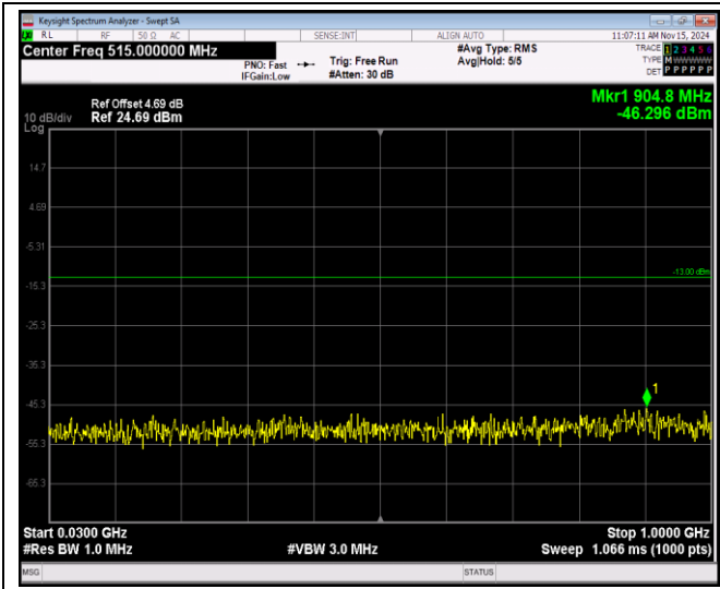
Band2-20MHz-16QAM-18900-1RB#0-Range1:30~1000MHz
