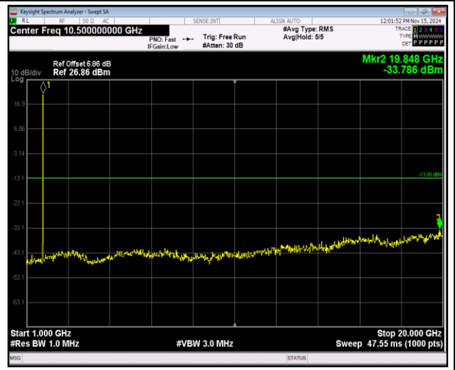
Band4-1.4MHz-64QAM-19957-1RB#0-Range2:1000~20000MHz
