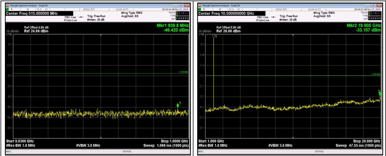
Band2-1.4MHz-16QAM-18607-1RB#0-Range1:30~1000MHz
