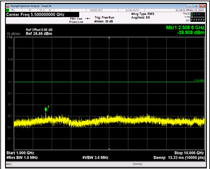
Band5-1.4MHz-QPSK-20643-1RB#0-Range2:1000~10000MHz
