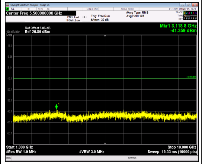
Band5-1.4MHz-16QAM-20407-1RB#0-Range2:1000~10000MHz
