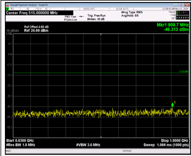
Band4-1.4MHz-QPSK-20175-1RB#0-Range1:30~100 OMHz
