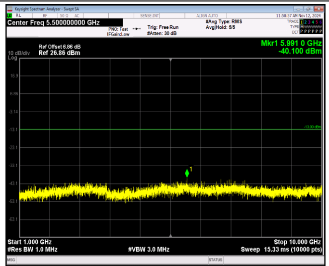
Band5-1.4MHz-64QAM-20643-1RB#0-Range2:1000~10000MHz
