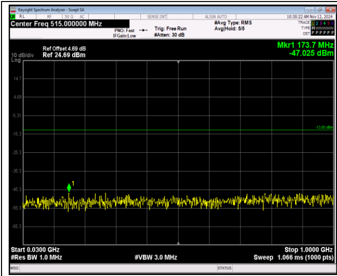
Band4-1.4MHz-16QAM-20393-1RB#0-Range1:30~1000MHz
