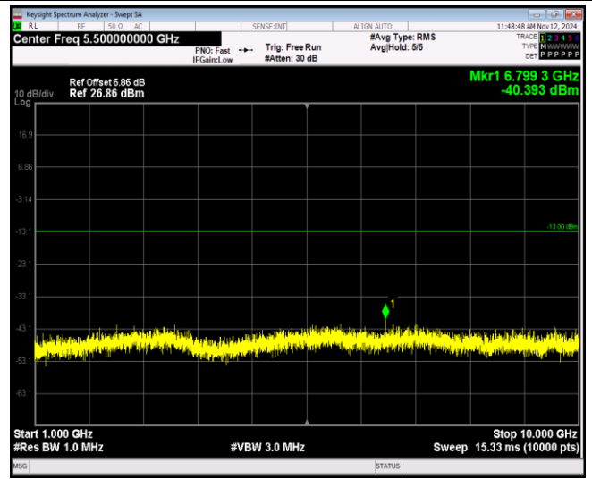
Band5-1.4MHz-16QAM-20407-1RB#0-Range2:1000~ 10000MHz
