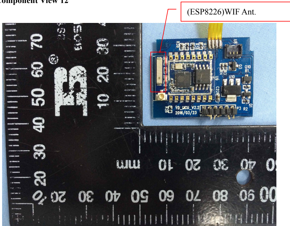
Solder Board-Component View 12
