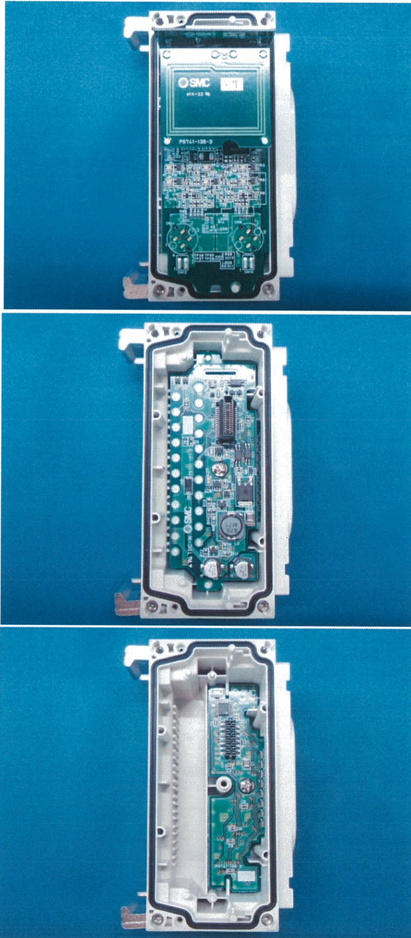
EX600-WSV1 Inside View
