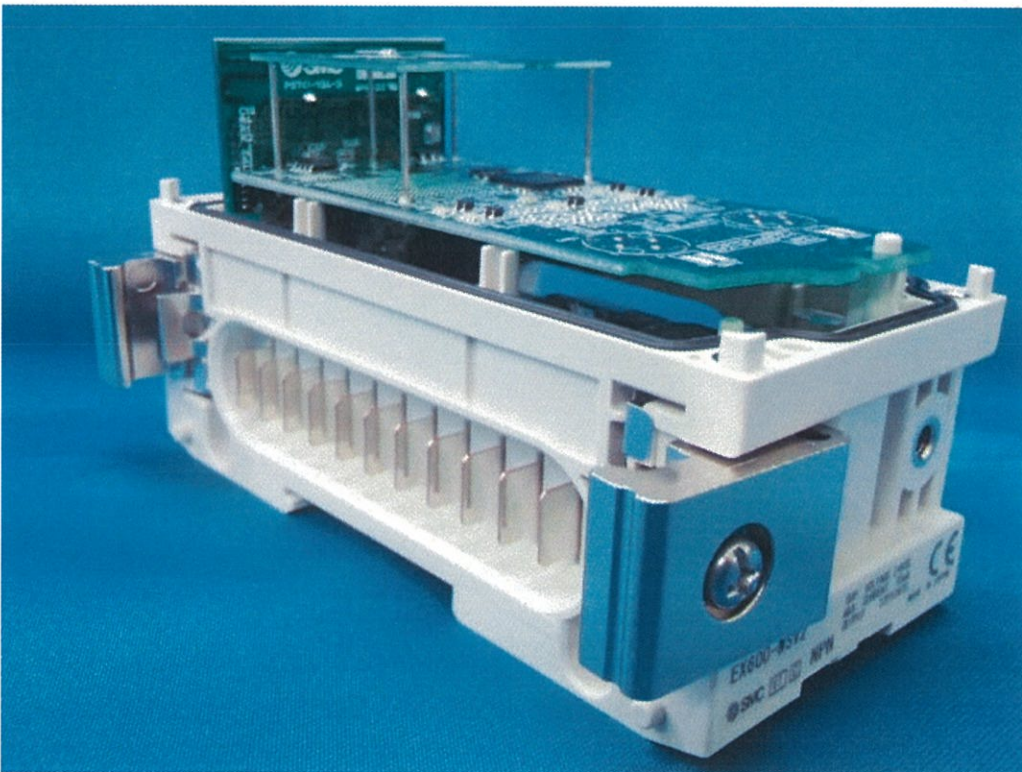
EX600-WSV2 Inside view
