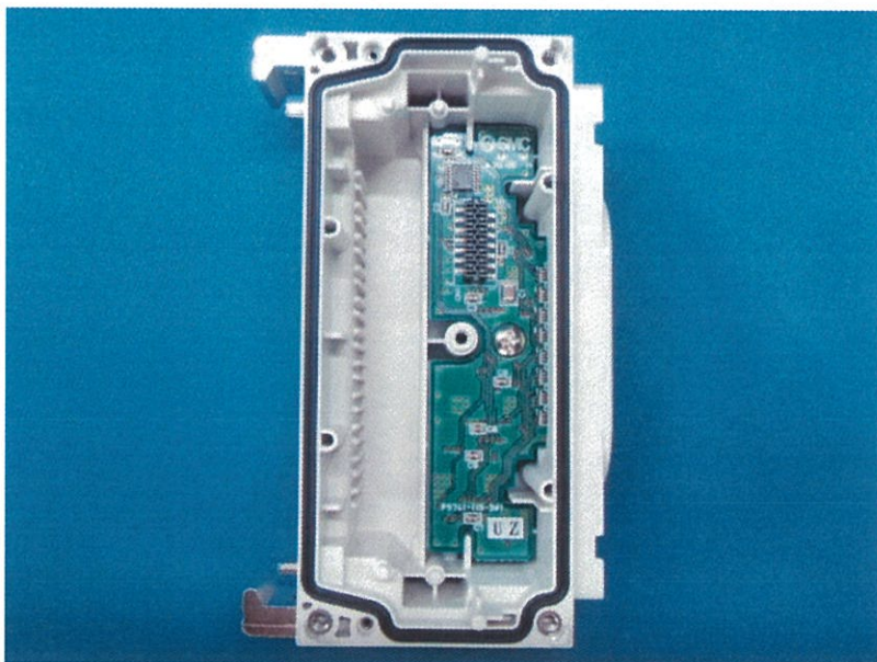
Ex600-WEN2 Inside view
