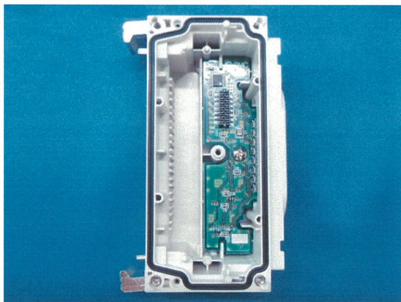
EX600-WEN1 Inside view
