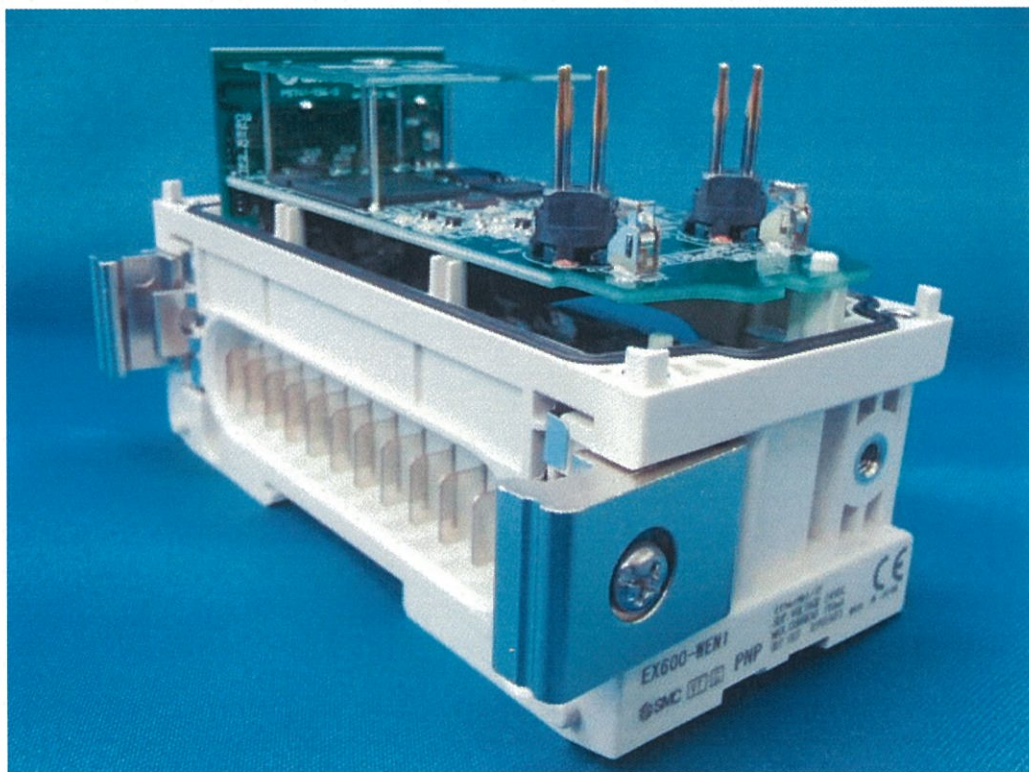
EX600-WEN1 Inside view
