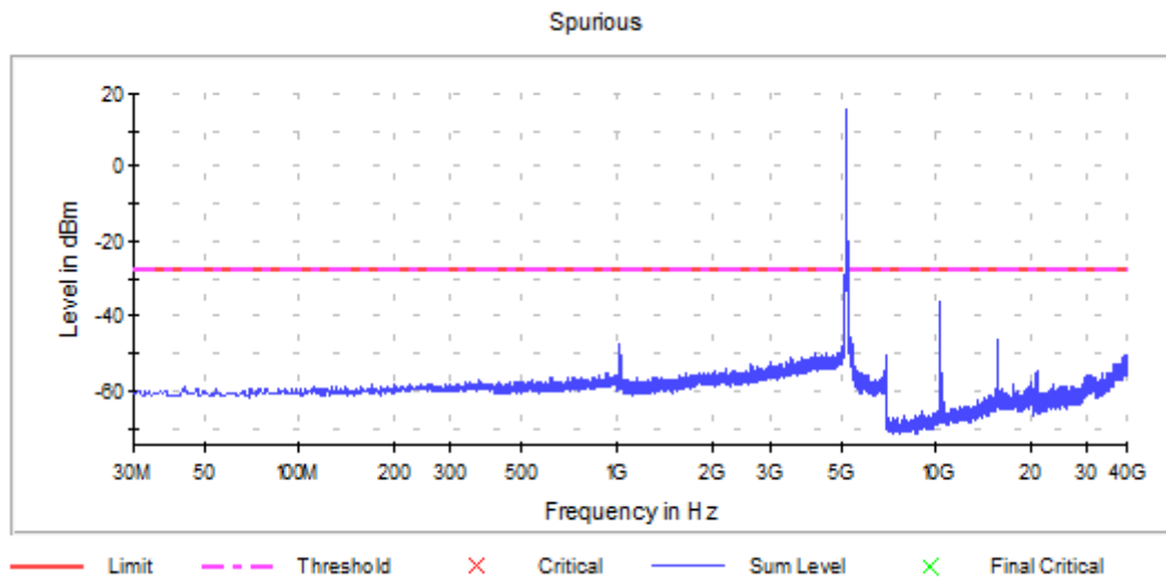
Graph 34: Antenna 0 – Spurious Emissions Channel 44 Transmitting (5220MHz) – Setting 20
