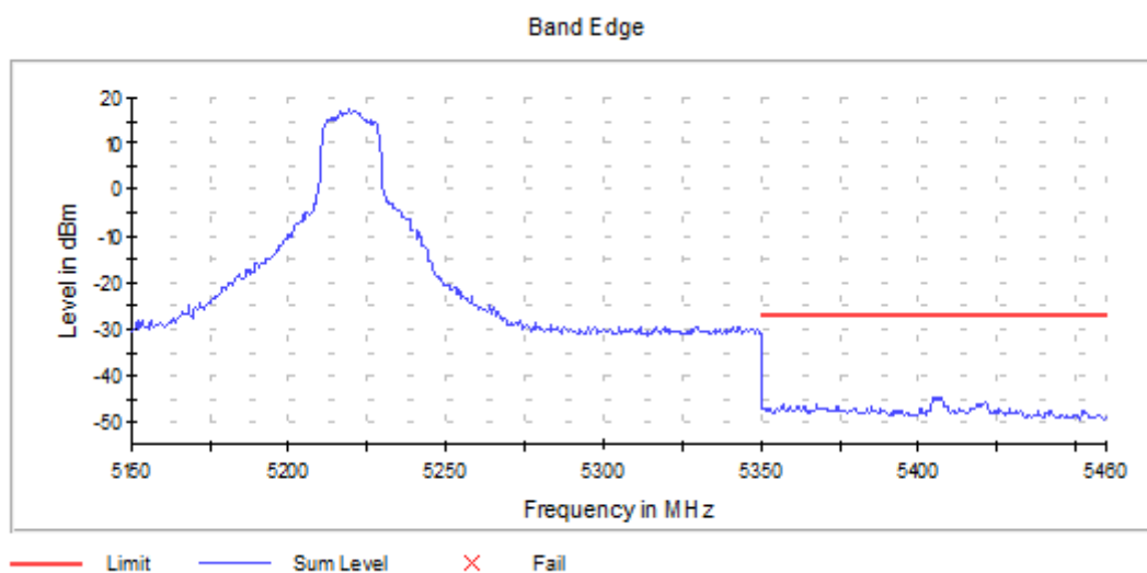
Graph 21: Antenna 0 – Upper Band Edge Channel 44 Transmitting (5220MHz) - Setting 20
