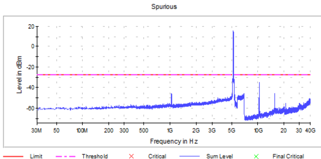
Graph 39: Antenna 1 – Spurious Emissions Channel 48 Transmitting (5240MHz) - Setting 20
