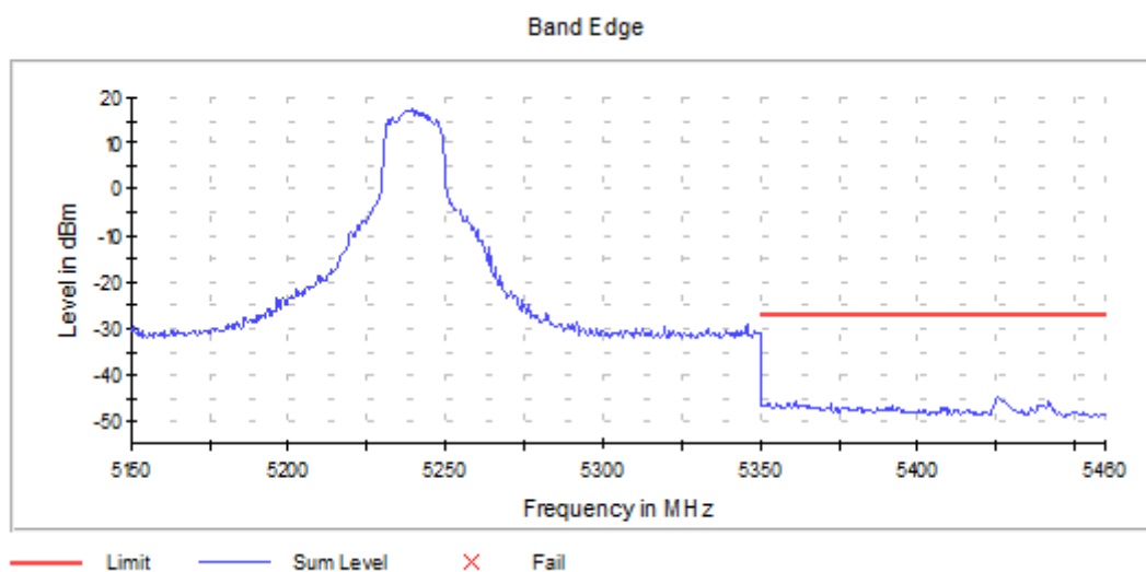
Graph 31: Antenna 1 – Upper Band Edge Channel 48 Transmitting (5240MHz) - Setting 20
