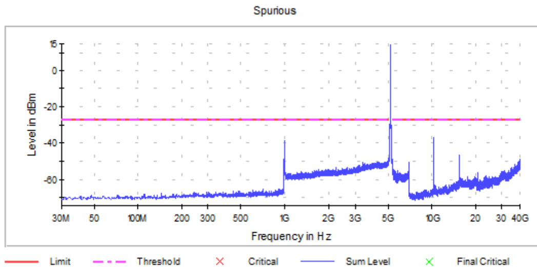
Graph 33: Antenna 0 – Spurious Emissions Channel 40 Transmitting (5200MHz) - Setting 18
