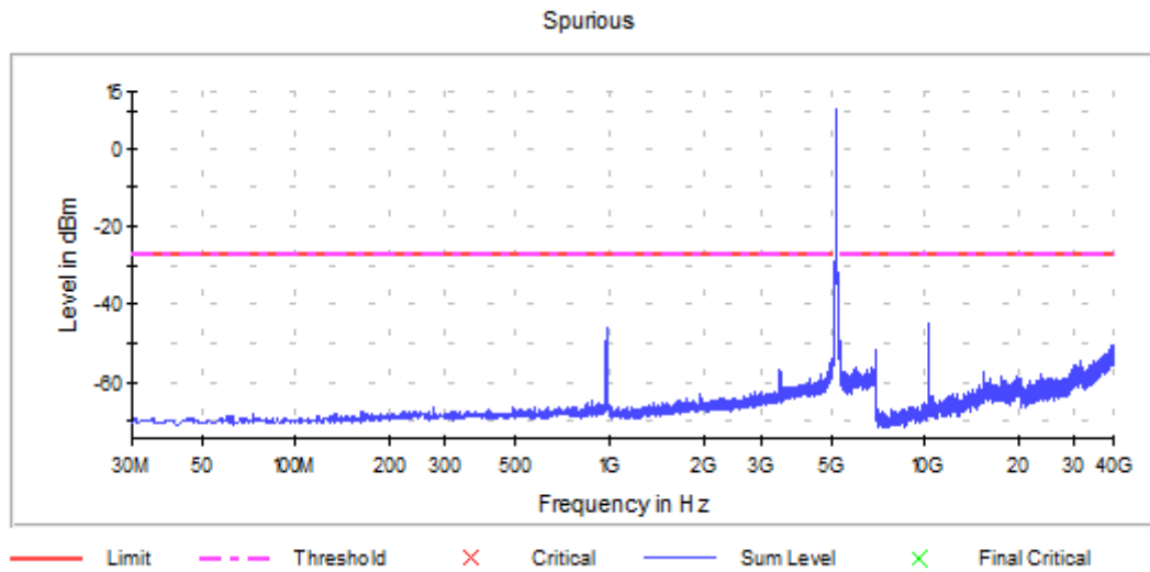
Graph 32: Antenna 0 – Spurious Emissions Channel 36 Transmitting (5180MHz) - Setting 13
