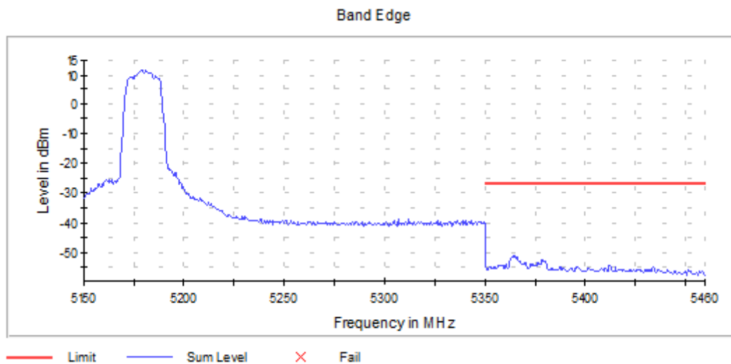
Graph 17: Antenna 0 – Upper Band Edge Channel 36 Transmitting (5180MHz) - Setting 13
