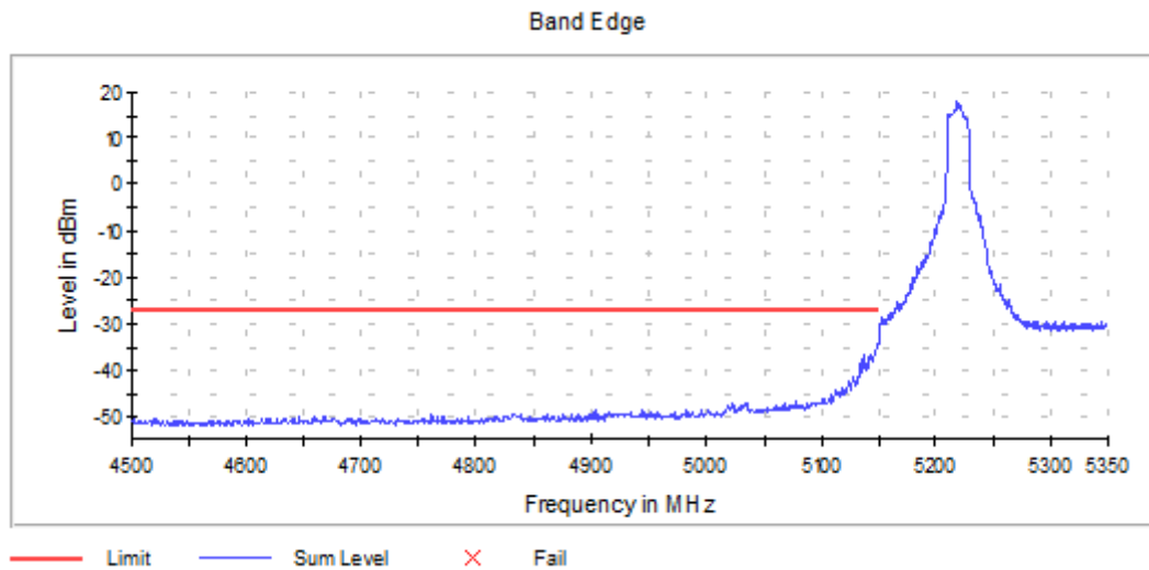
Graph 20: Antenna 0 – Lower Band Edge Channel 44 Transmitting (5220MHz) – Setting 20
