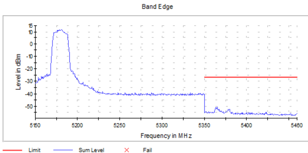
Graph 25: Antenna 1 – Upper Band Edge Channel 36 Transmitting (5180MHz) - Setting 13
