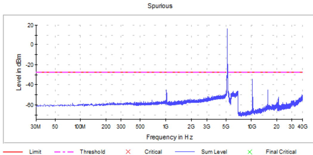
Graph 38: Antenna 1 – Spurious Emissions Channel 44 Transmitting (5220MHz) - Setting 20
