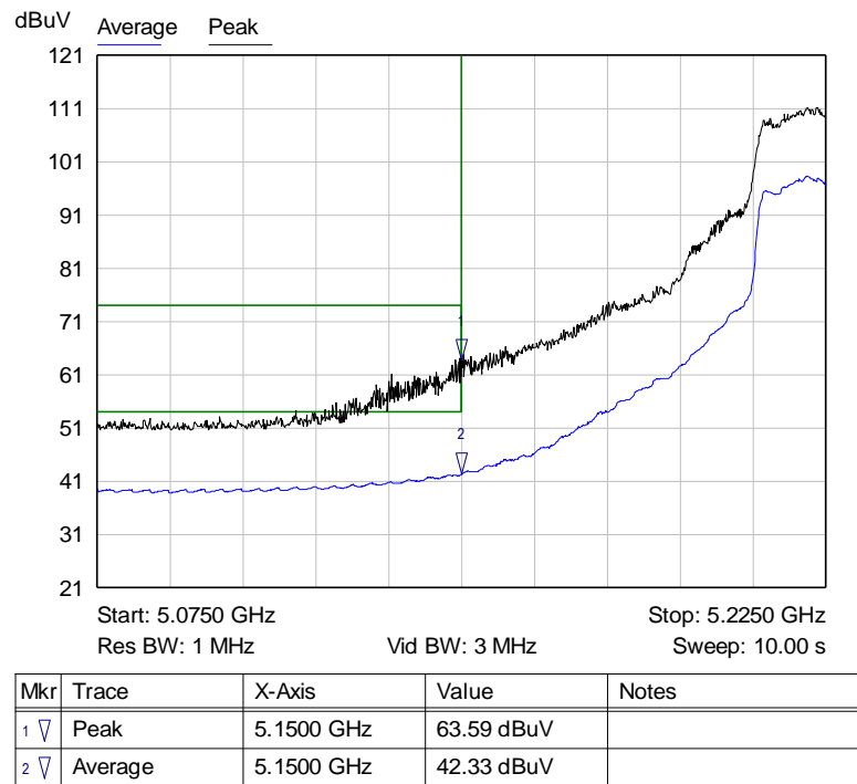
Graph 12:Antenna 0 – Channel 44 Band Edge at the Restricted Band Plot – Setting 20
