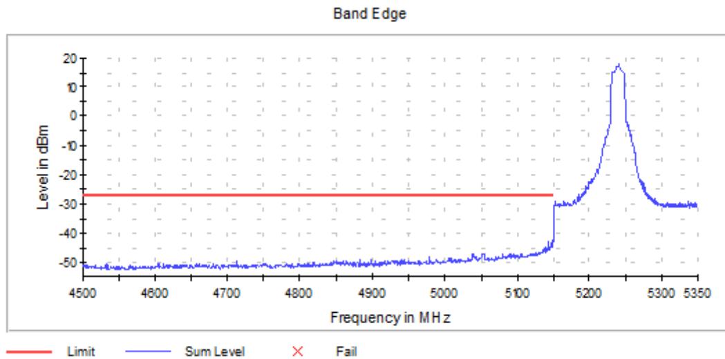
Graph 22: Antenna 0 – Lower Band Edge Channel 48 Transmitting (5240MHz) - Setting 20
