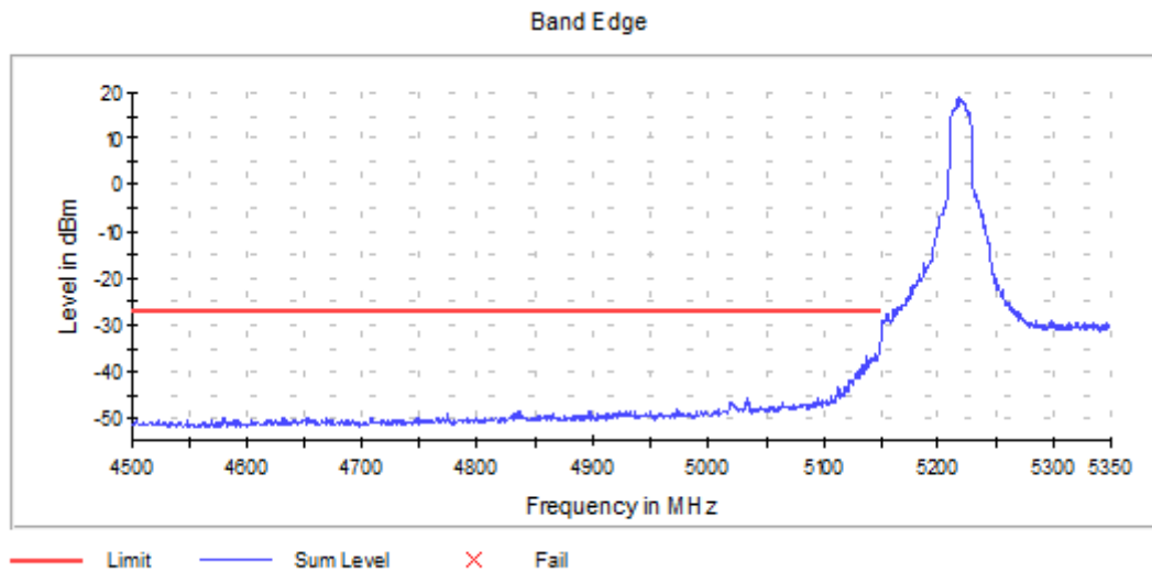
Graph 28: Antenna 1 – Lower Band Edge Channel 44 Transmitting (5220MHz) – Setting 20
