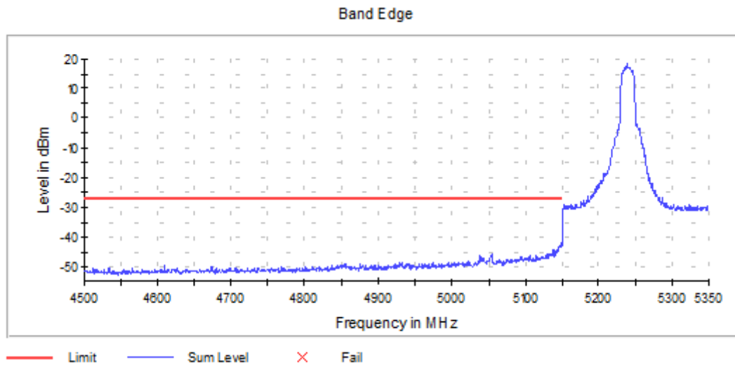
Graph 30: Antenna 1 – Lower Band Edge Channel 48 Transmitting (5240MHz) - Setting 20
