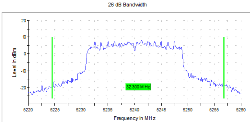
Graph 5: Antenna 0 – 26 dB Emissions Bandwidth Transmitting at 5240 MHz – Setting 20
