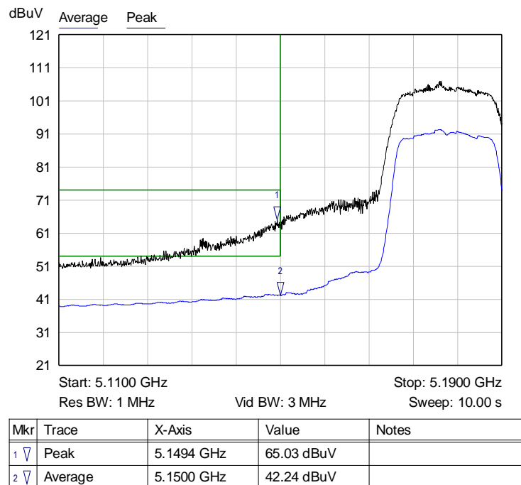
Graph 13: Antenna 1 – Channel 36 Band Edge at the Restricted Band Plot – Setting 13
