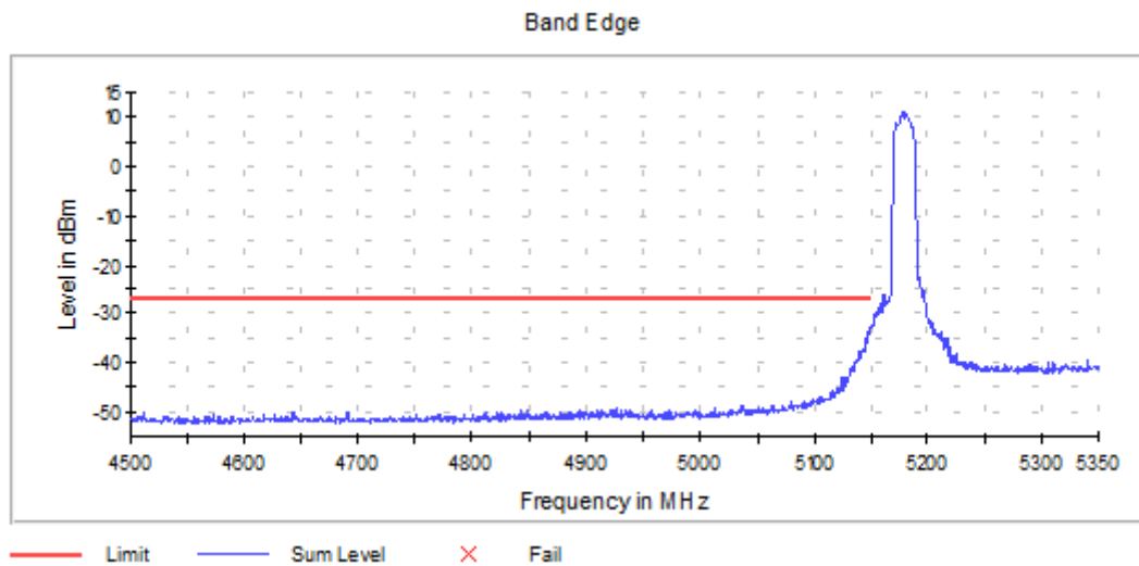
Graph 16: Antenna 0 – Lower Band Edge Channel 36 Transmitting (5180MHz) - Setting 13
