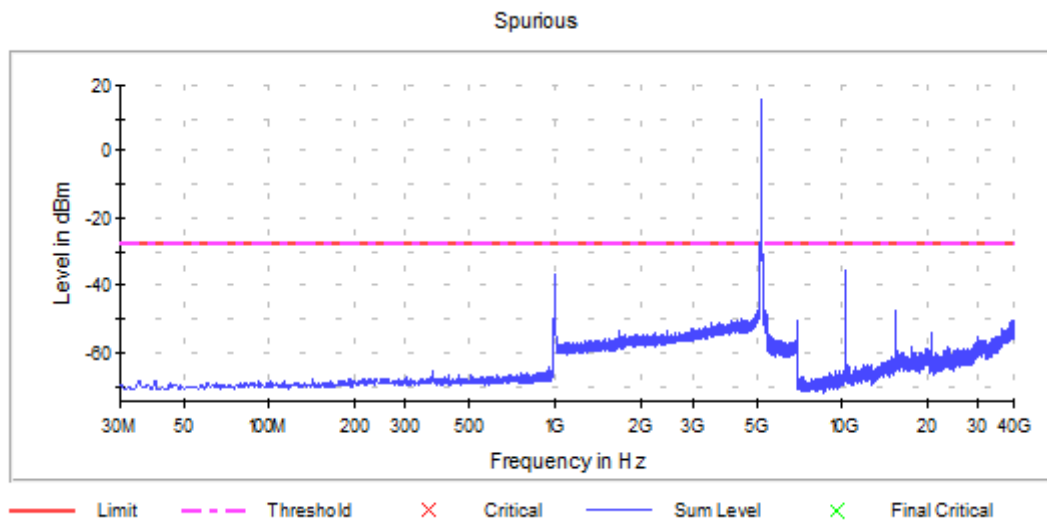
Graph 37: Antenna 1 – Spurious Emissions Channel 40 Transmitting (5200MHz) - Setting 18
