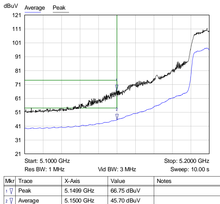
Graph 11: Antenna 0 – Channel 40 Band Edge at the Restricted Band Plot – Setting 18
