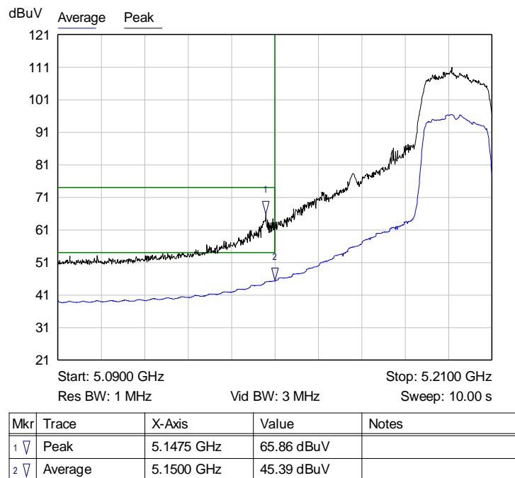
Graph 14: Antenna 1 – Channel 40 Band Edge at the Restricted Band Plot – Setting 18
