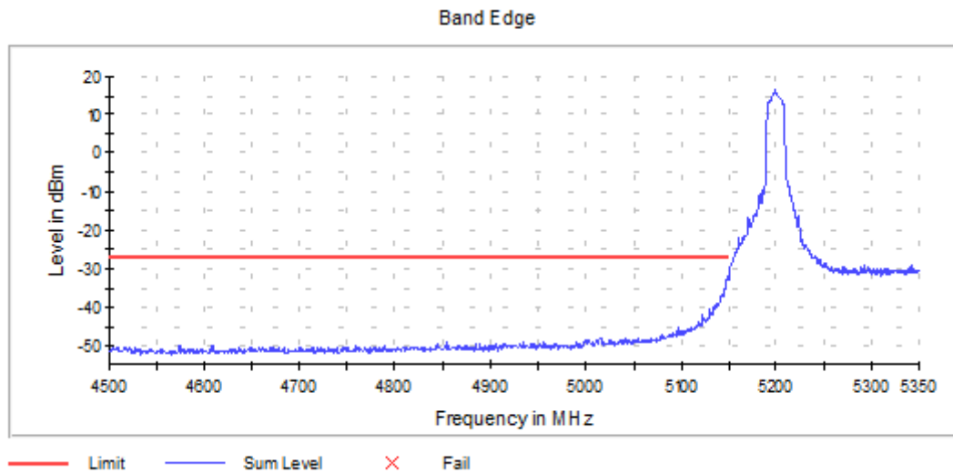
Graph 18: Antenna 0 – Lower Band Edge Channel 40 Transmitting (5200MHz) - Setting 18
