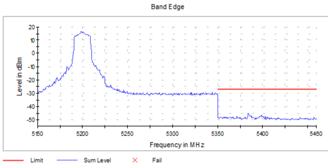
Graph 27: Antenna 1 – Upper Band Edge Channel 40 Transmitting (5200MHz) - Setting 18
