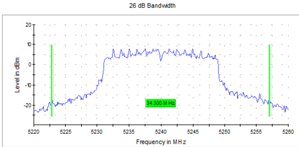
Graph 9: Antenna 1 – 26 dB Emissions Bandwidth Transmitting at 5240 MHz – Setting 20
