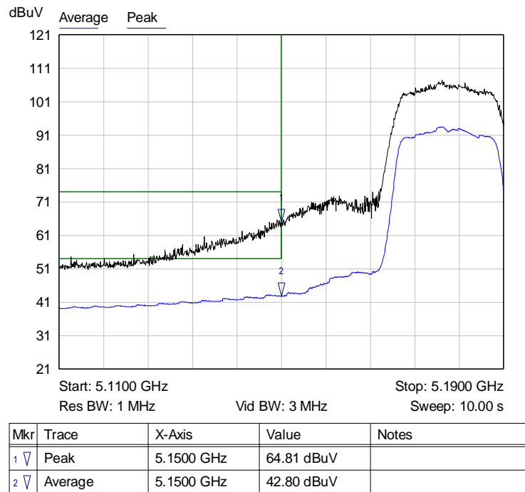
Graph 10: Antenna 0 – Channel 36 Band Edge at the Restricted Band Plot – Setting 13
