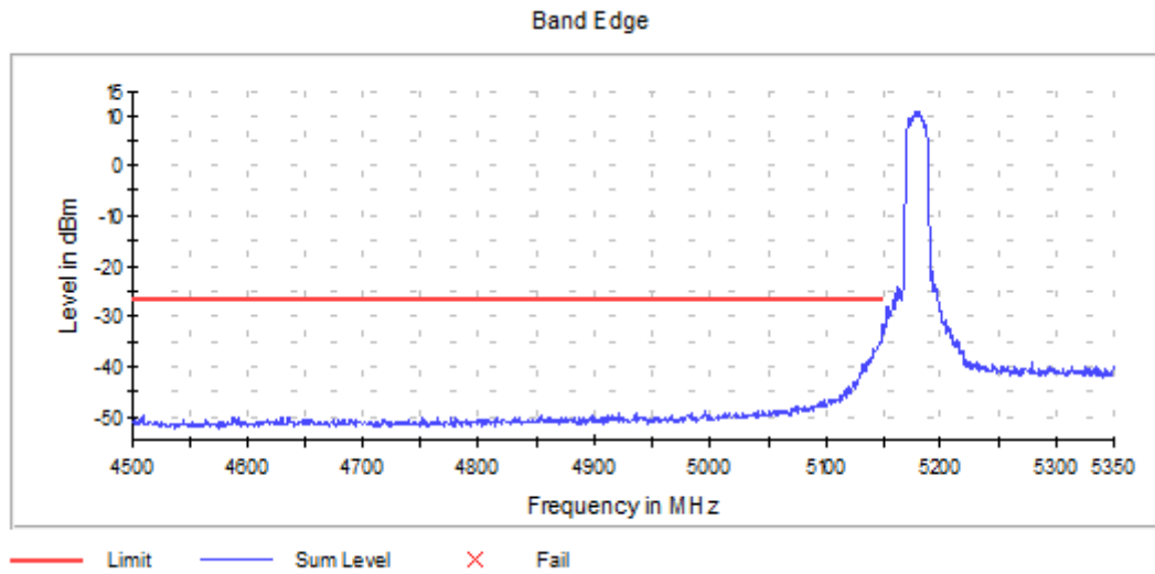
Graph 24: Antenna 1 – Lower Band Edge Channel 36 Transmitting (5180MHz) - Setting 13
