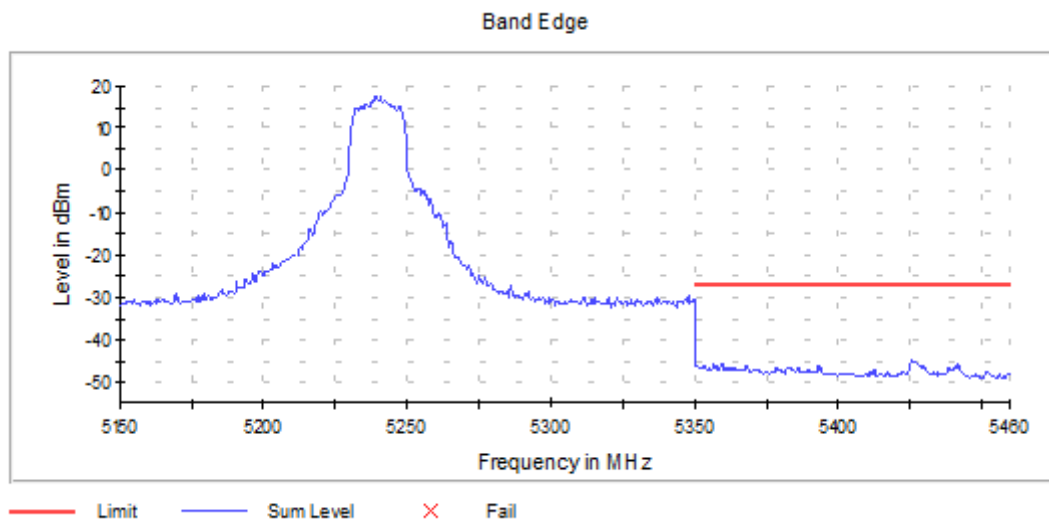
Graph 23: Antenna 0 – Upper Band Edge Channel 48 Transmitting (5240MHz) - Setting 20
