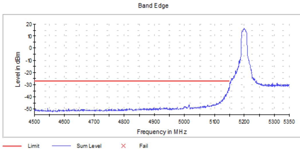
Graph 26: Antenna 1 – Lower Band Edge Channel 40 Transmitting (5200MHz) - Setting 18
