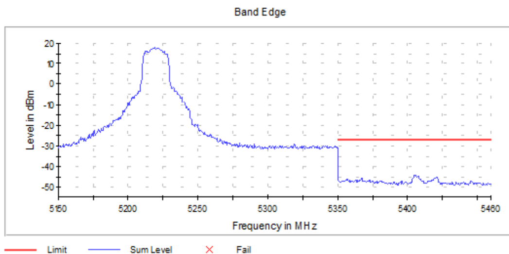
Graph 29: Antenna 1 – Upper Band Edge Channel 44 Transmitting (5220MHz) - Setting 20
