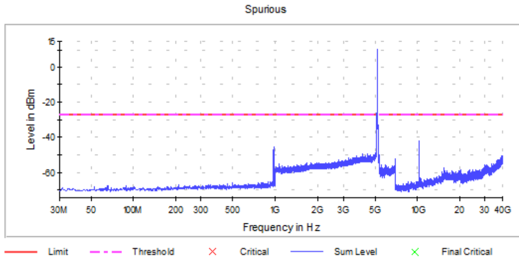
Graph 36: Antenna 1 – Spurious Emissions Channel 36 Transmitting (5180MHz) - Setting 13
