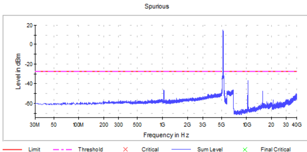
Graph 35: Antenna 0 – Spurious Emissions Channel 48 Transmitting (5240MHz) - Setting 20
