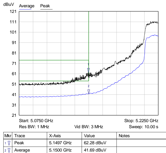
Graph 15: Antenna 1 – Channel 44 Band Edge at the Restricted Band Plot – Setting 20
