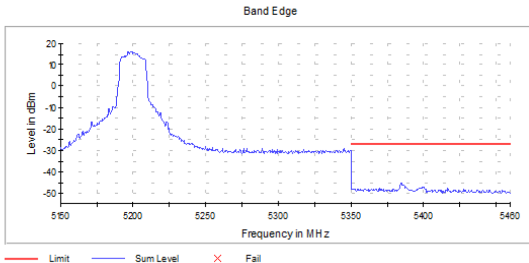
Graph 19: Antenna 0 – Upper Band Edge Channel 40 Transmitting (5200MHz) - Setting 18
