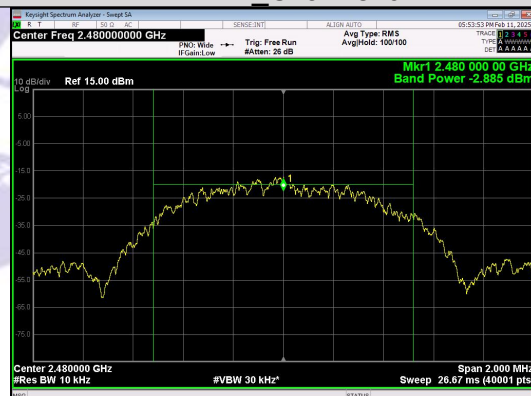
Average Output Power BLE 1M_Channel 39
