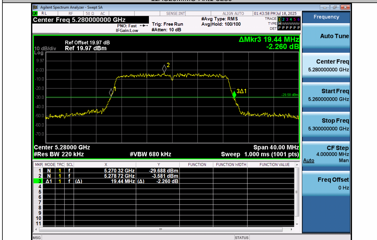
11AC20MIMO-Ant2-5280
