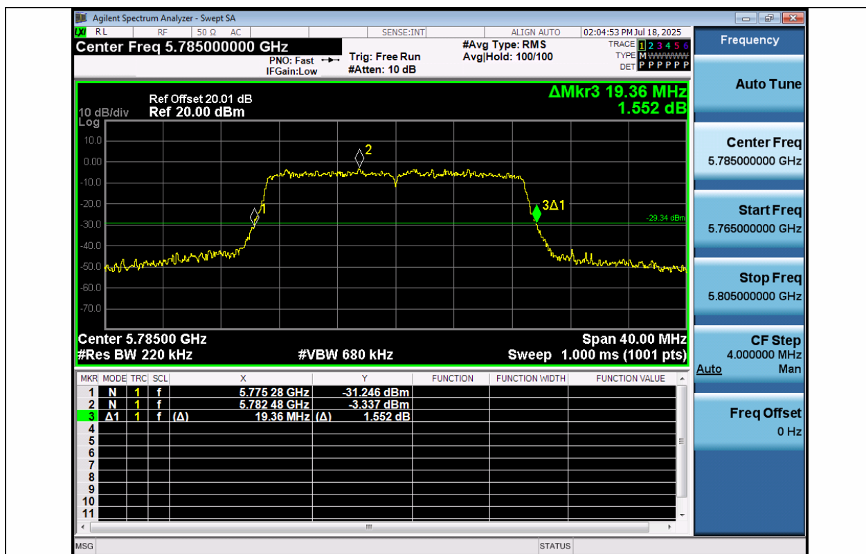
11AC20MIMO-Ant1-5785
