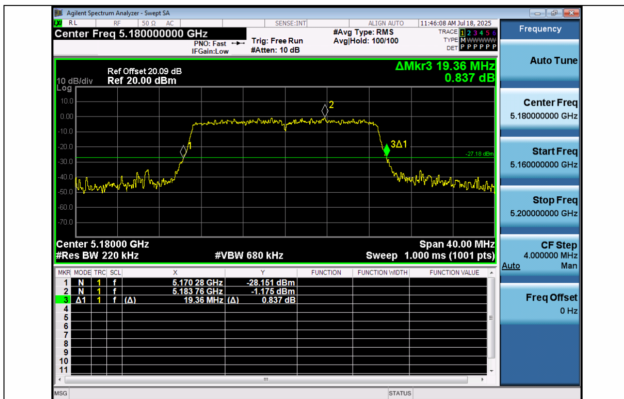
11AC20MIMO-Ant1-5180
