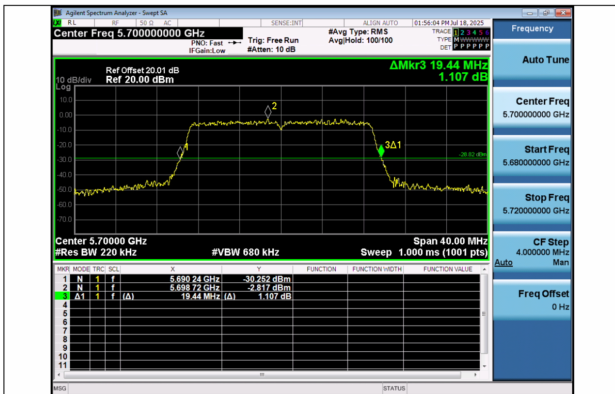
11AC20MIMO-Ant1-5700
