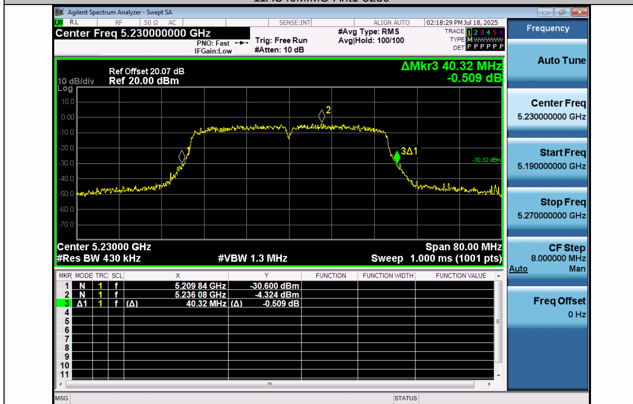
11AC40MIMO-Ant2-5230
