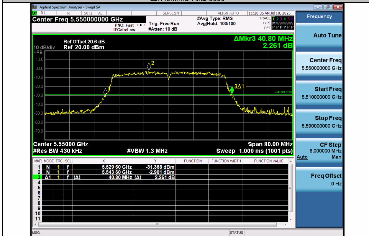
11N40MIMO-Ant2-5550
