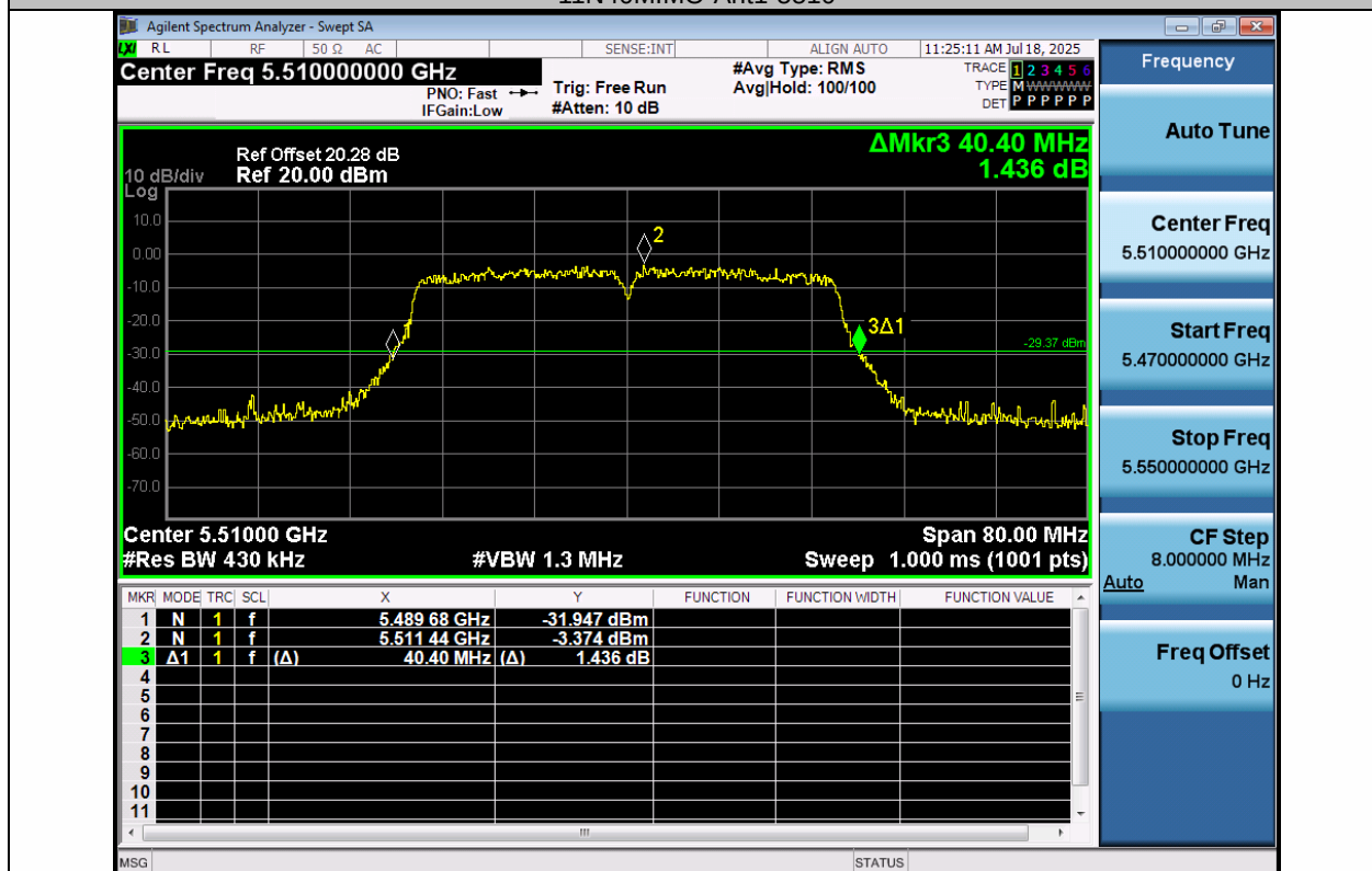
11N40MIMO-Ant2-5510
