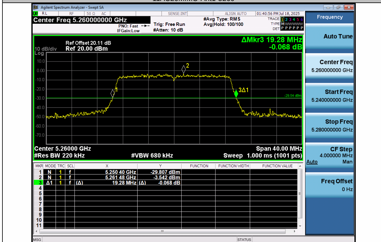
11AC20MIMO-Ant2-5260
