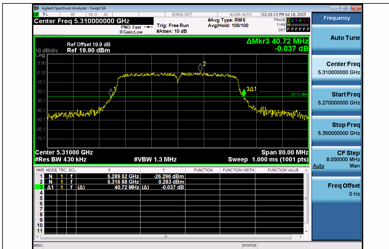
11AC40MIMO-Ant1-5310
