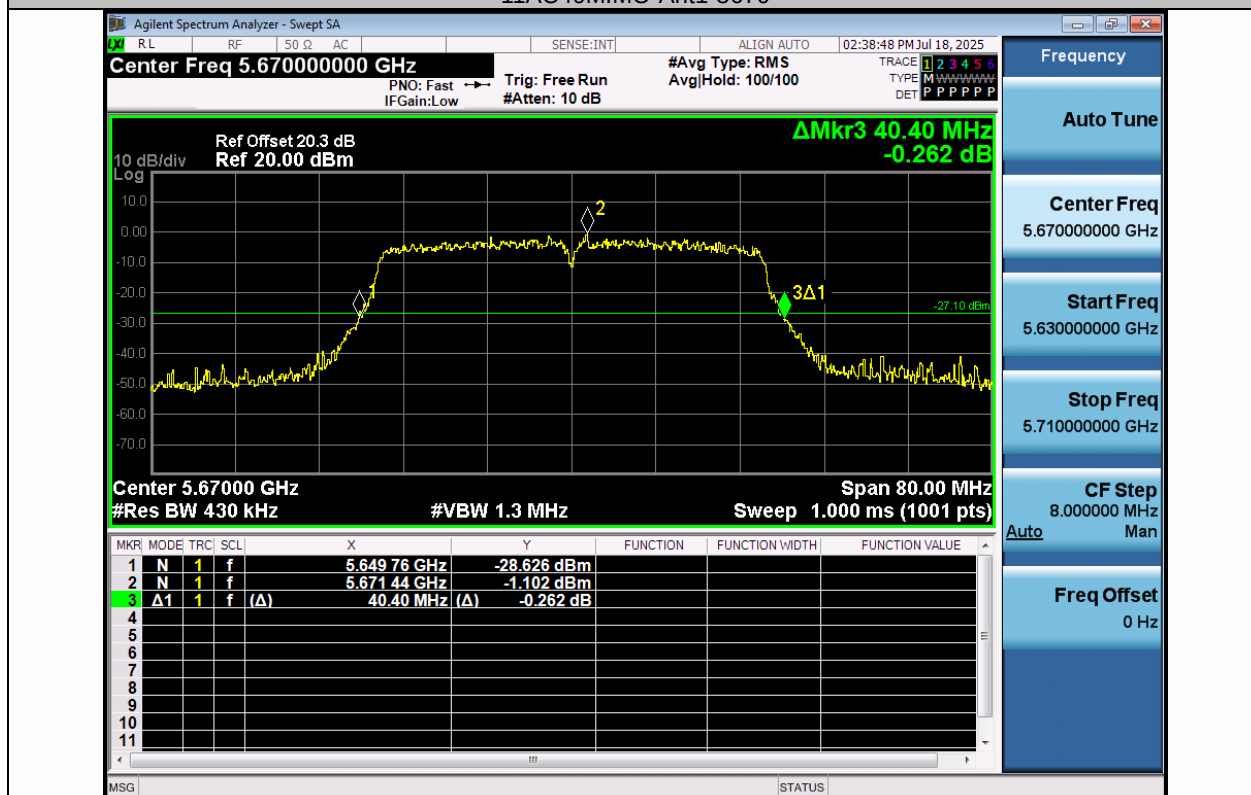
11AC40MIMO-Ant2-5670
