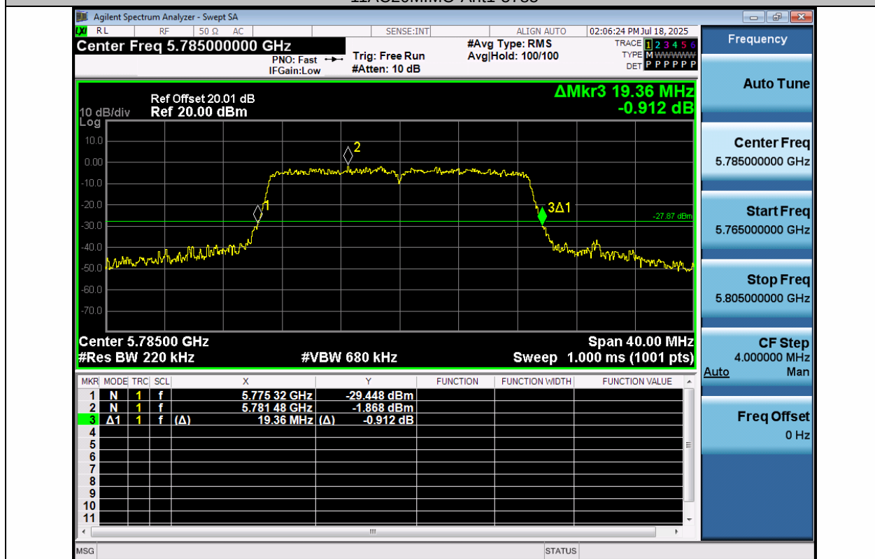
11AC20MIMO-Ant2-5785
