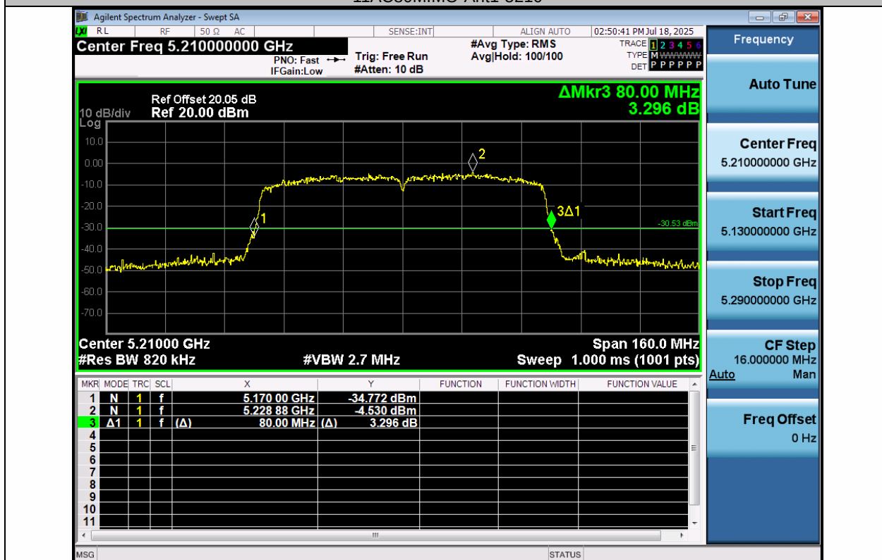
11AC80MIMO-Ant2-5210
