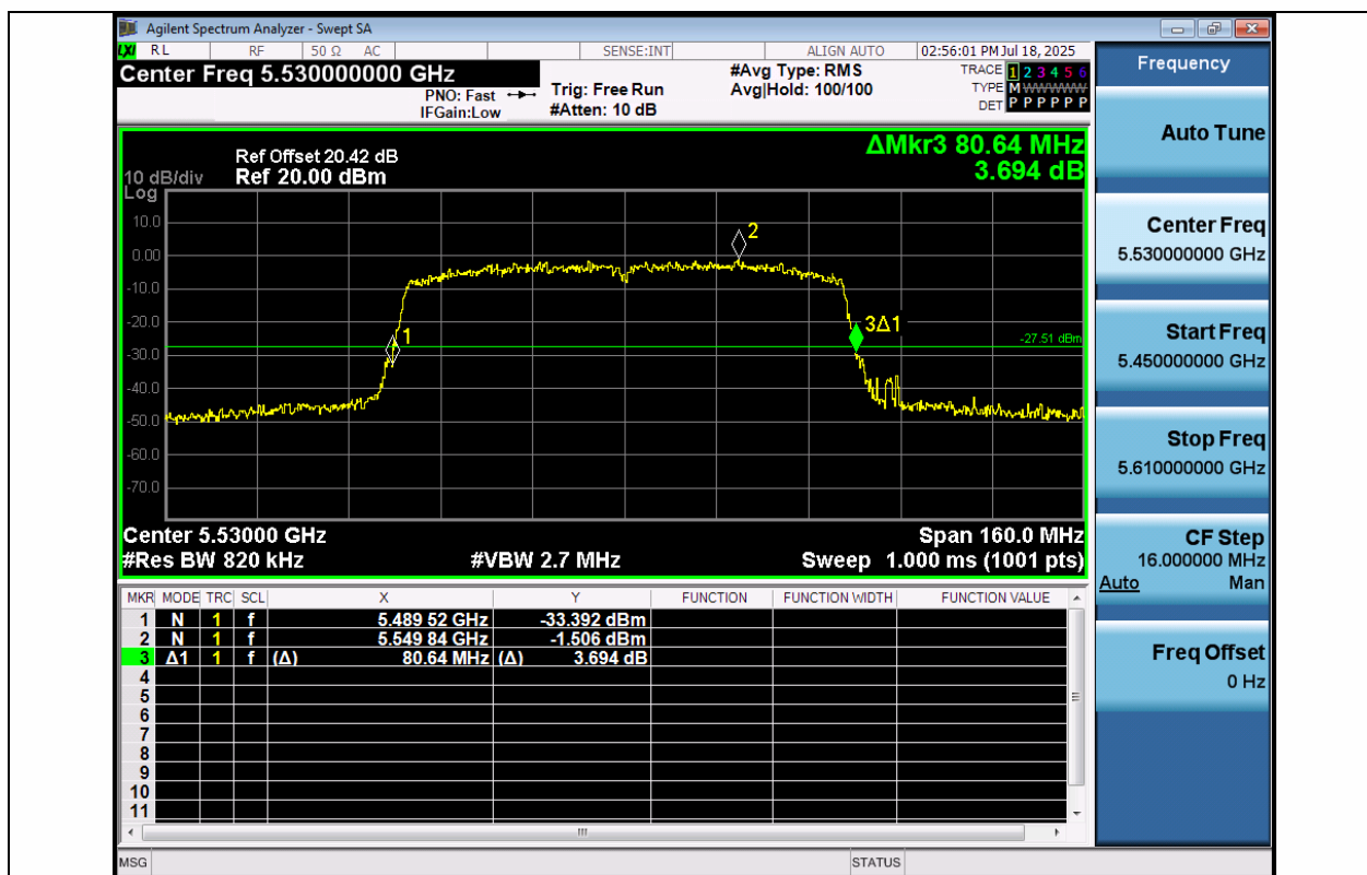
11AC80MIMO-Ant1-5530
