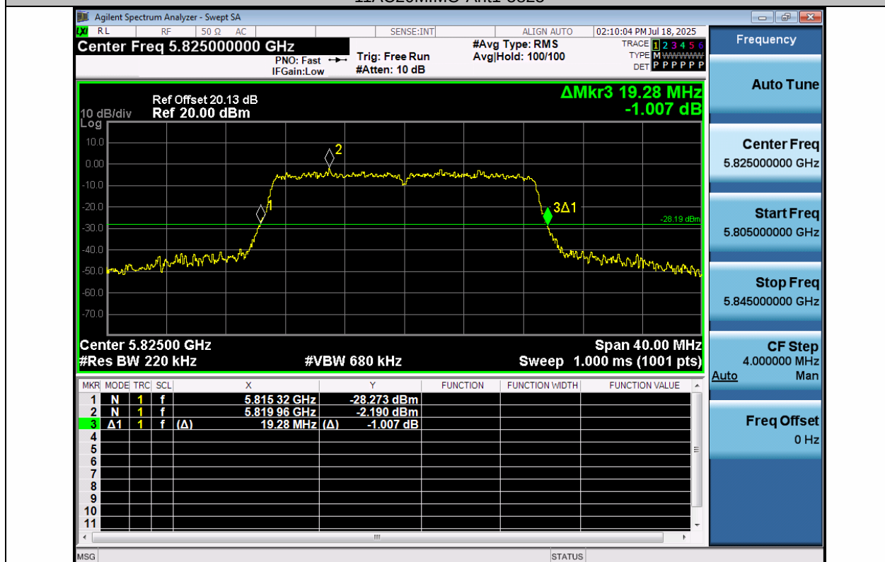
11AC20MIMO-Ant2-5825
