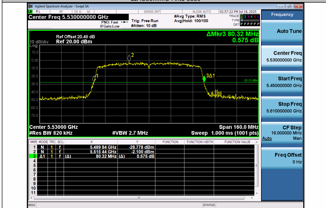
11AC80MIMO-Ant2-5530
