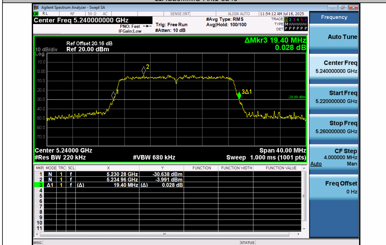
11AC20MIMO-Ant2-5240
