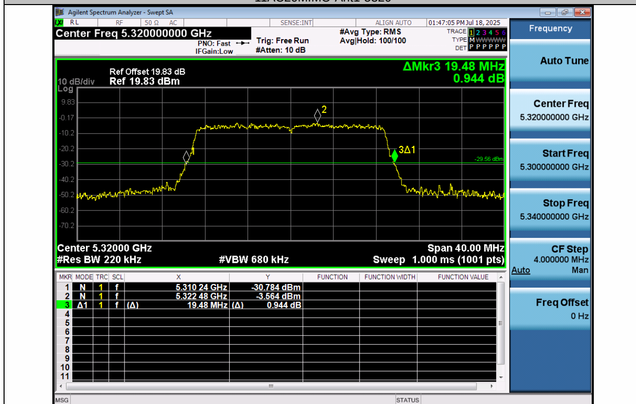
11AC20MIMO-Ant2-5320
