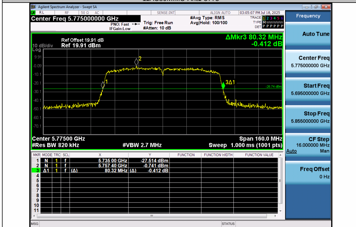
11AC80MIMO-Ant2-5775
