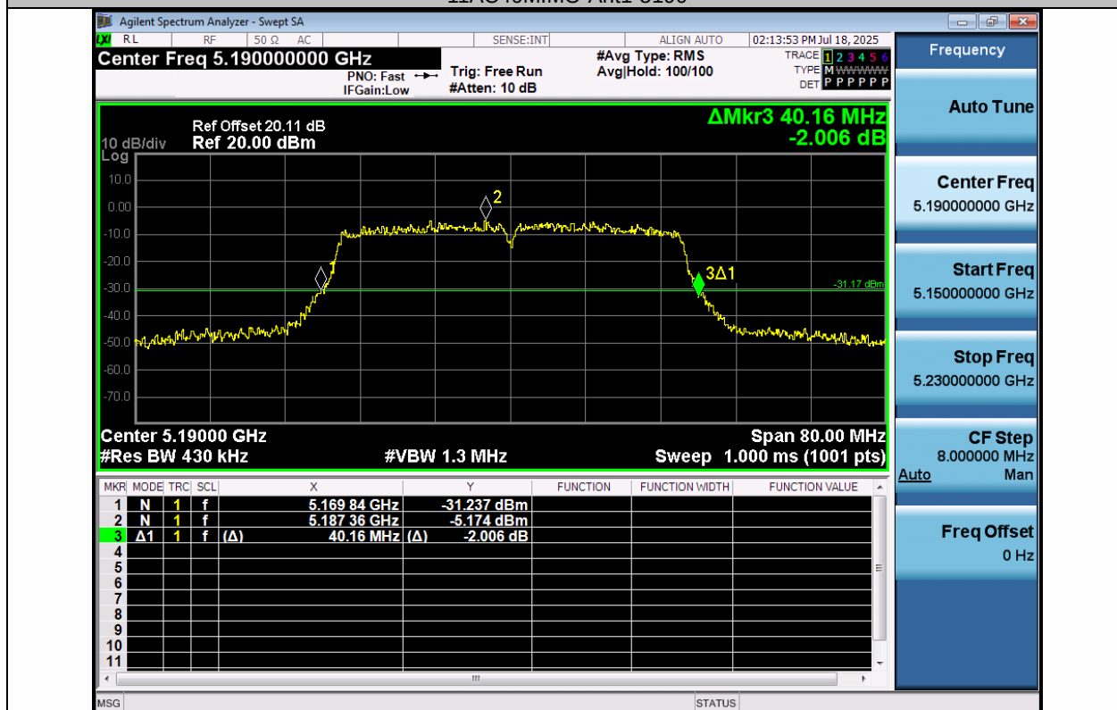
11AC40MIMO-Ant2-5190
