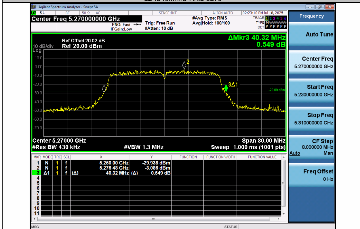
11AC40MIMO-Ant2-5270
