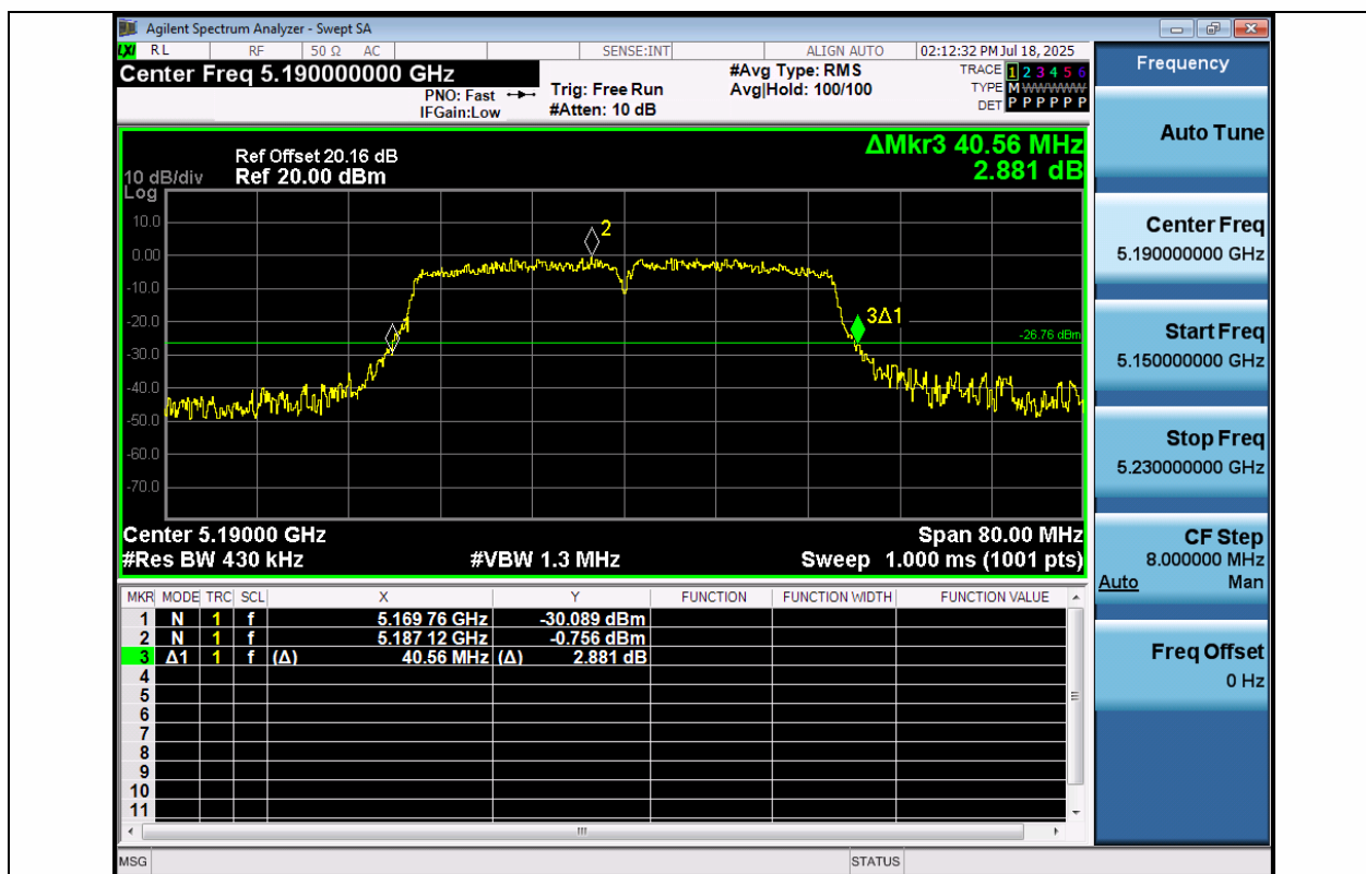
11AC40MIMO-Ant1-5190
