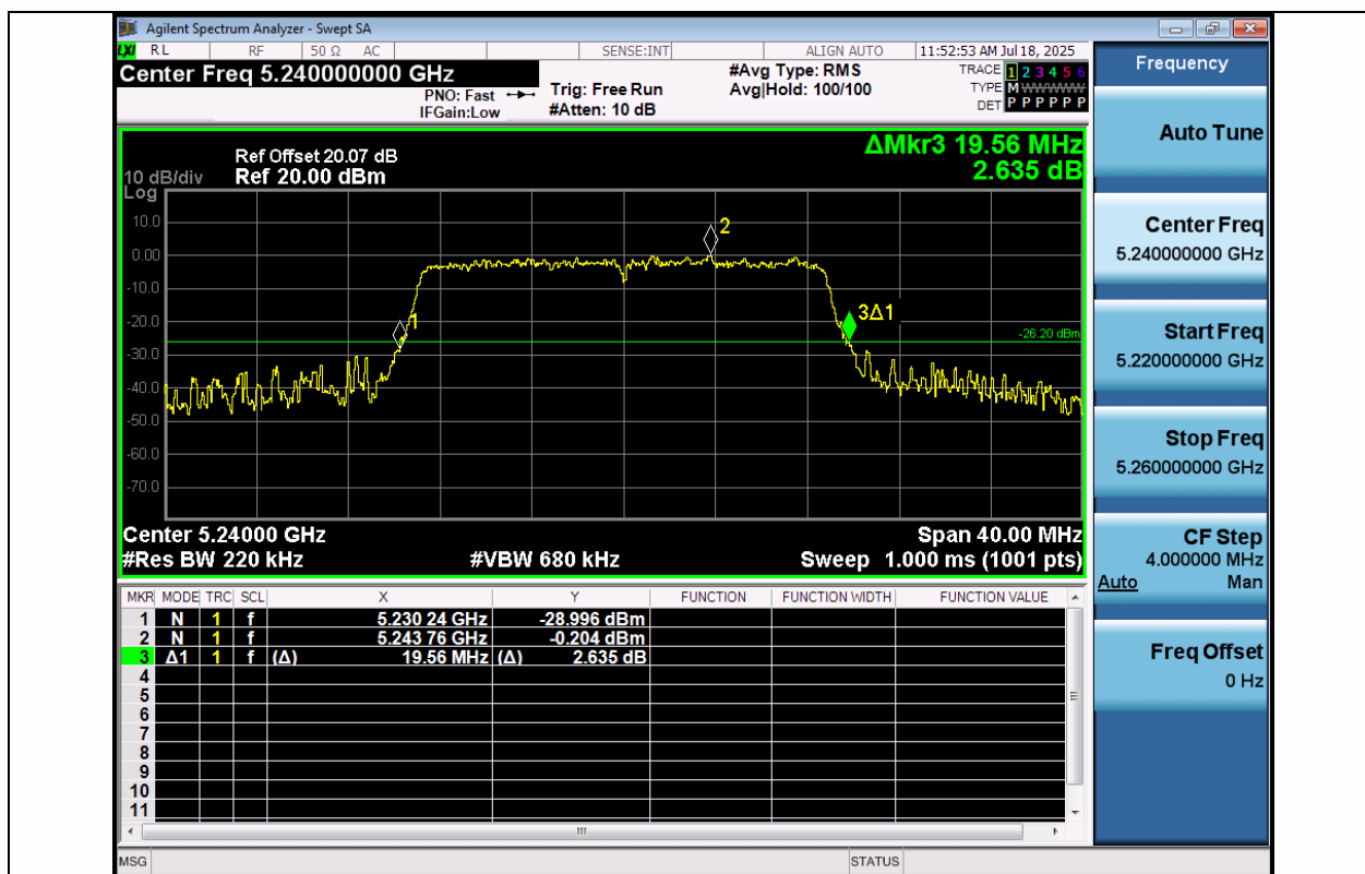
11AC20MIMO-Ant1-5240
