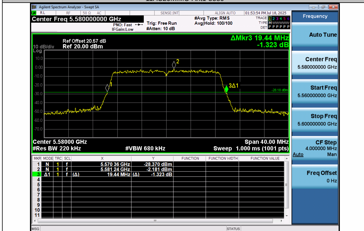
11AC20MIMO-Ant2-5580
