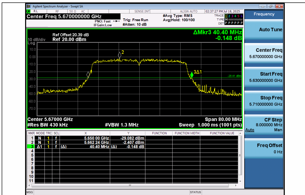
11AC40MIMO-Ant1-5670
