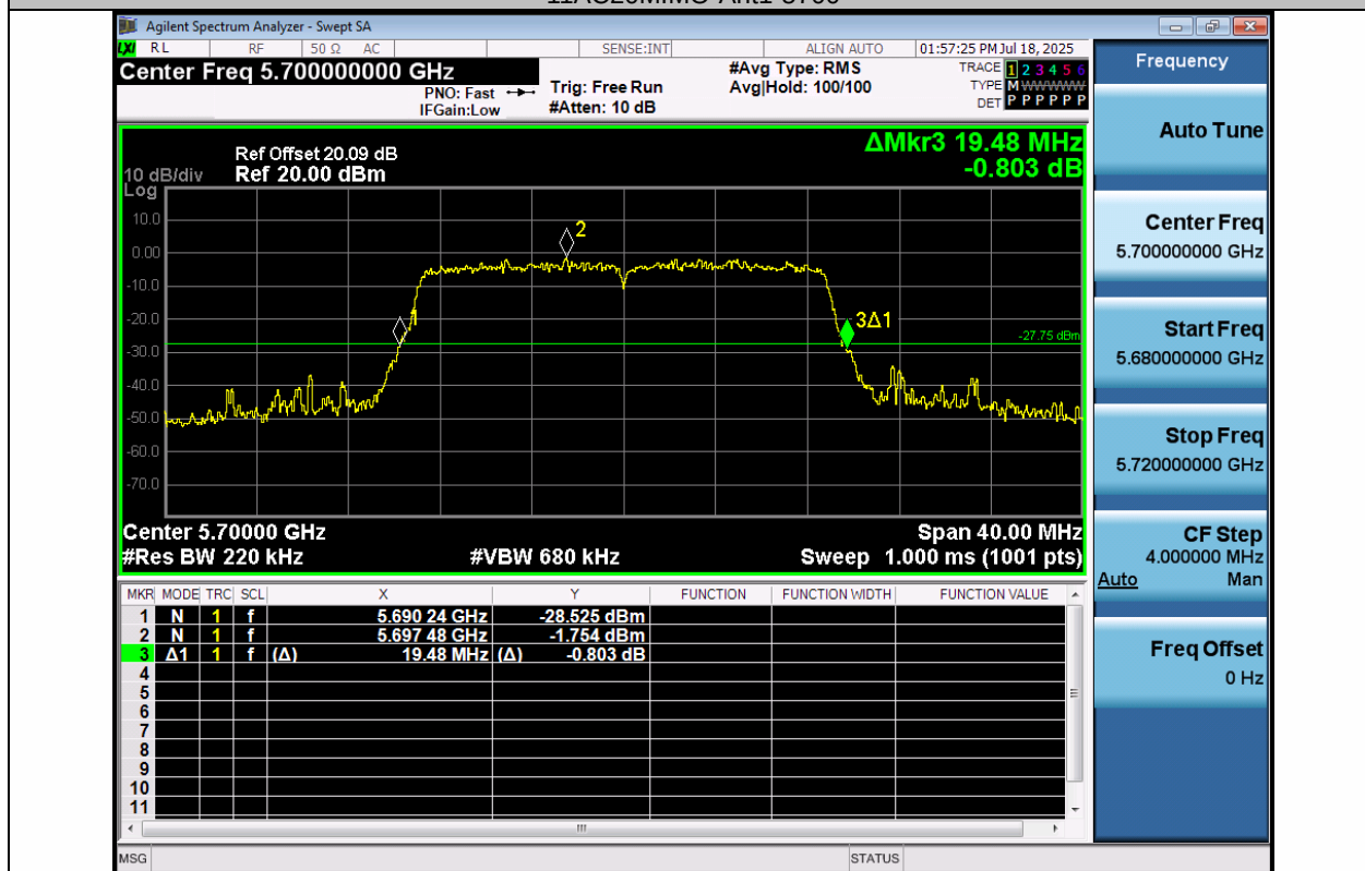
11AC20MIMO-Ant2-5700
