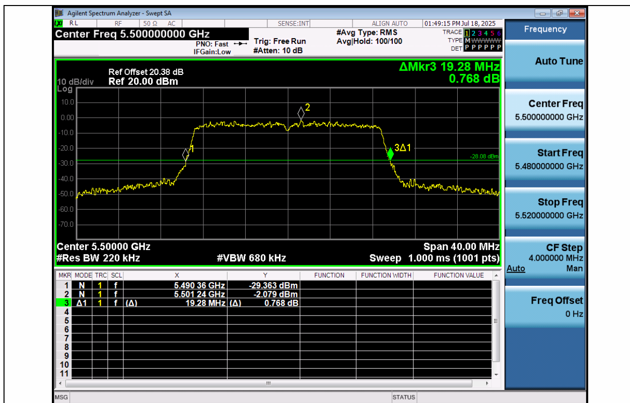
11AC20MIMO-Ant1-5500
