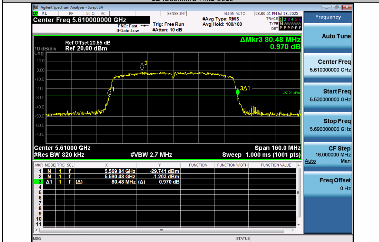
11AC80MIMO-Ant2-5610
