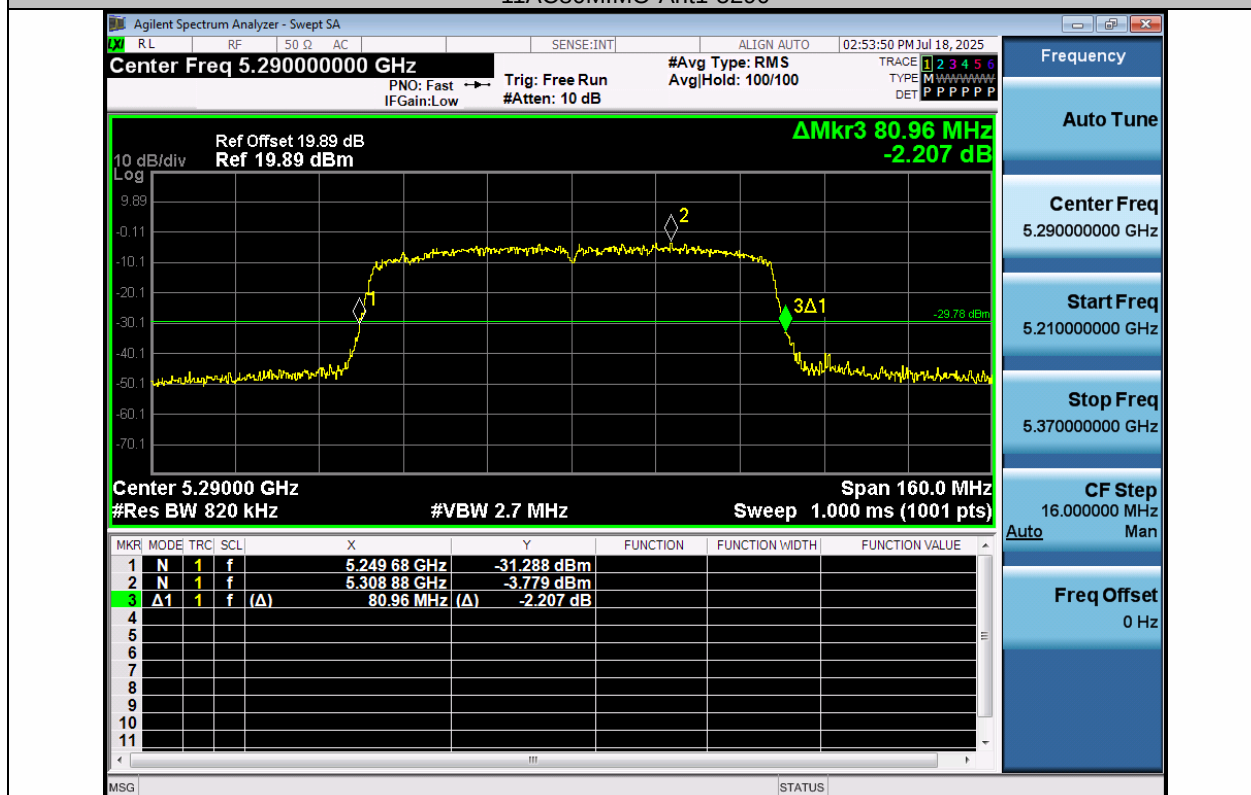
11AC80MIMO-Ant2-5290
