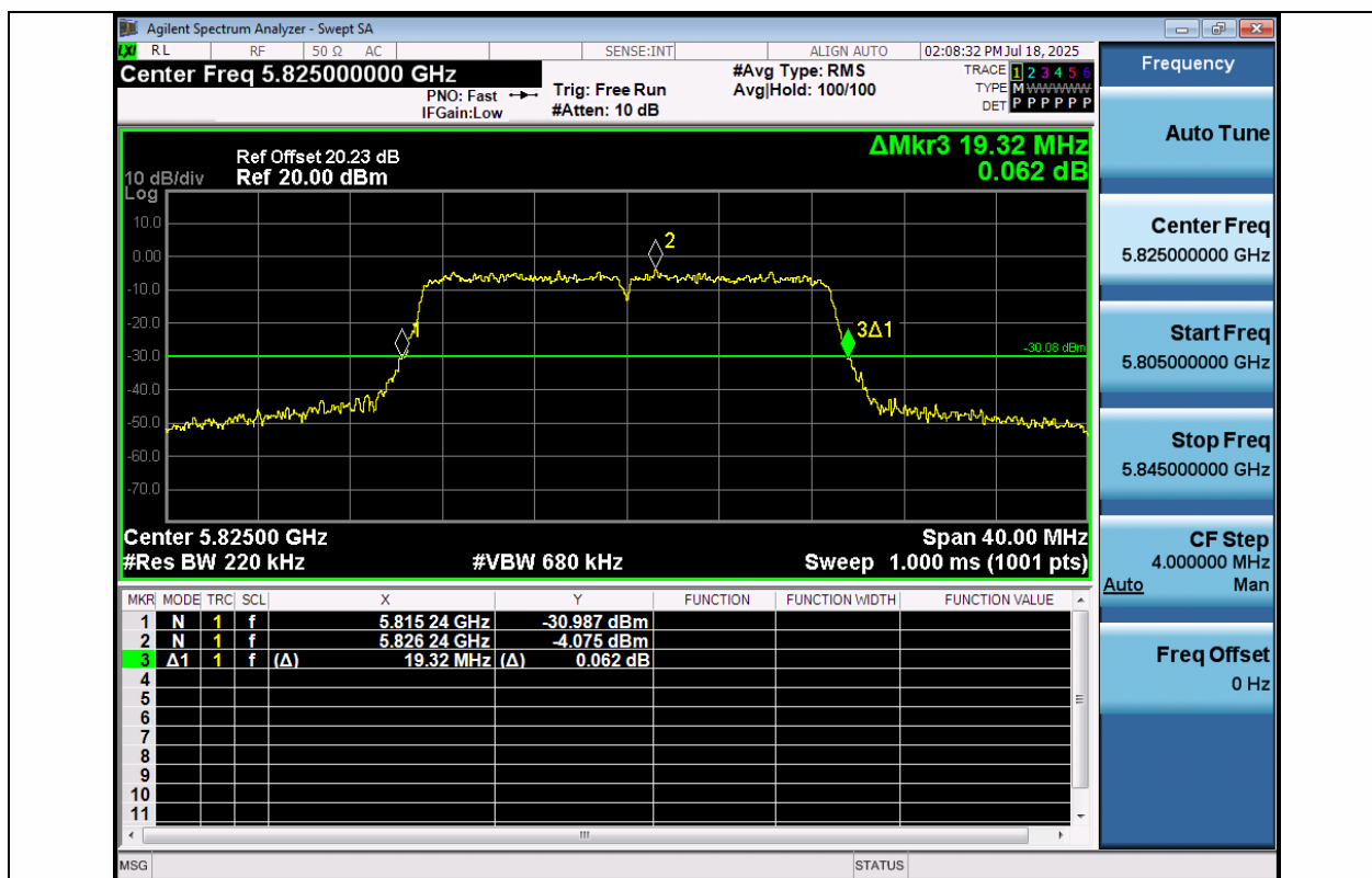
11AC20MIMO-Ant1-5825
