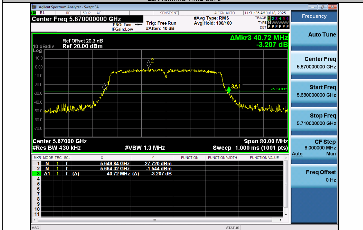
11N40MIMO-Ant2-5670
