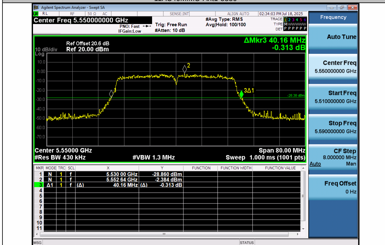
11AC40MIMO-Ant2-5550
