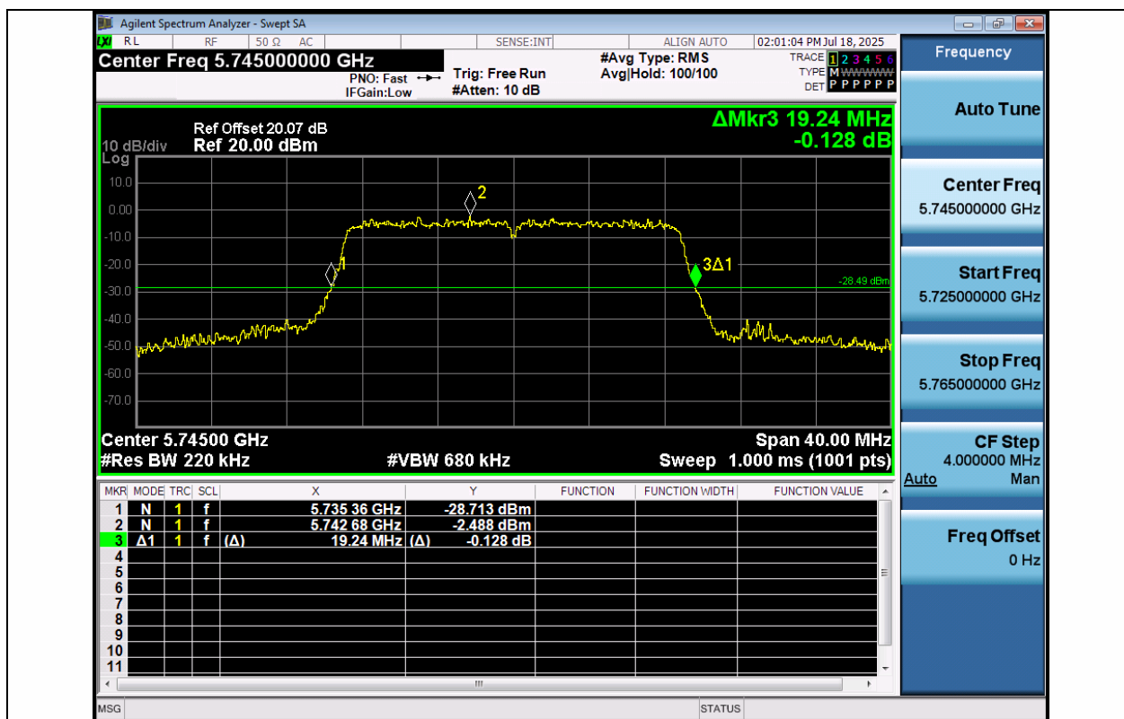
11AC20MIMO-Ant1-5745
