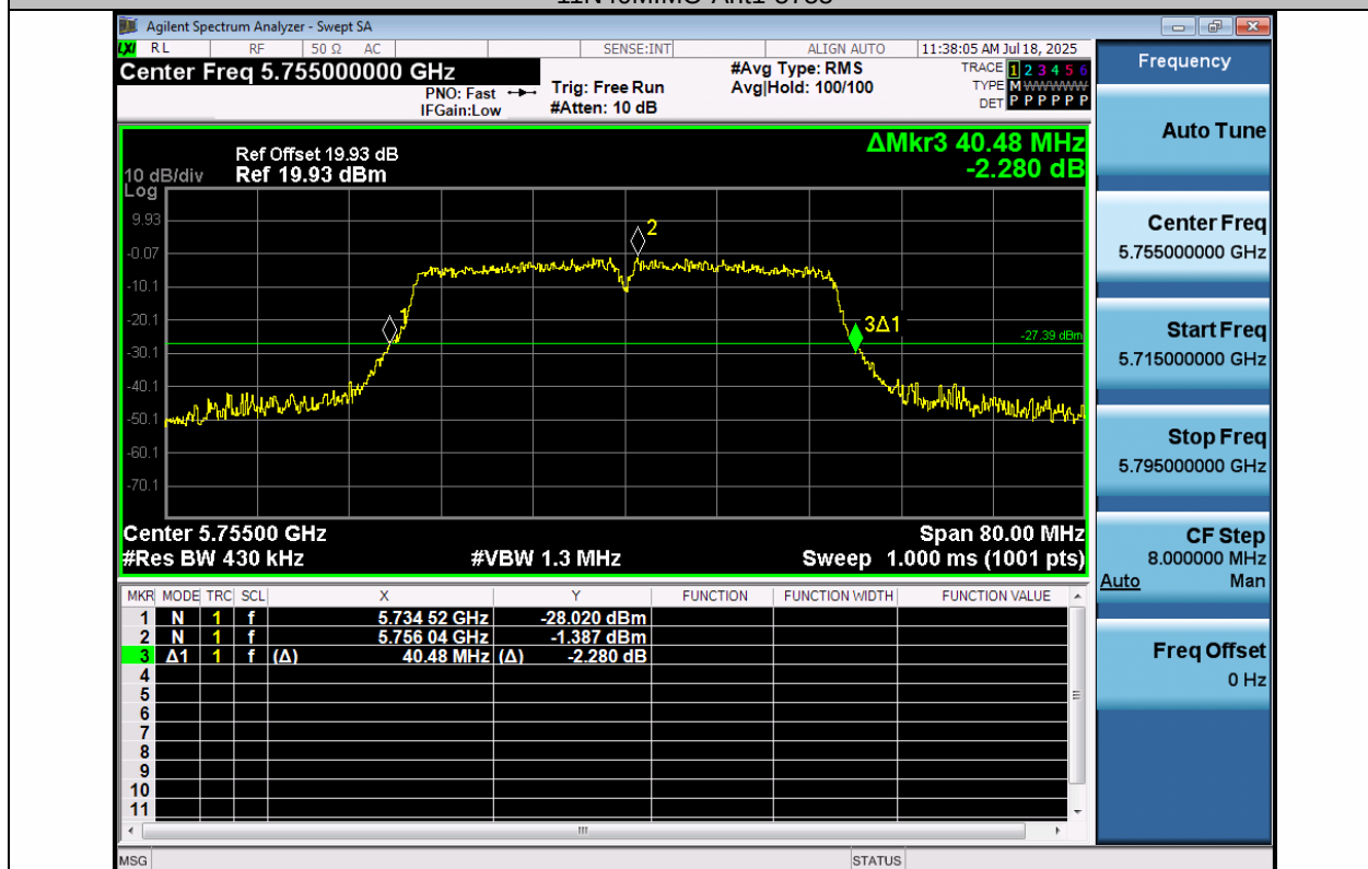
11N40MIMO-Ant2-5755
