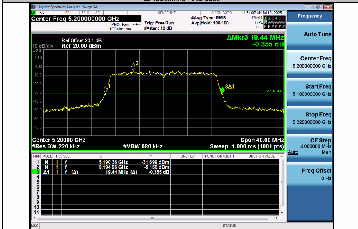
11AC20MIMO-Ant2-5200
