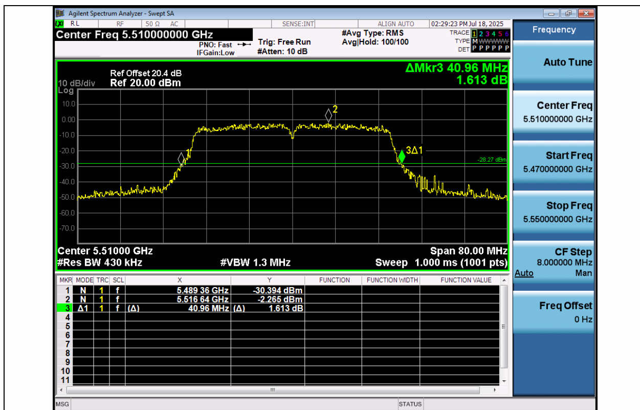
11AC40MIMO-Ant1-5510
