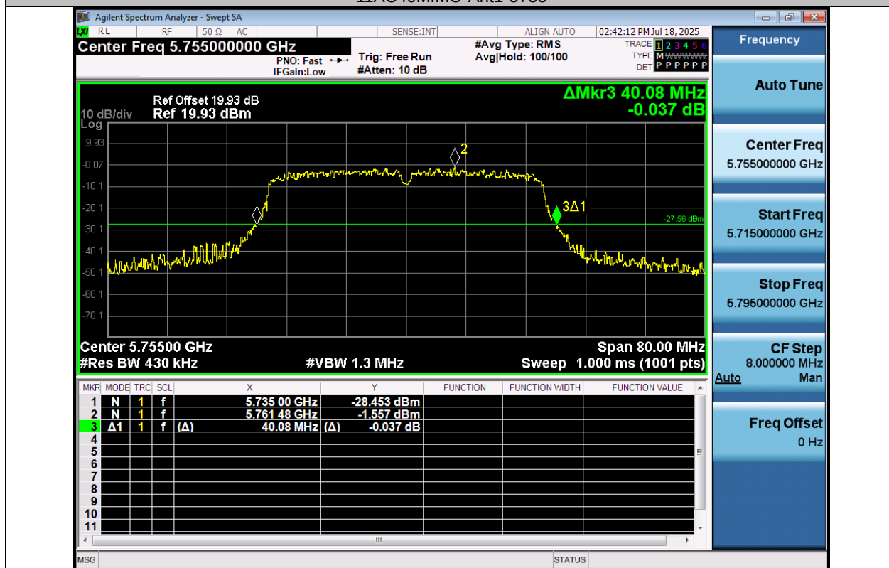
11AC40MIMO-Ant2-5755
