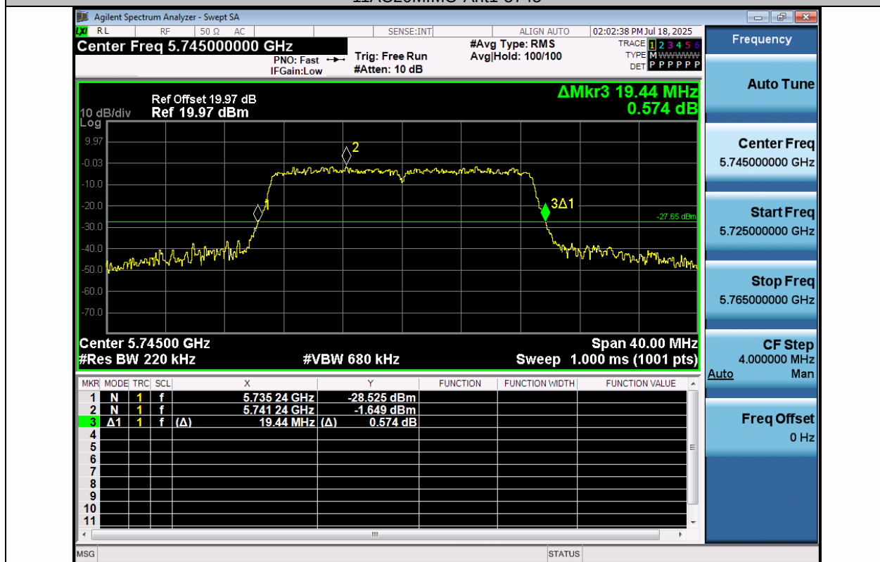
11AC20MIMO-Ant2-5745
