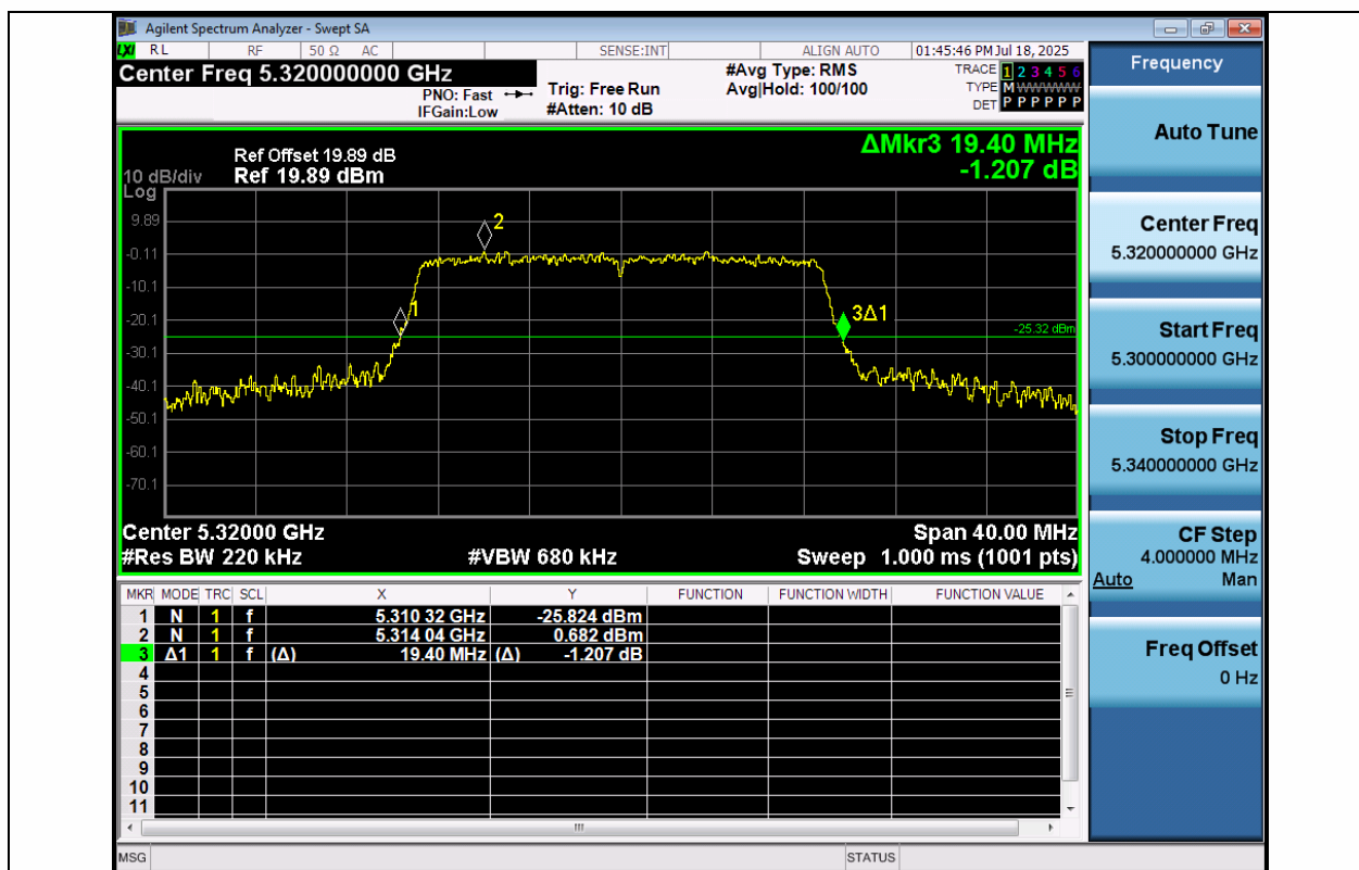
11AC20MIMO-Ant1-5320
