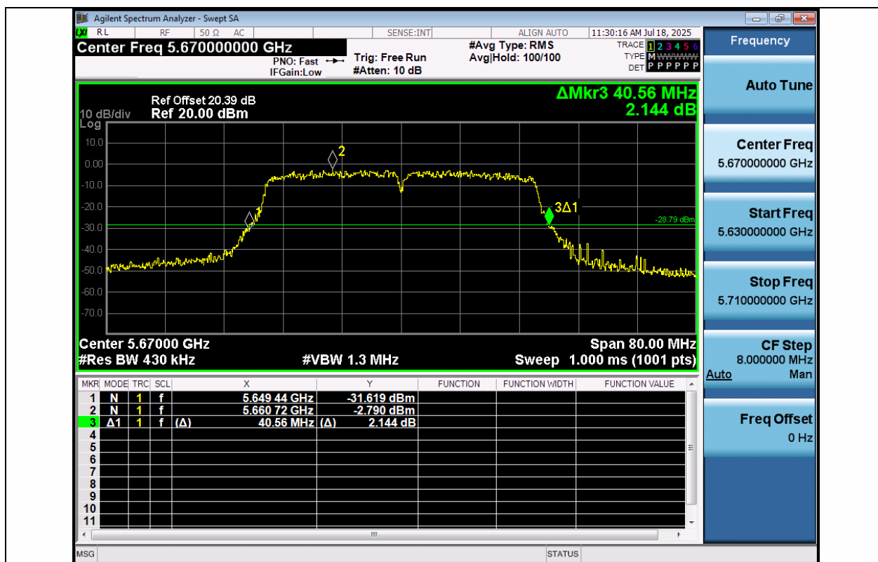
11N40MIMO-Ant1-5670
