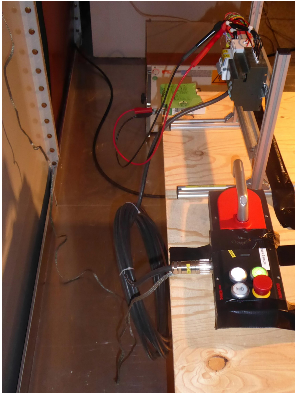
Test setup shielded room M4; Conducted emissions on supply line
