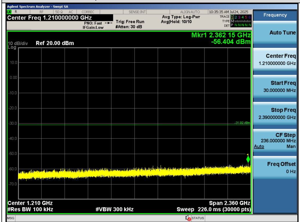
Test_Graph_GFSK_ANT1_2416_Lower Band Emissions
