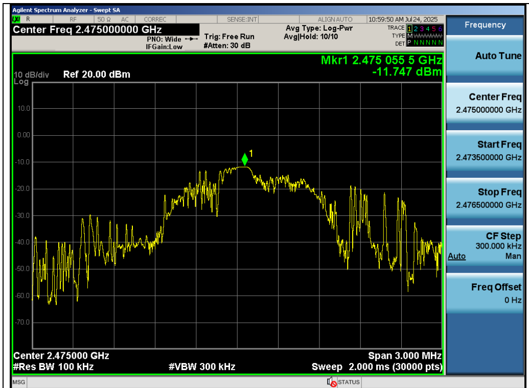
Test_Graph_GFSK_ANT1_2475_Reference Level
