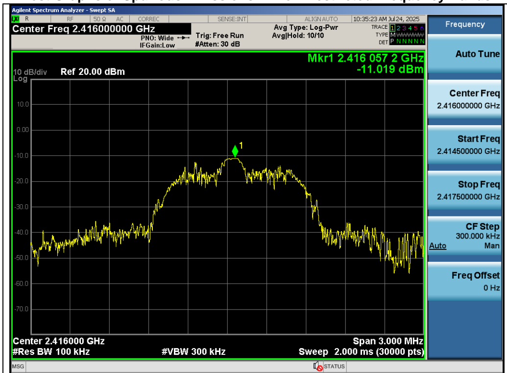
Test_Graph_GFSK_ANT1_2416_Reference Level
