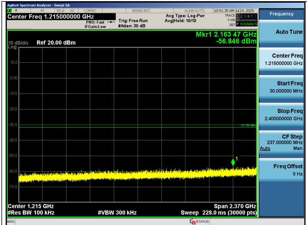
Test_Graph_GFSK_ANT1_2468_Lower Band Emissions
