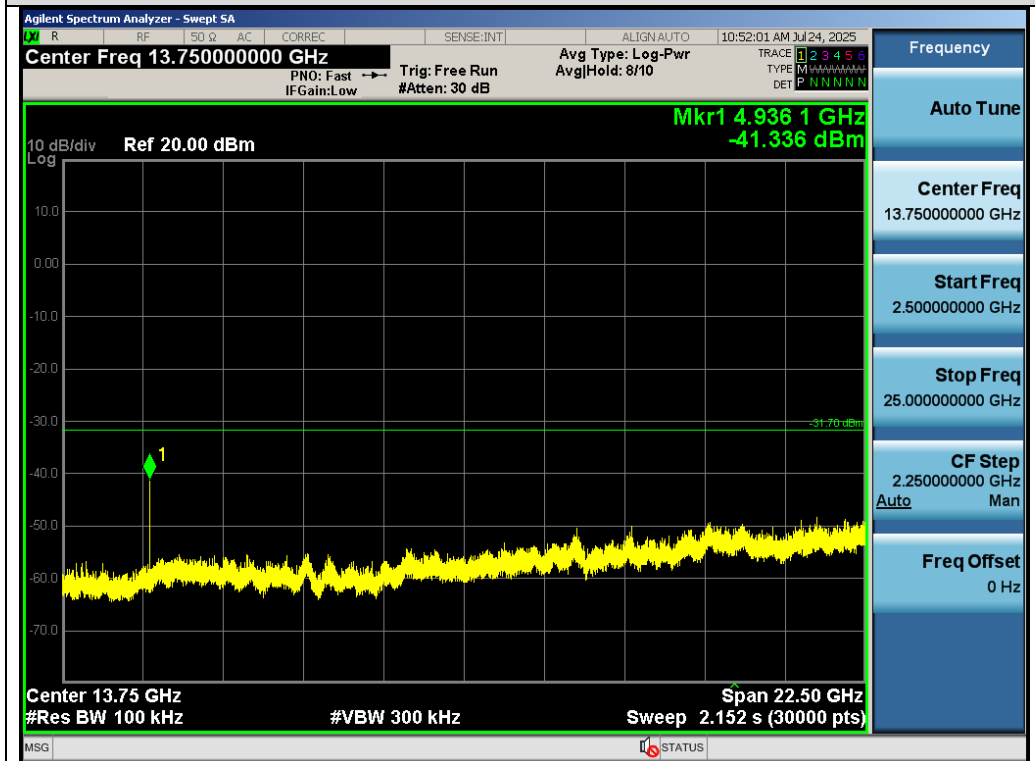
Test_Graph_GFSK_ANT1_2468_Higher Band Emissions
