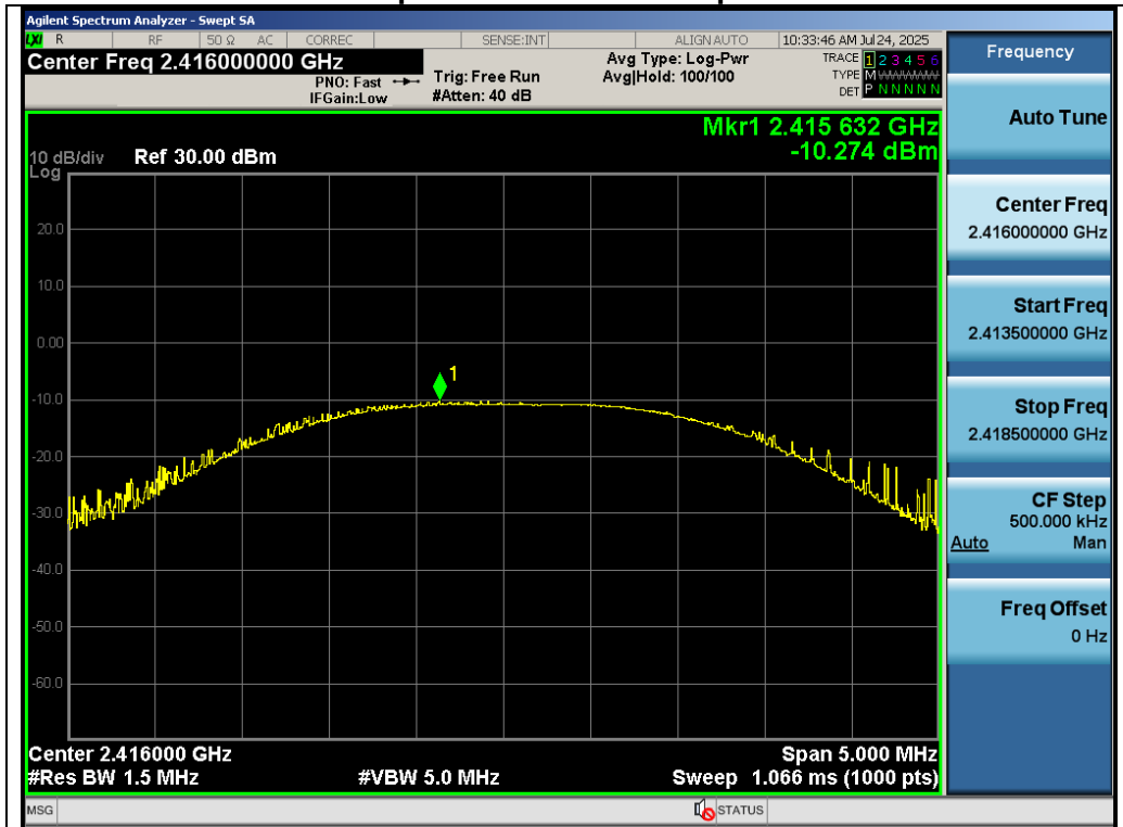
Test_Graph_GFSK_ANT1_2416_Peak Power
