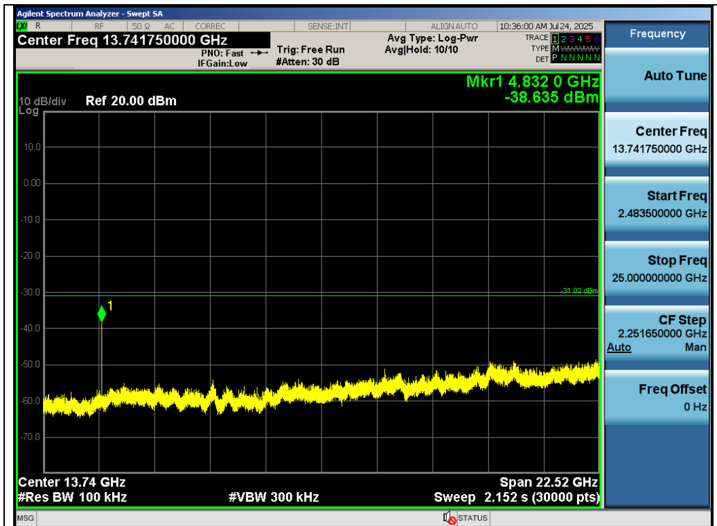
Test_Graph_GFSK_ANT1_2416_Higher Band Emissions
