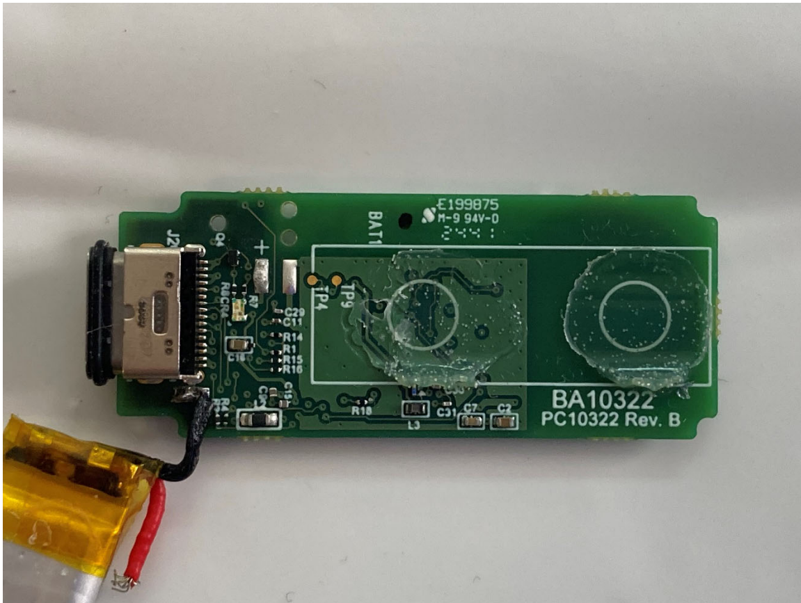
Figure 2. Top with batter pack removed
