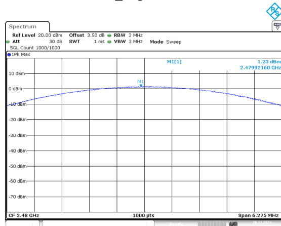
3DH1_High 1.23dBm
