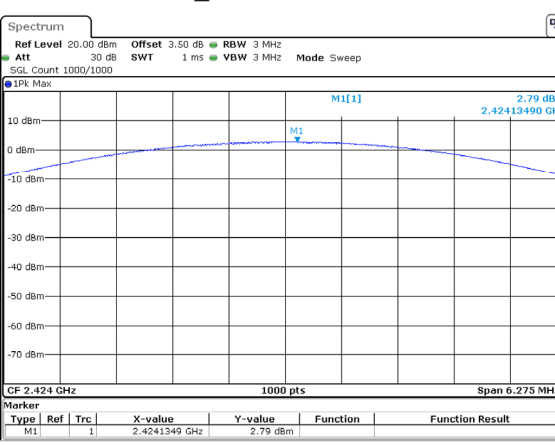
2DH1_Additional 2.79dBm
