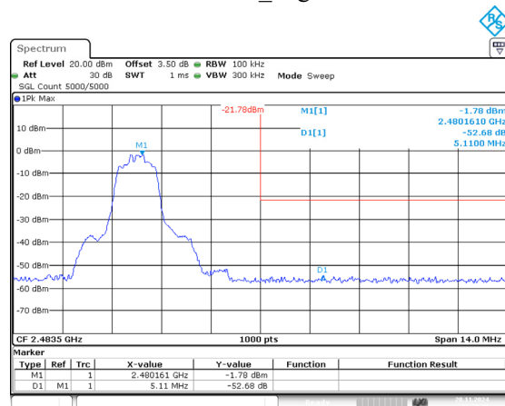
2DH1_High
