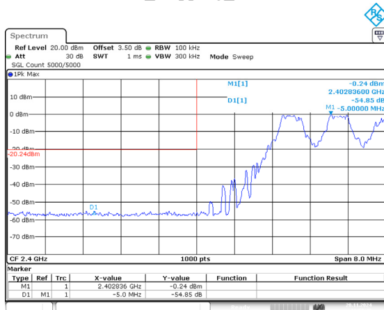
DH1_Hopping_Lower
