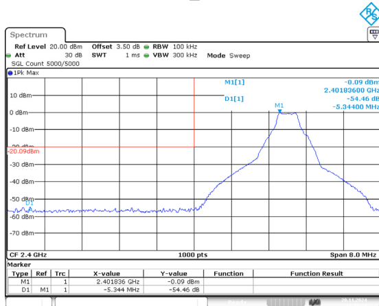
DH1_Low
