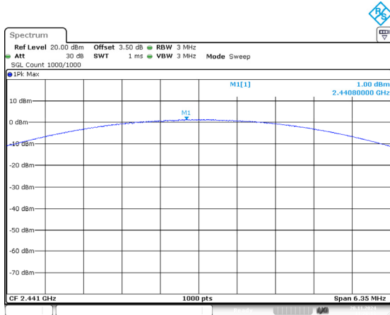
2DH1_Middle 1.00dBm
