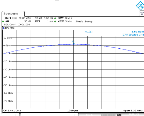
3DH1_Middle 1.63dBm
