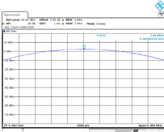
3DH1_Low 2.68dBm
