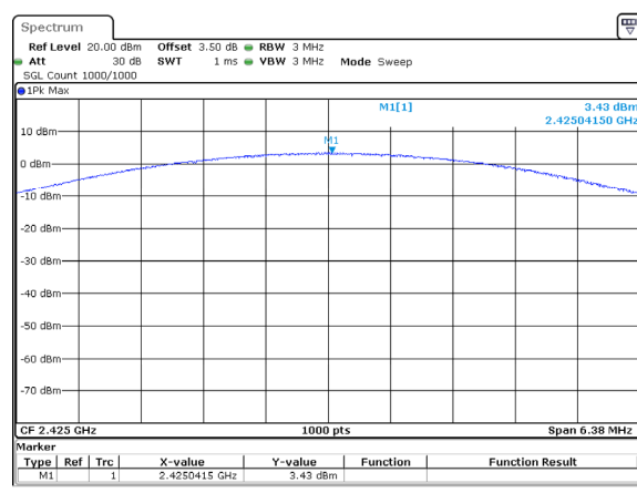
3DH1_Additional 3.43dBm
