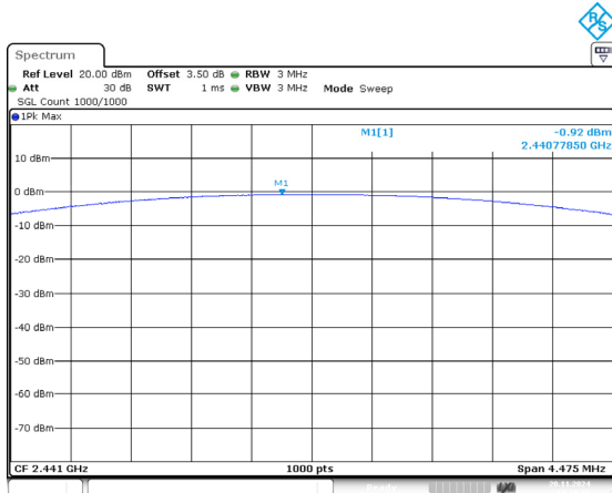
DH1_Middle -0.92dBm
