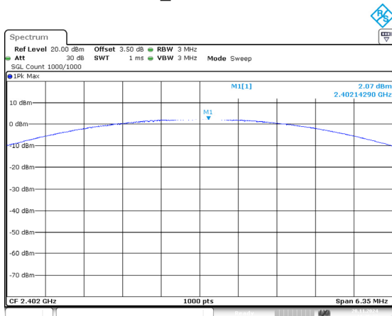
2DH1_Low 2.07dBm
