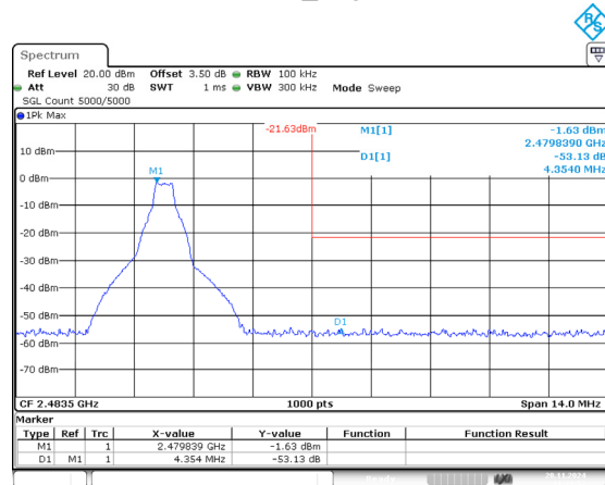
DH1_High
