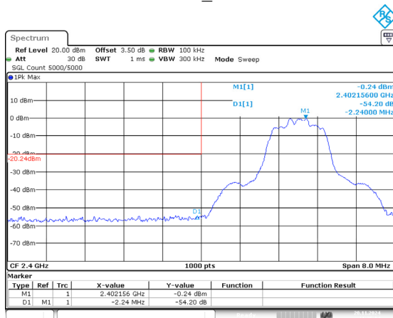
2DH1_Low
